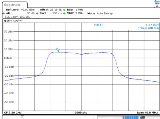
a_5260_Ant B
