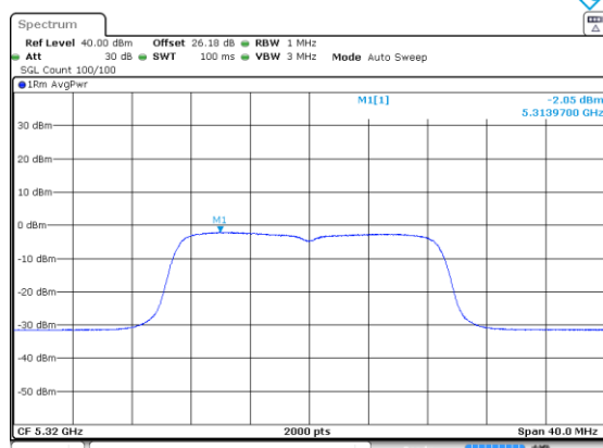
n/ac20_5320_Ant B
