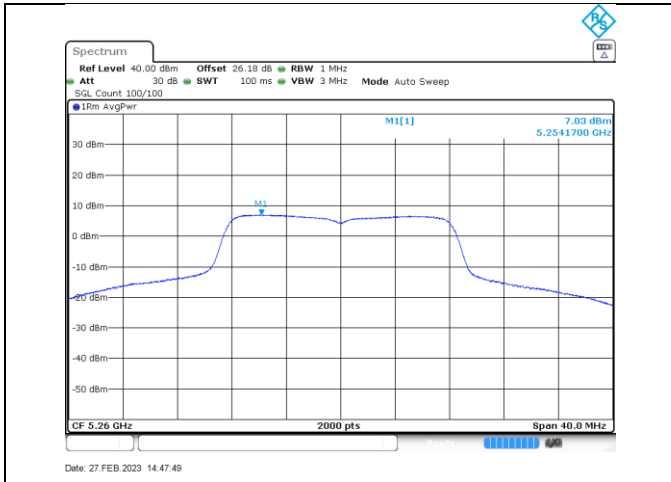
a_5260_Ant A
