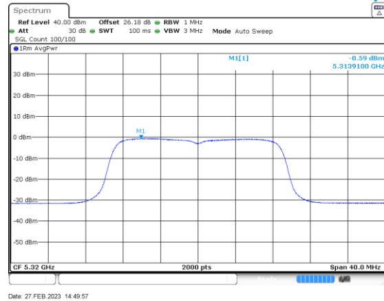
n/ac20_5320_Ant A
