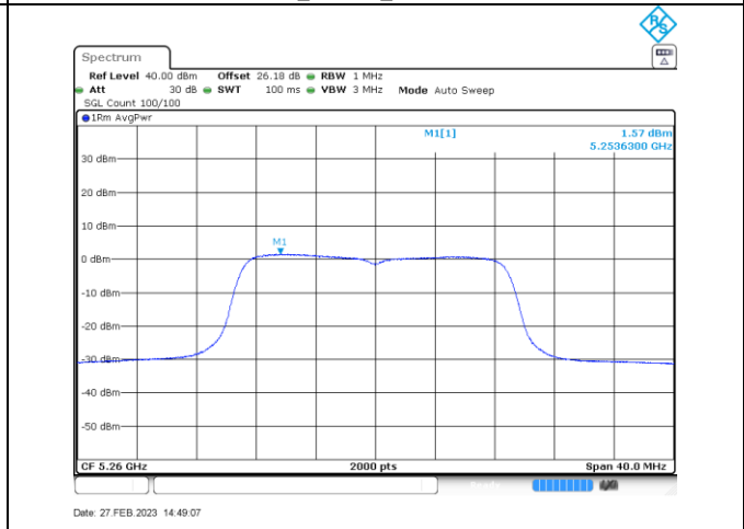
n/ac20_5260_Ant A
