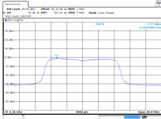
n/ac20_5260_Ant B
