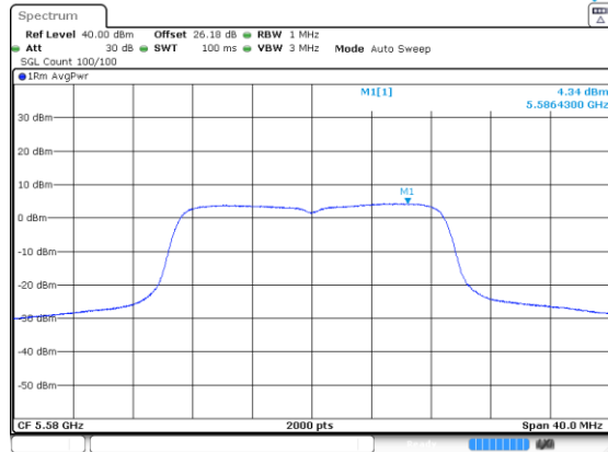
n/ac20_5580_Ant B
