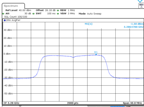
n/ac20_5280_Ant B
