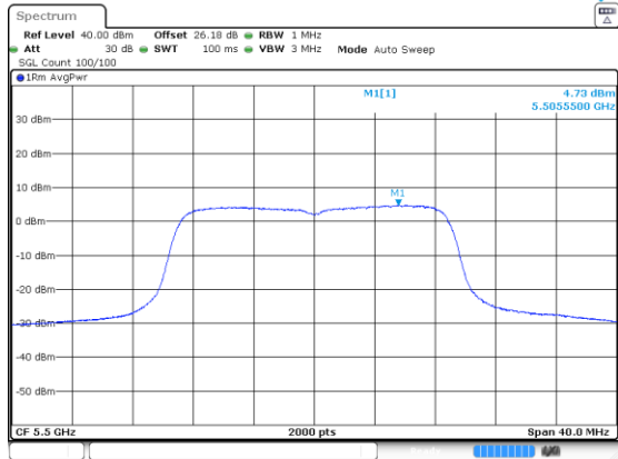
n/ac20_5500_Ant B
