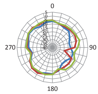
2D YOZ
