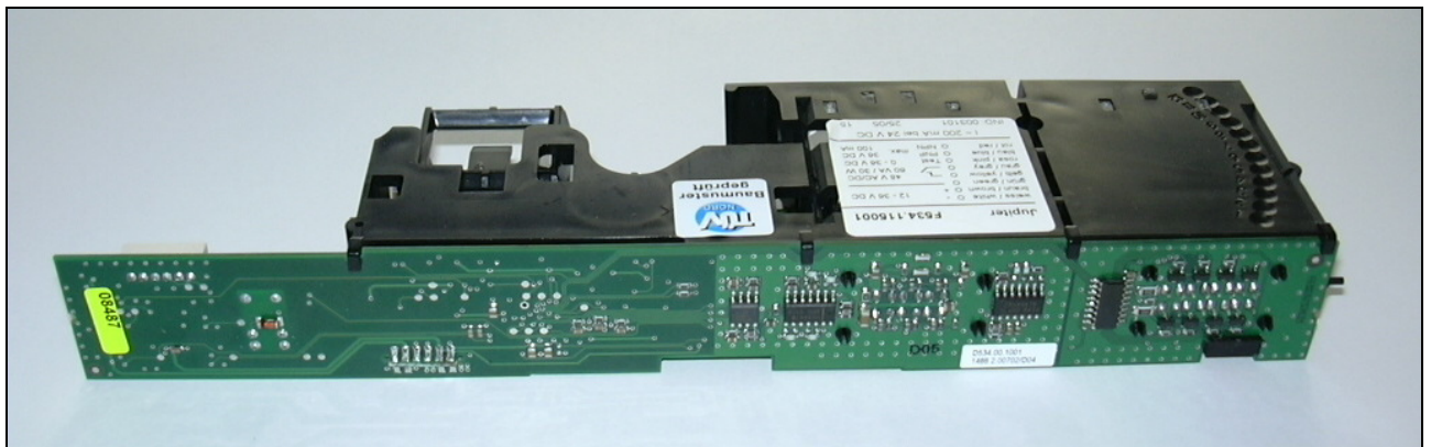
Photo 3: Overall appearance Back View
