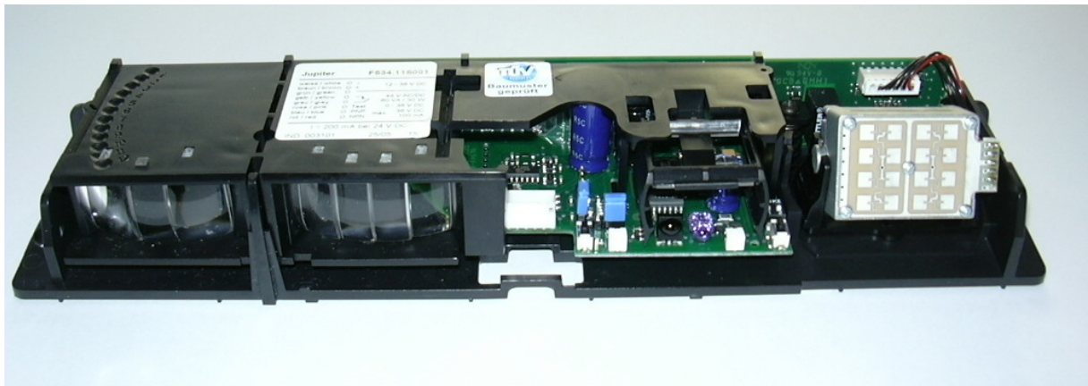
Photo 3: Component placement on the chassis
