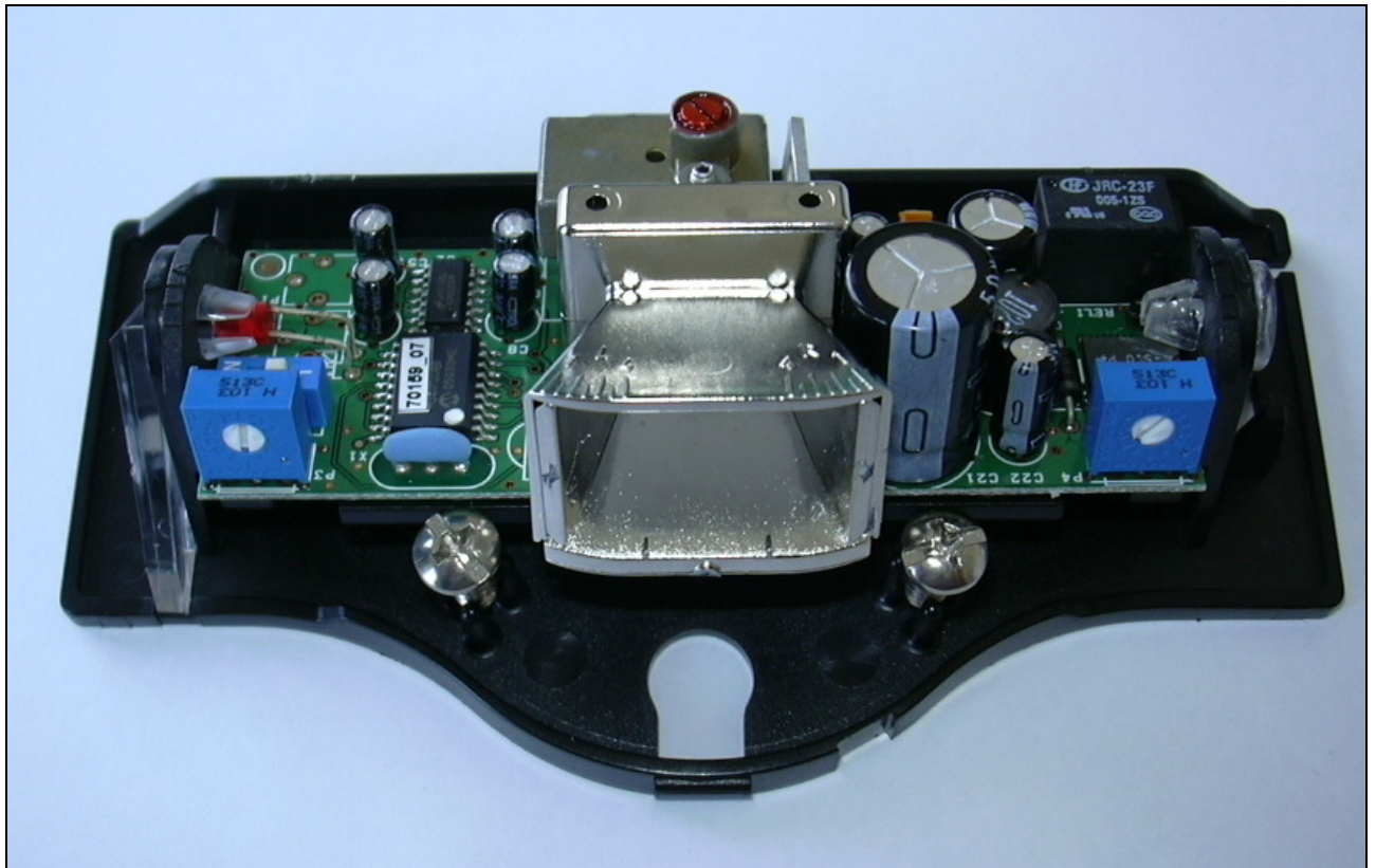
Photo 3: Component placement on the chassis
