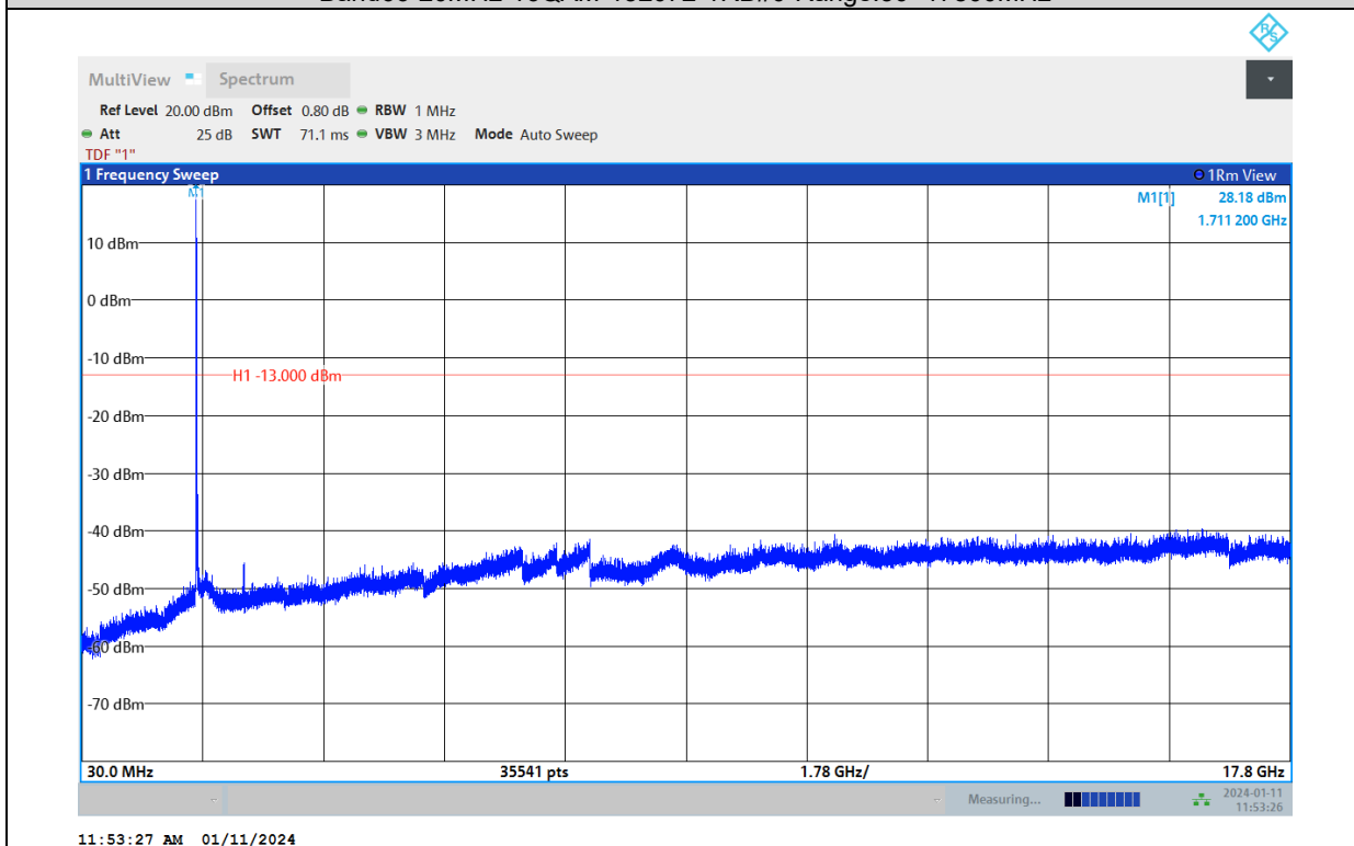
Band66-20MHz-16QAM-132322-1RB#0-Range:30~17800MHz
