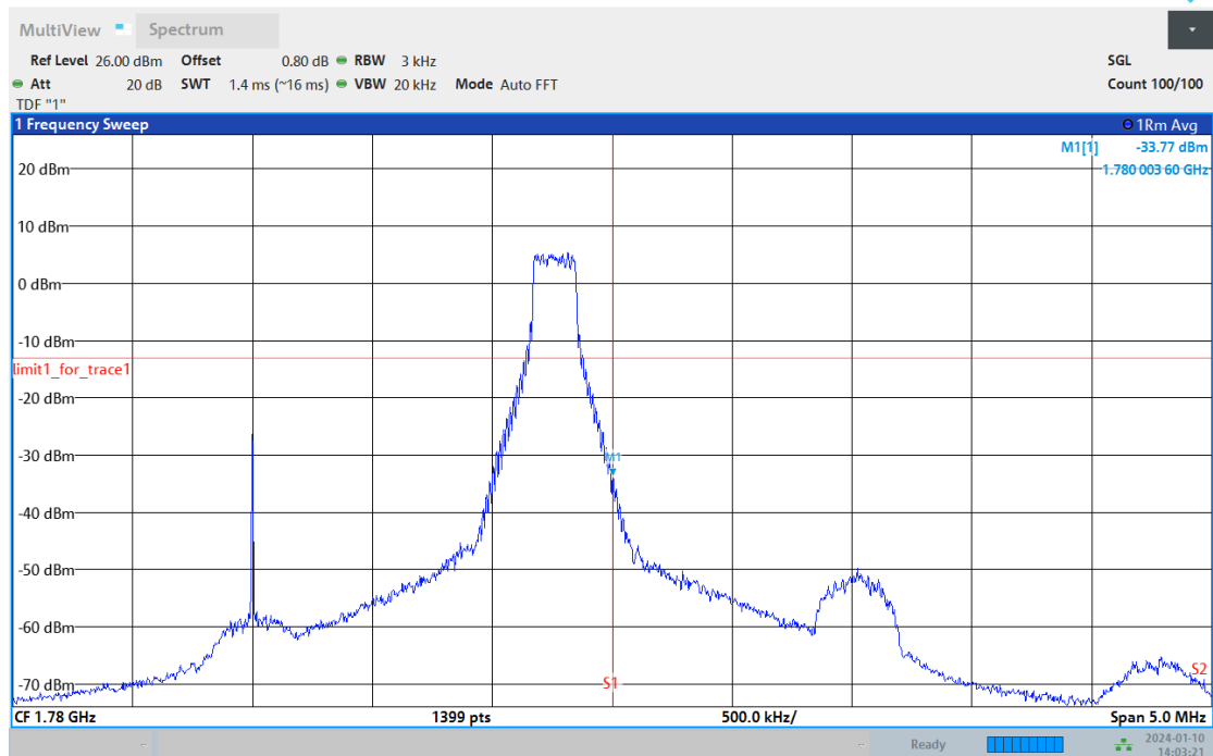
Band66-3MHz-64QAM-132657-15RB#0
