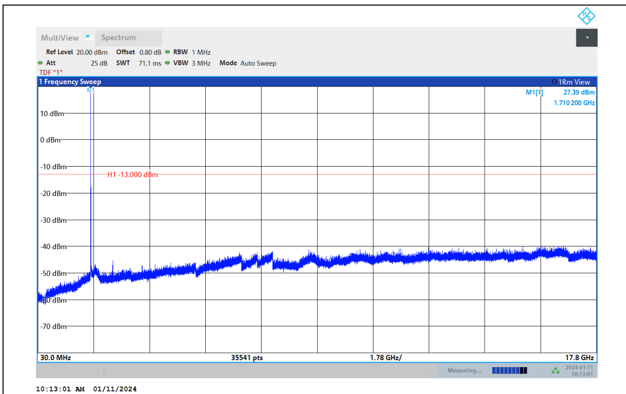
Band66-3MHz-16QAM-132322-1RB#0-Range:30~17800MHz
