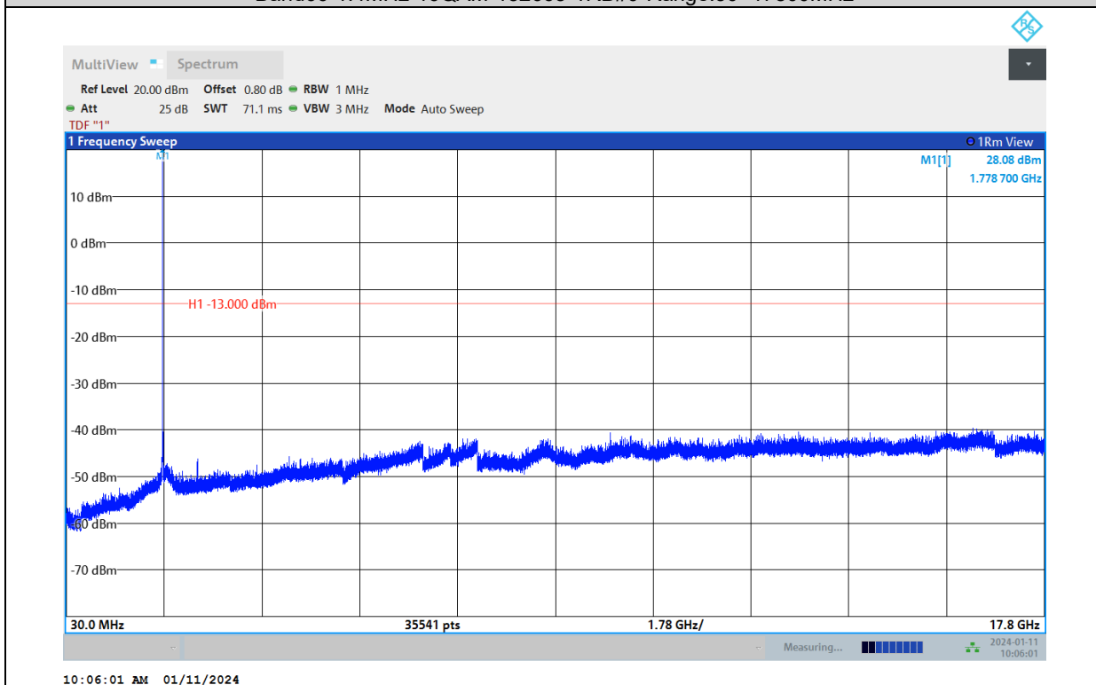
Band66-1.4MHz-64QAM-131979-1RB#0-Range:30~17800MHz
