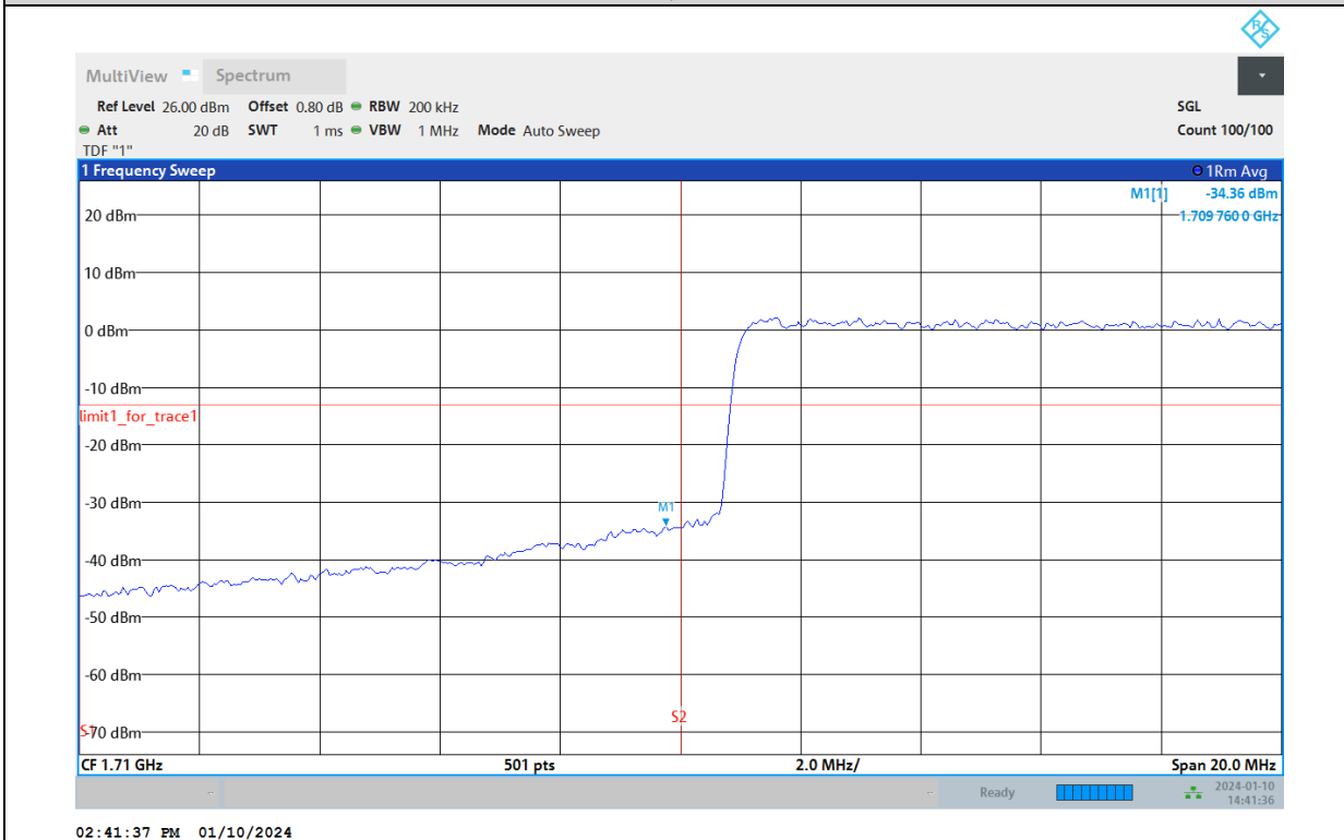
Band66-20MHz-16QAM-132572-1RB#99
