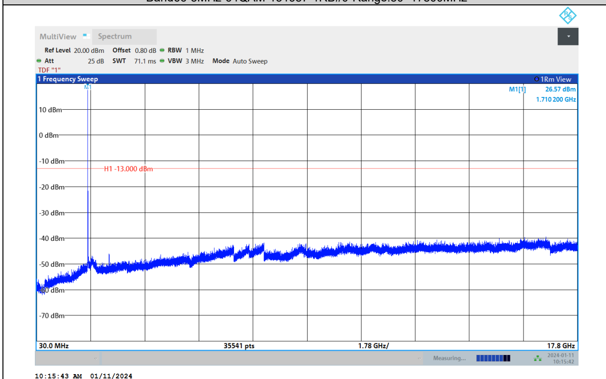
Band66-3MHz-64QAM-132322-1RB#0-Range:30~17800MHz
