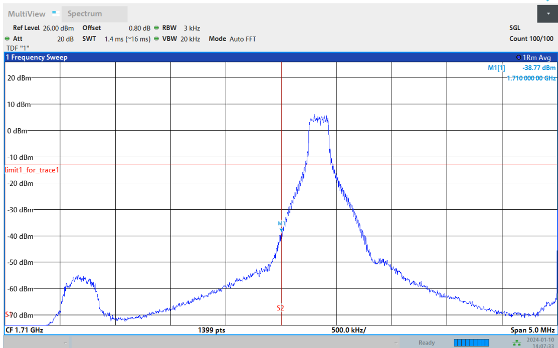
Band66-5MHz-16QAM-131997-25RB#0
