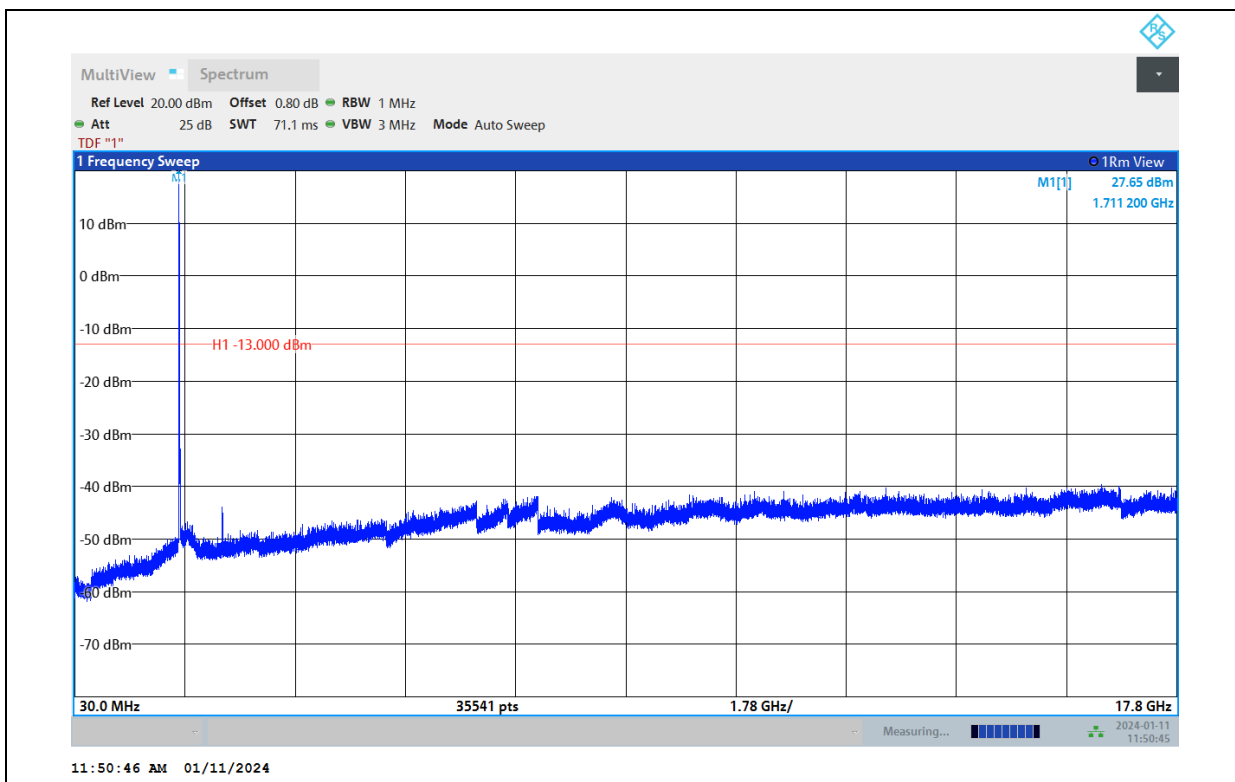
Band66-20MHz-QPSK-132322-1RB#0-Range:30~17800MHz
