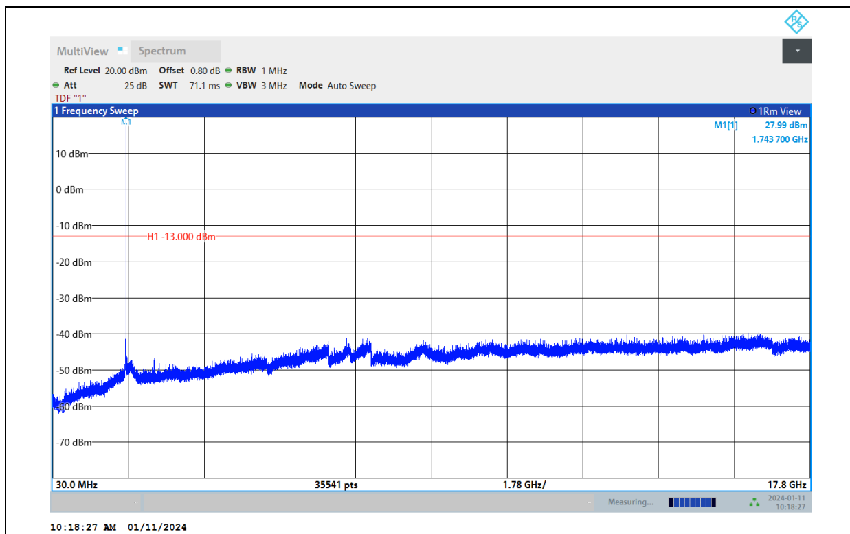
Band66-3MHz-QPSK-132657-1RB#0-Range:30~17800MHz
