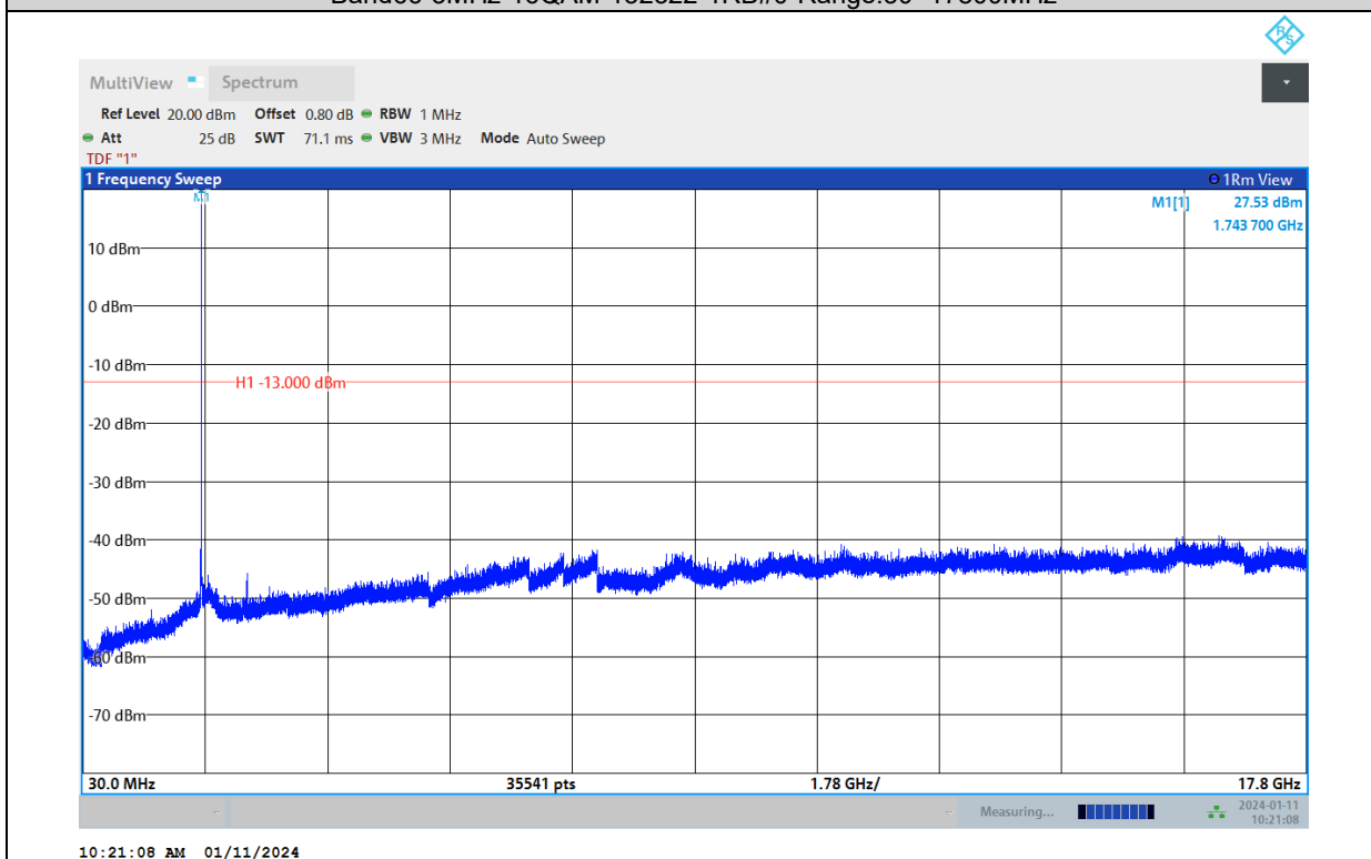
Band66-3MHz-16QAM-132657-1RB#0-Range:30~17800MHz
