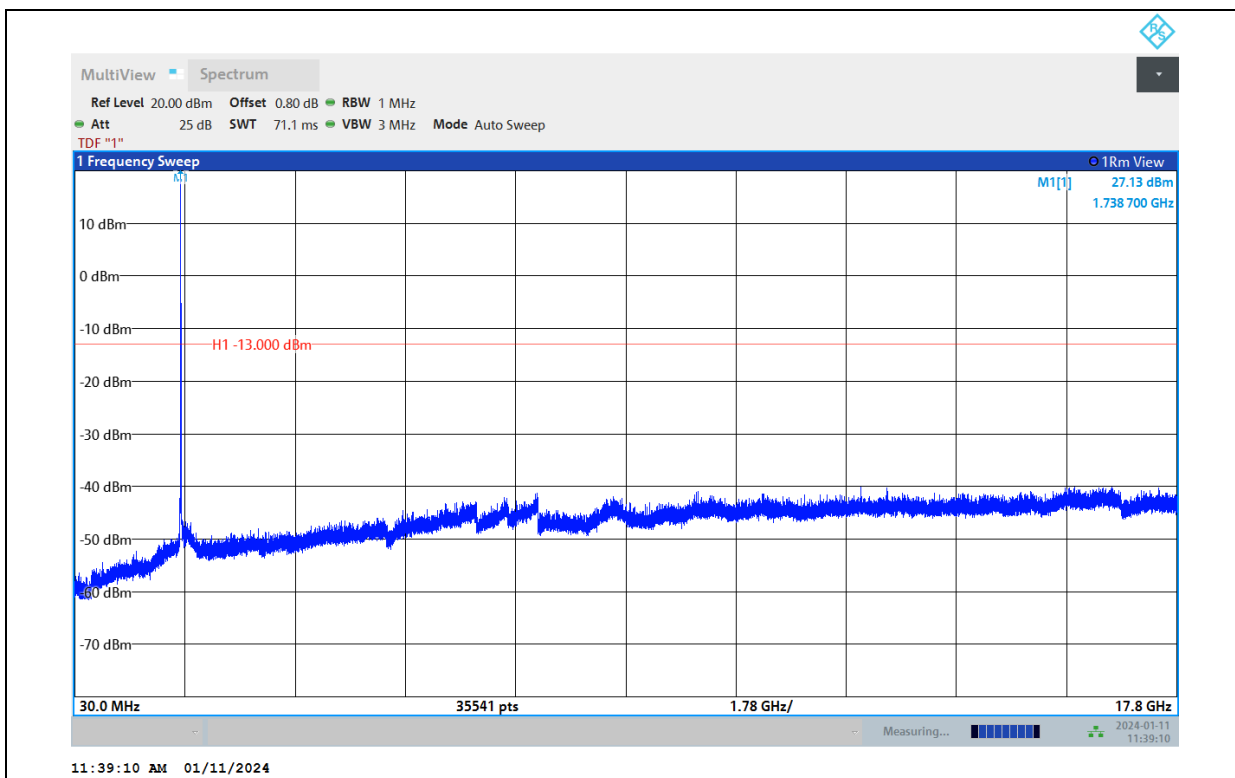
Band66-15MHz-64QAM-132597-1RB#0-Range:30~17800MHz
