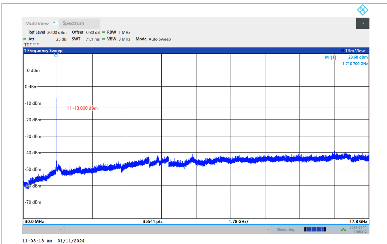
Band66-10MHz-16QAM-132322-1RB#0-Range:30~17800MHz
