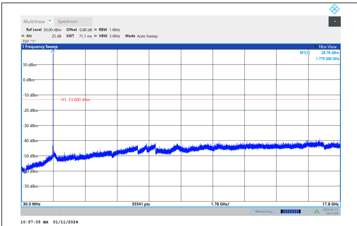
Band66-10MHz-QPSK-132022-1RB#0-Range:30~17800MHz
