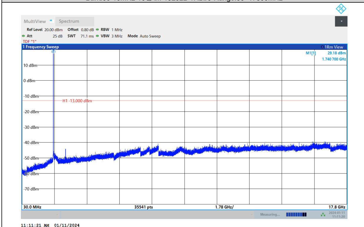
Band66-10MHz-16QAM-132622-1RB#0-Range:30~17800MHz
