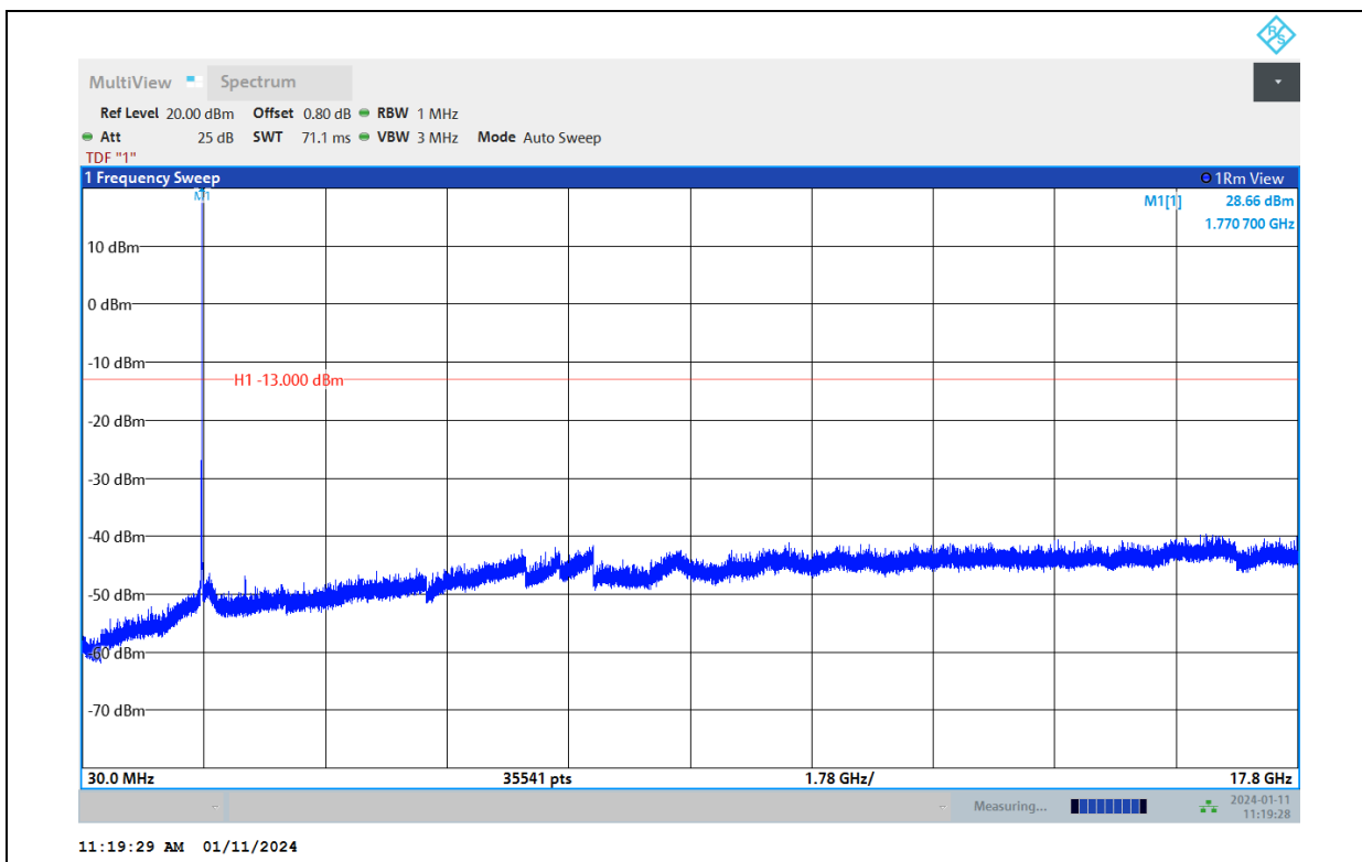
Band66-10MHz-64QAM-132022-1RB#0-Range:30~17800MHz
