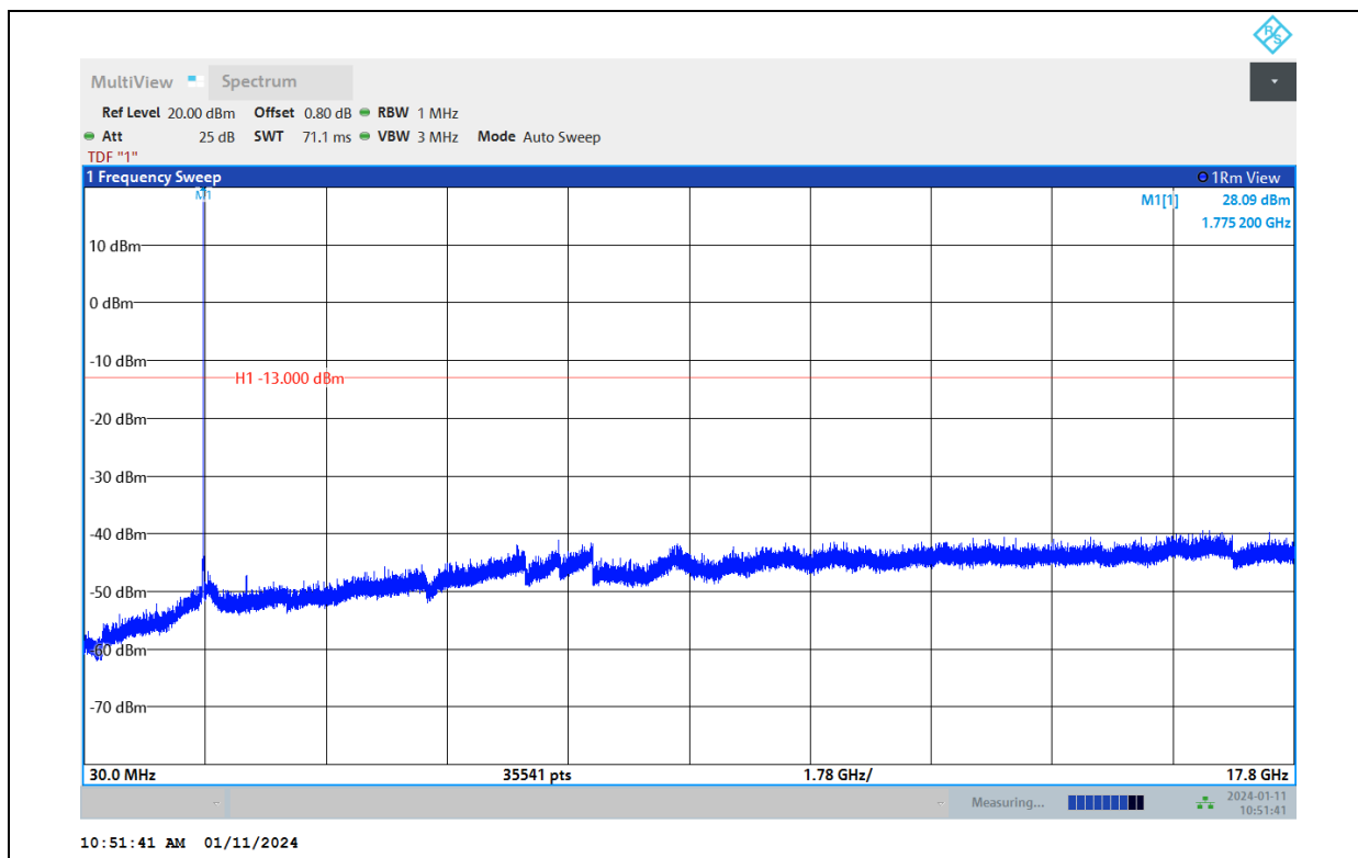
Band66-5MHz-16QAM-131997-1RB#0-Range:30~17800MHz
