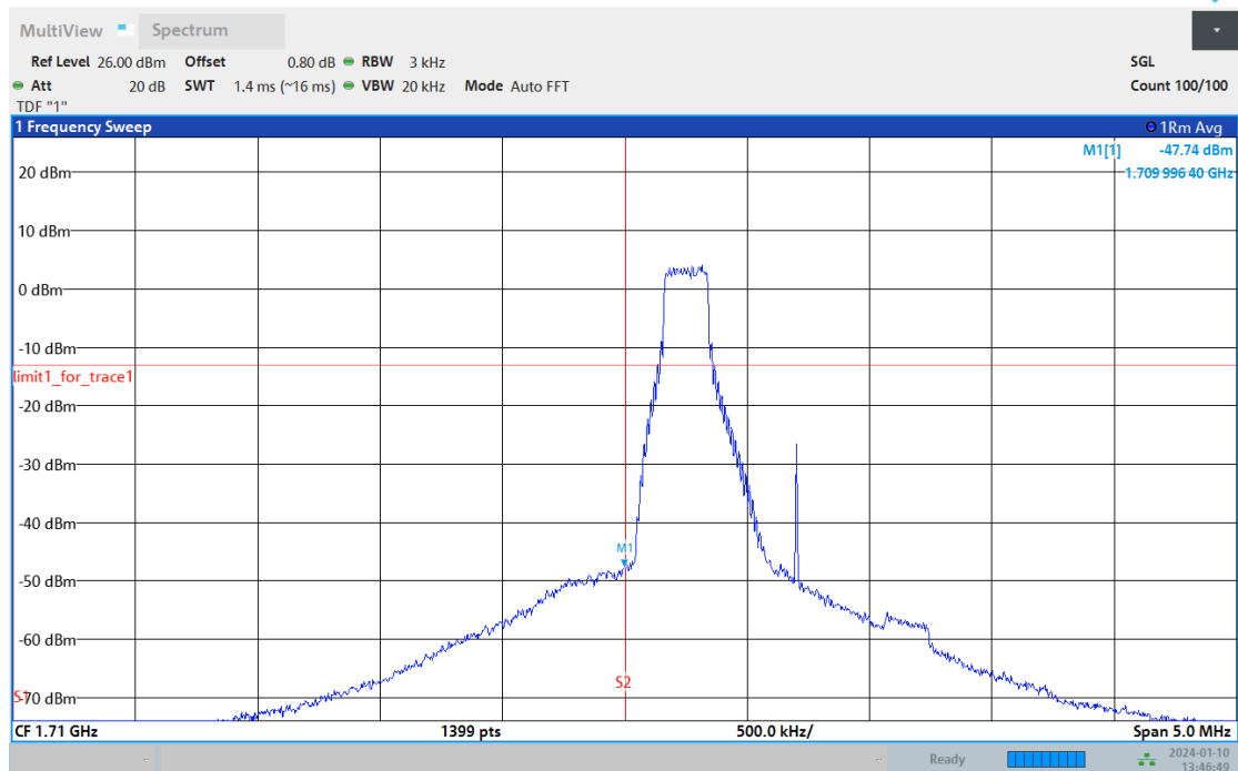
Band66-1.4MHz-64QAM-131979-6RB#0
