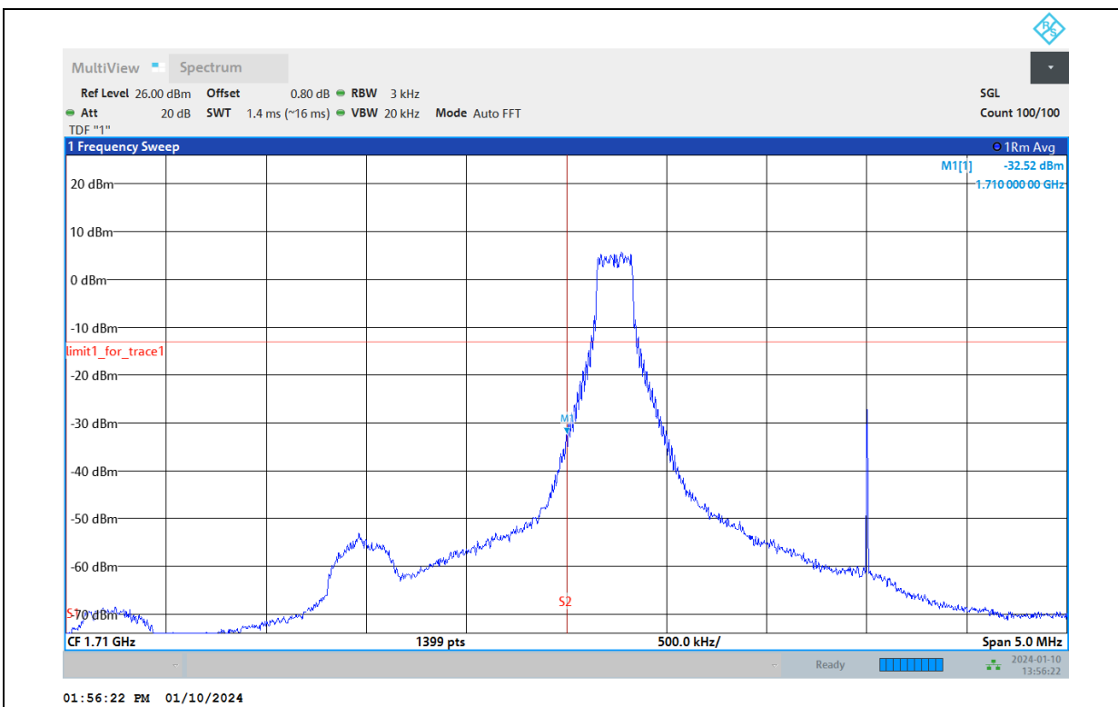
Band66-3MHz-16QAM-131987-15RB#0
