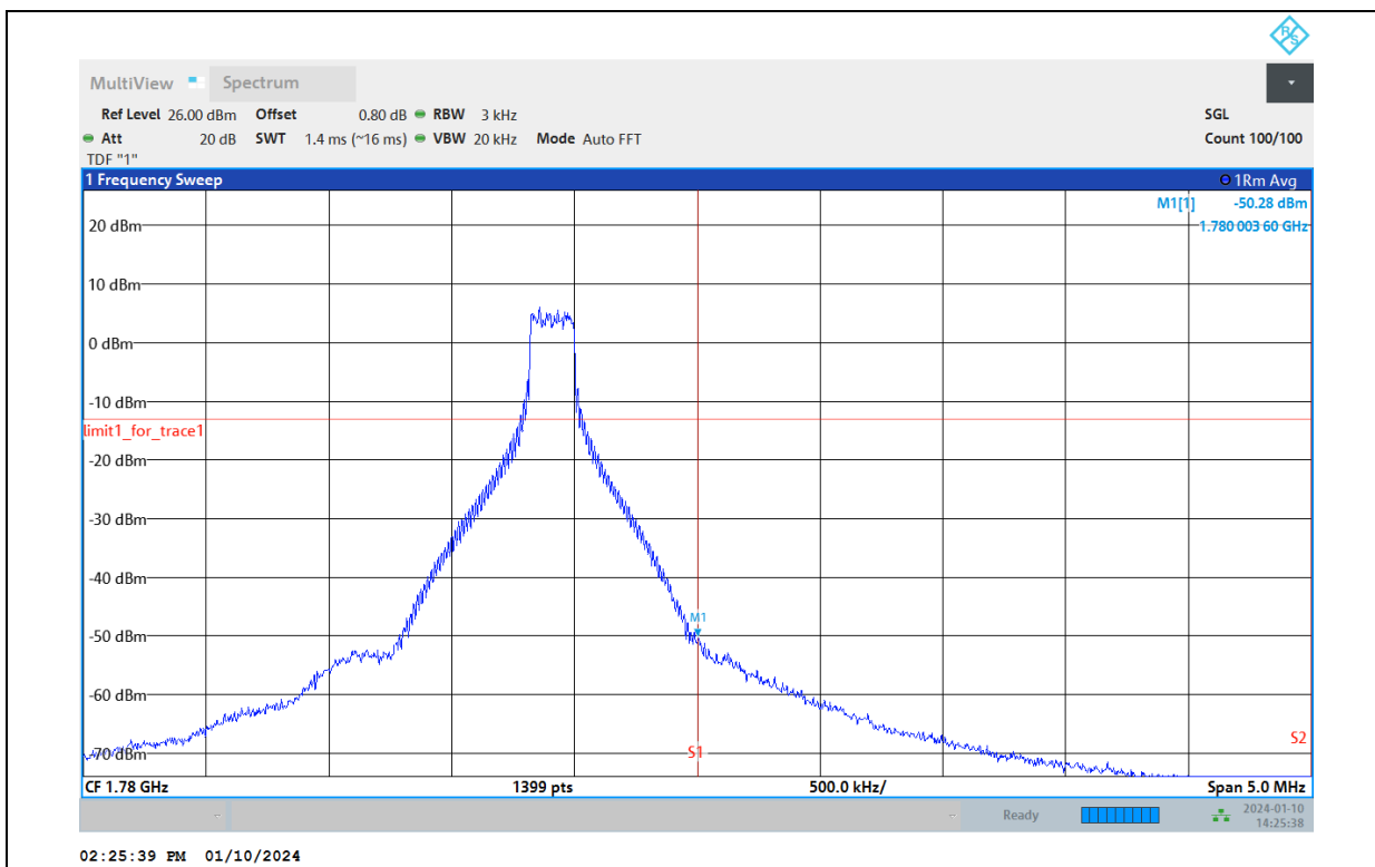
Band66-10MHz-64QAM-132622-50RB#0
