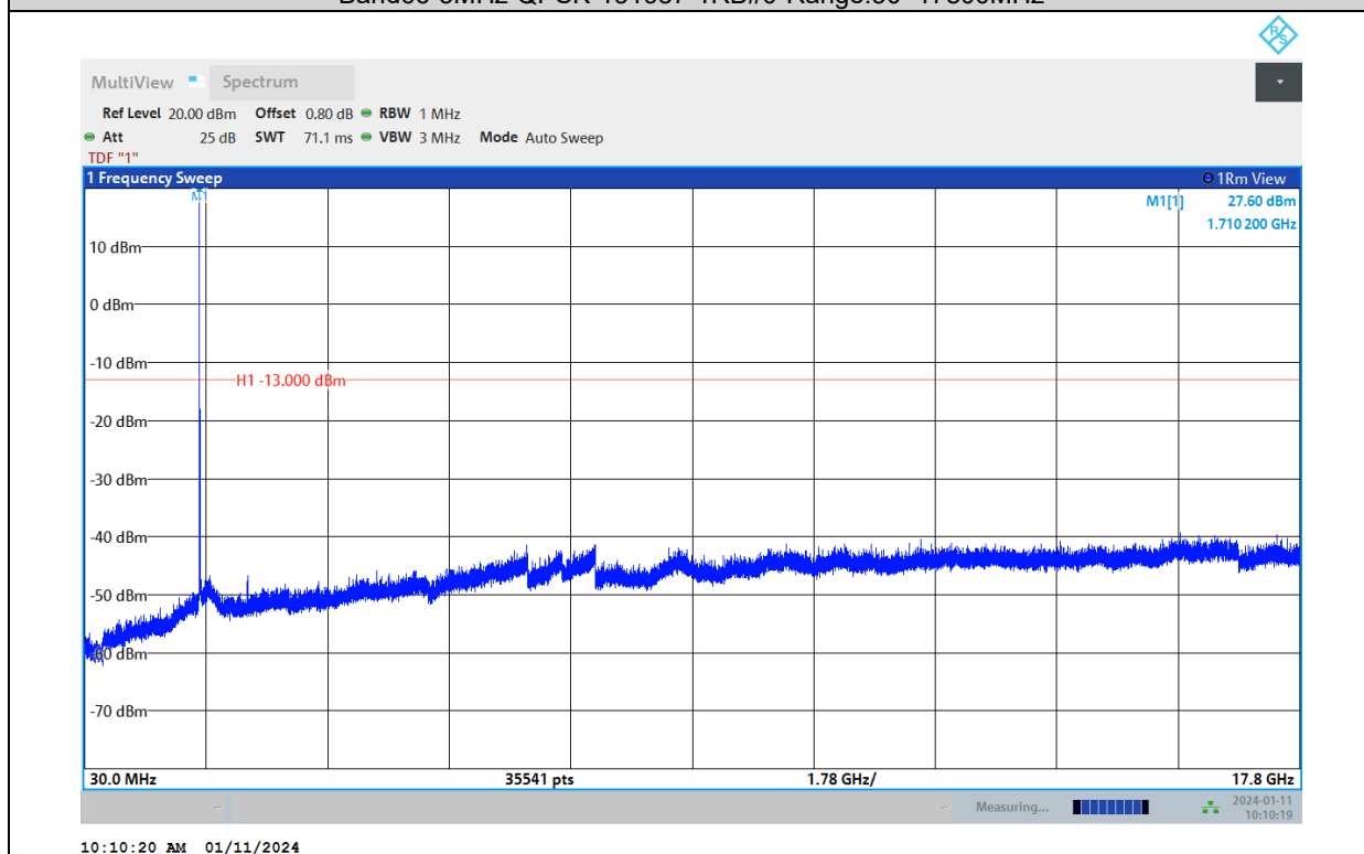
Band66-3MHz-QPSK-132322-1RB#0-Range:30~17800MHz
