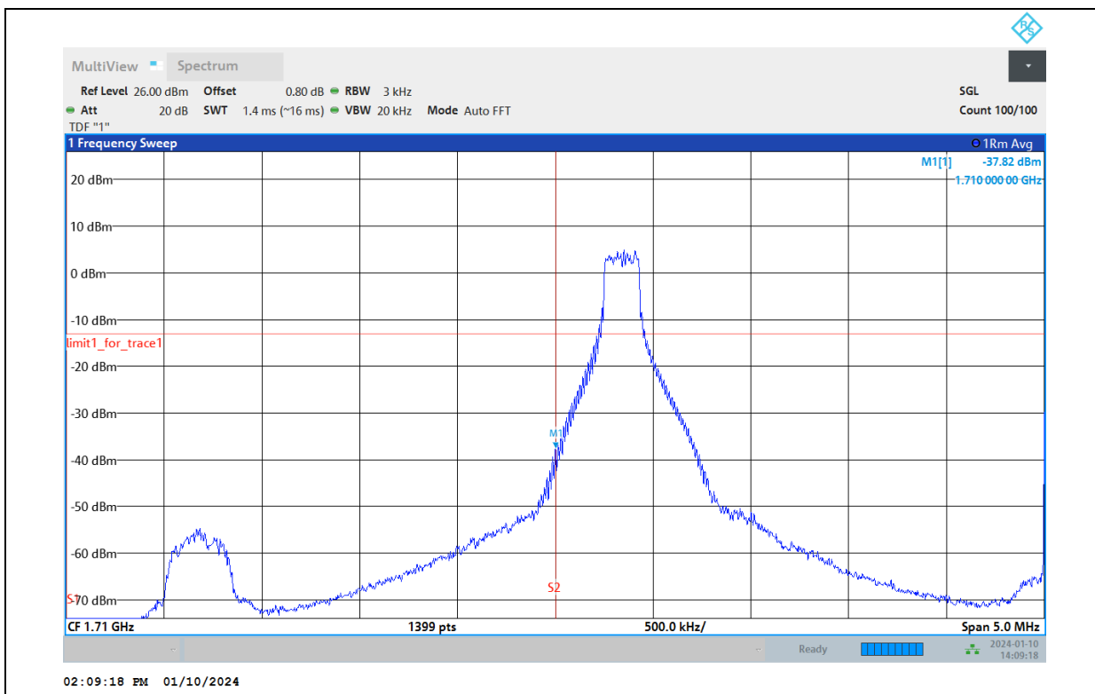
Band66-5MHz-64QAM-131997-25RB#0
