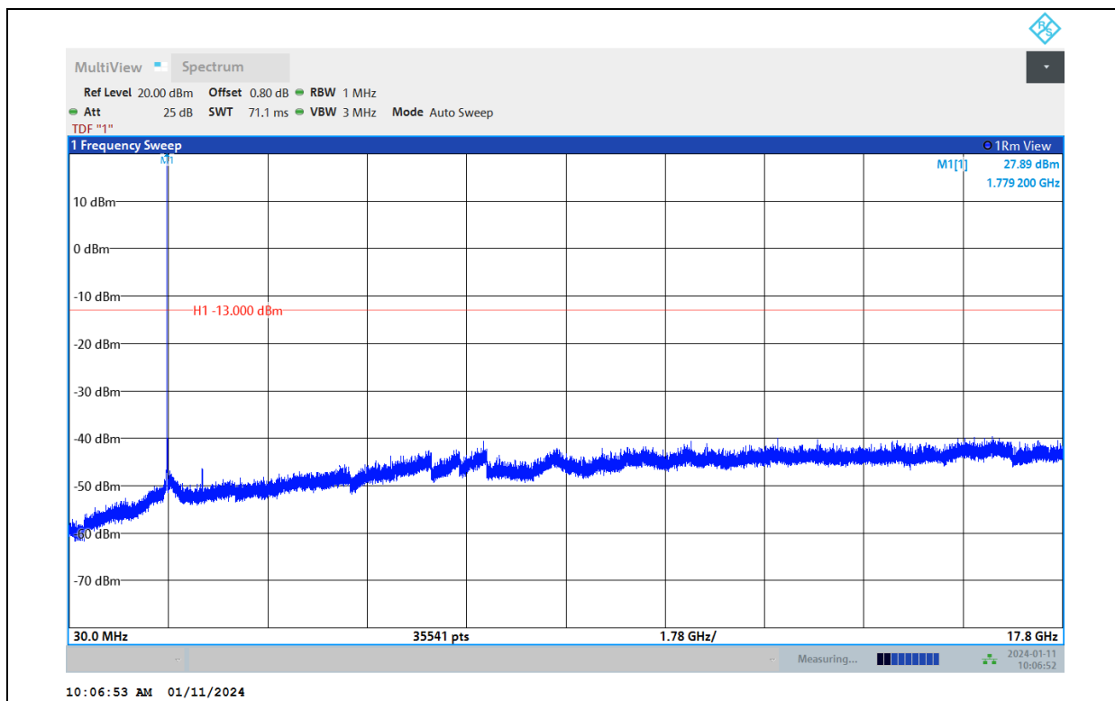
Band66-3MHz-QPSK-131987-1RB#0-Range:30~17800MHz
