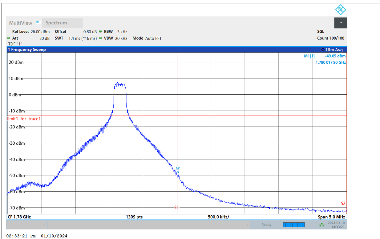
Band66-15MHz-QPSK-132597-75RB#0
