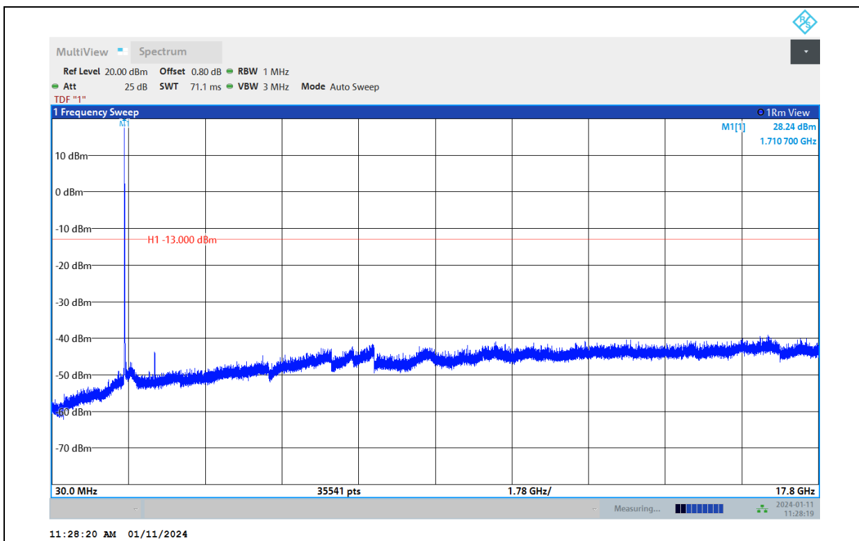
Band66-15MHz-16QAM-132322-1RB#0-Range:30~17800MHz
