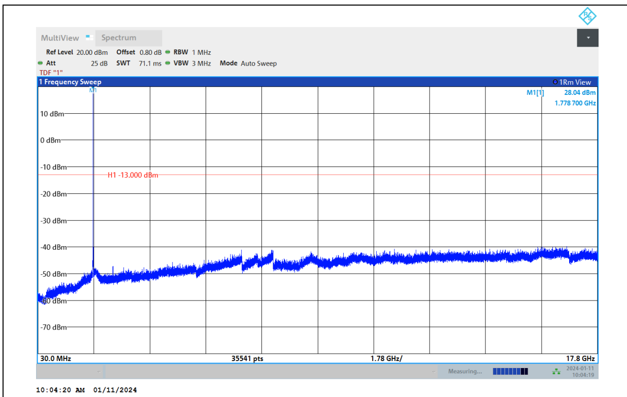
Band66-1.4MHz-16QAM-131979-1RB#0-Range:30~17800MHz
