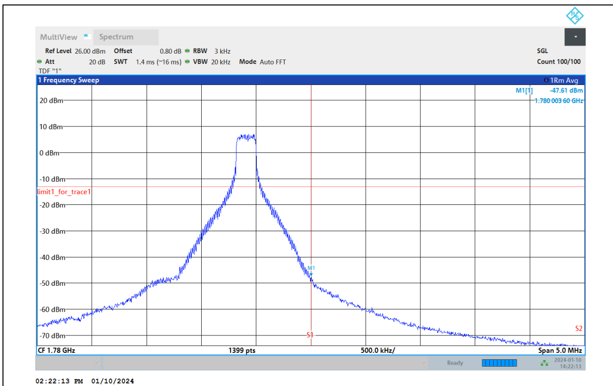
Band66-10MHz-QPSK-132622-50RB#0
