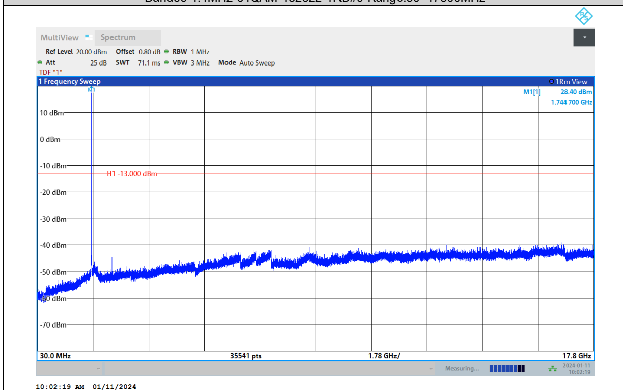
Band66-1.4MHz-64QAM-132665-1RB#0-Range:30~17800MHz
