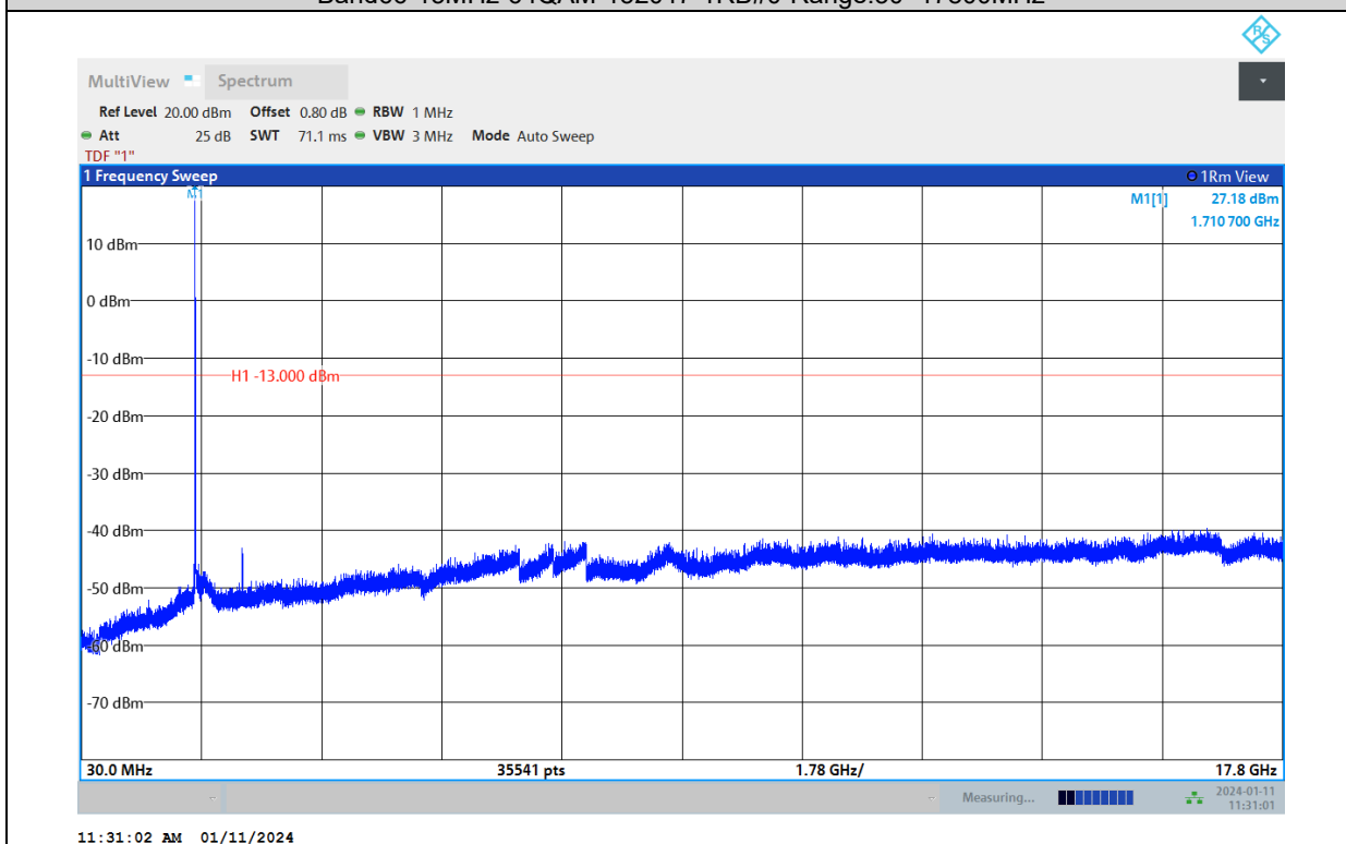
Band66-15MHz-64QAM-132322-1RB#0-Range:30~17800MHz
