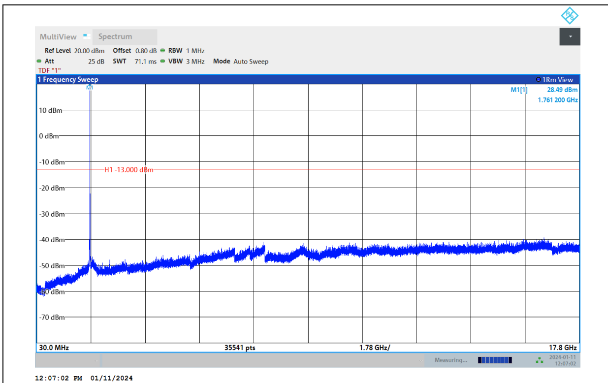
Band66-20MHz-16QAM-132072-1RB#0-Range:30~17800MHz
