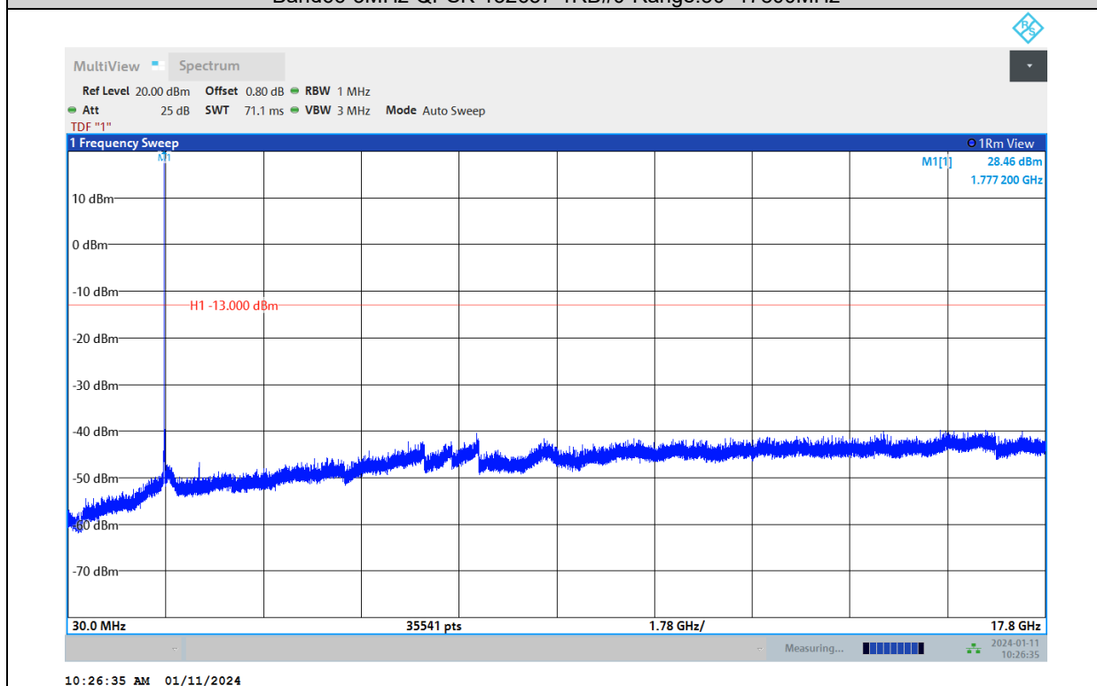
Band66-3MHz-16QAM-131987-1RB#0-Range:30~17800MHz
