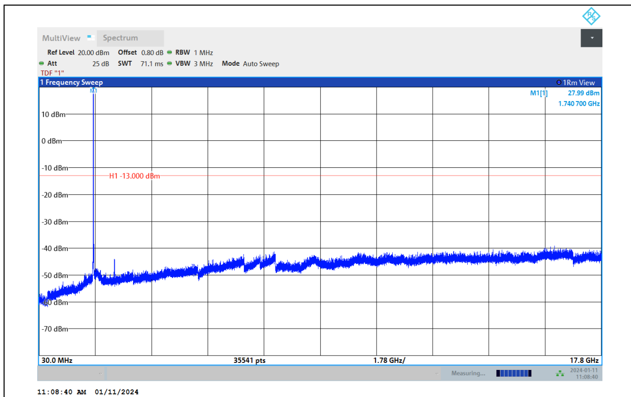
Band66-10MHz-QPSK-132622-1RB#0-Range:30~17800MHz
