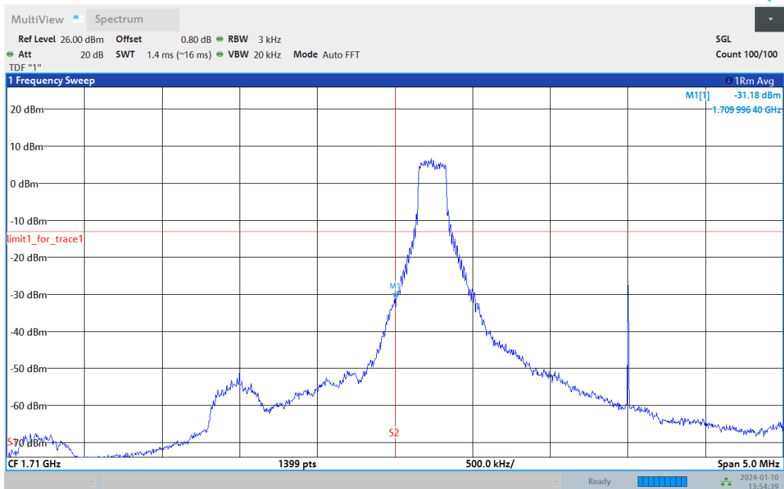
Band66-3MHz-QPSK-131987-15RB#0
