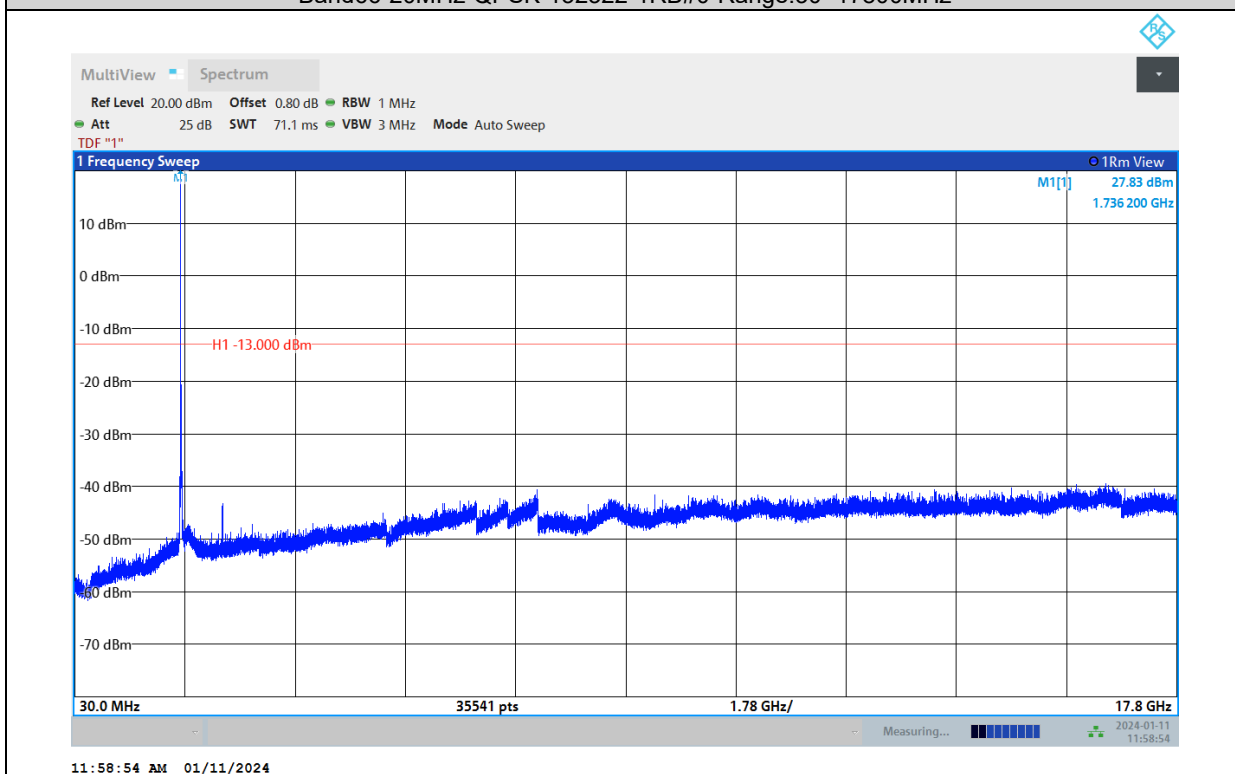
Band66-20MHz-QPSK-132572-1RB#0-Range:30~17800MHz
