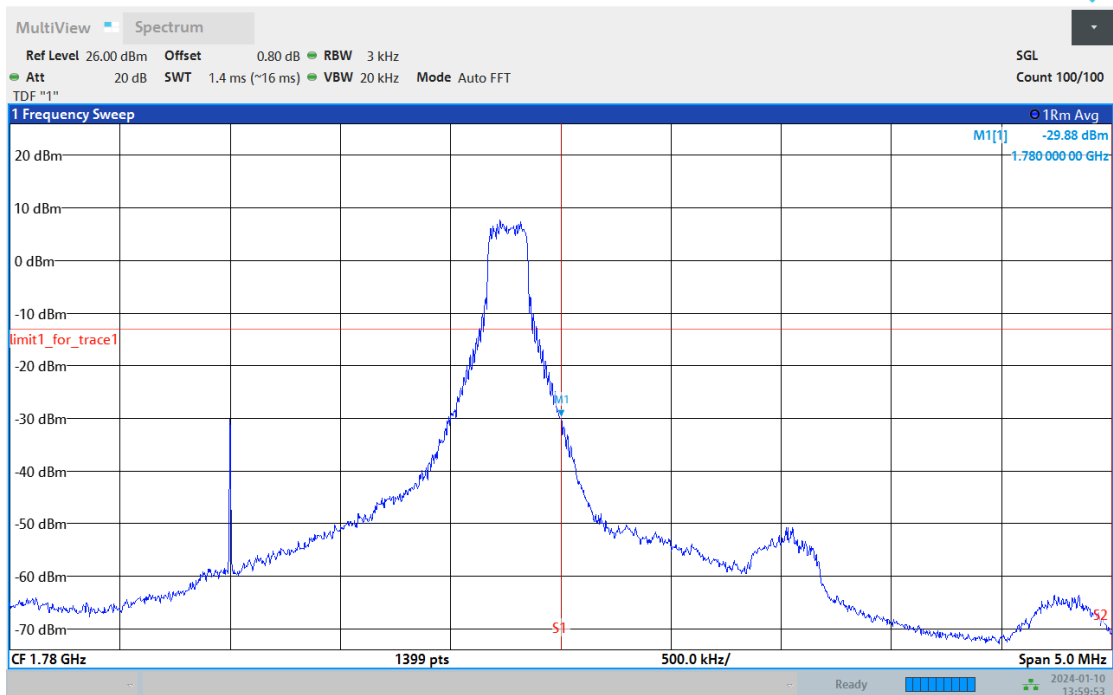
Band66-3MHz-QPSK-132657-15RB#0
