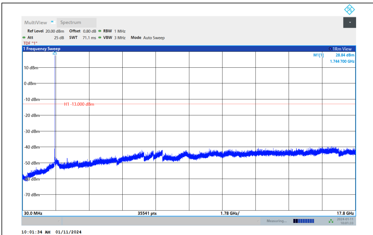
Band66-1.4MHz-16QAM-132665-1RB#0-Range:30~17800MHz
