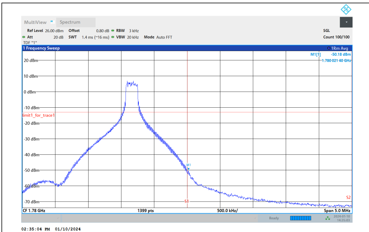
Band66-15MHz-16QAM-132597-75RB#0
