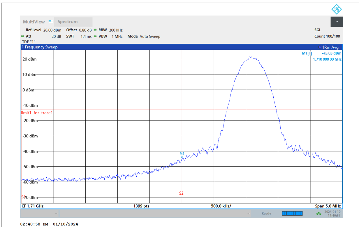
Band66-20MHz-16QAM-132072-100RB#0
