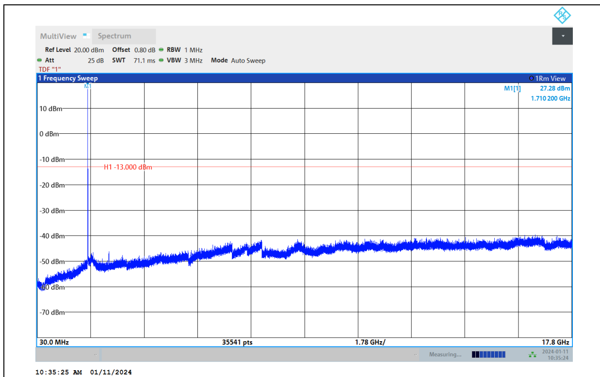
Band66-5MHz-QPSK-132322-1RB#0-Range:30~17800MHz
