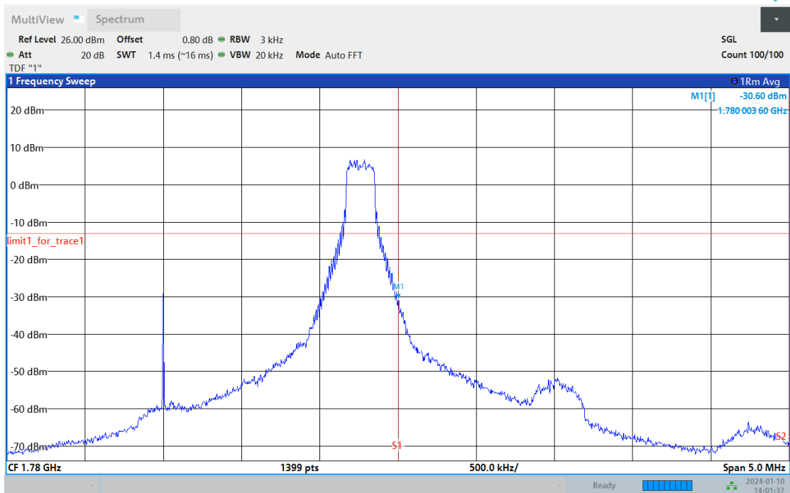
Band66-3MHz-16QAM-132657-15RB#0
