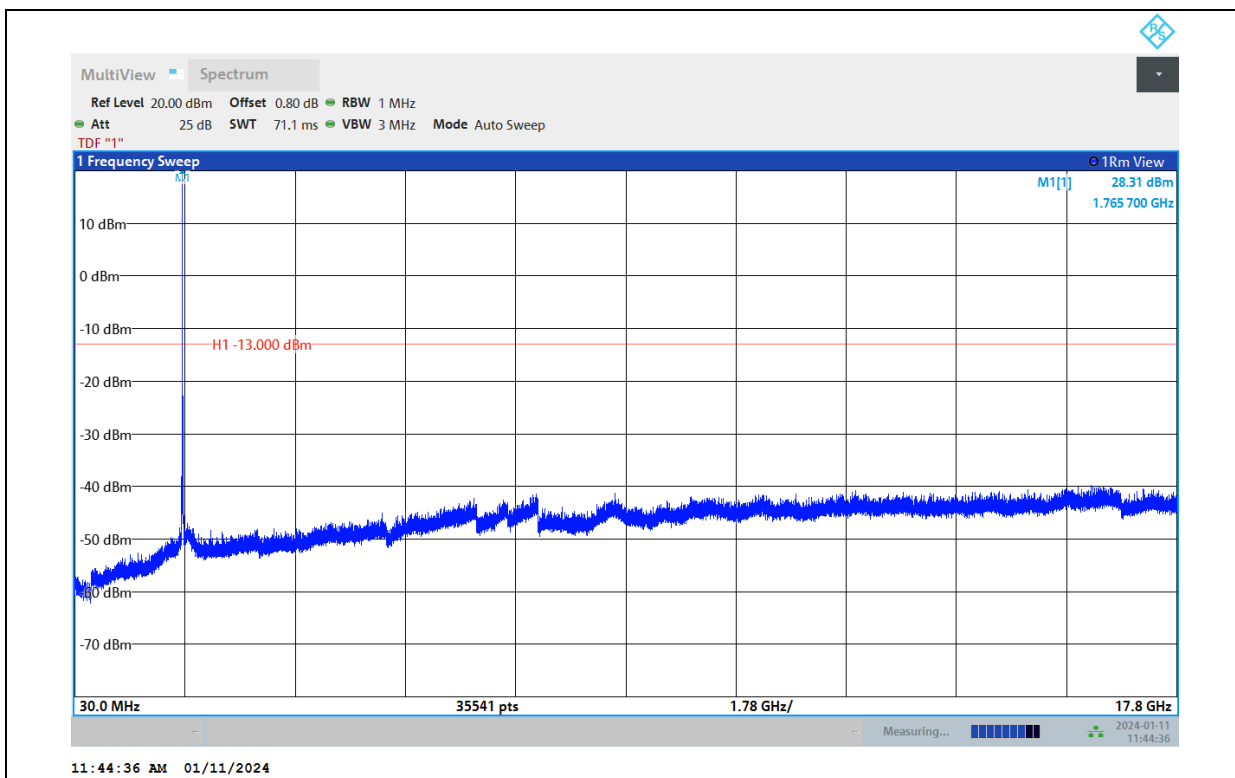
Band66-15MHz-64QAM-132047-1RB#0-Range:30~17800MHz
