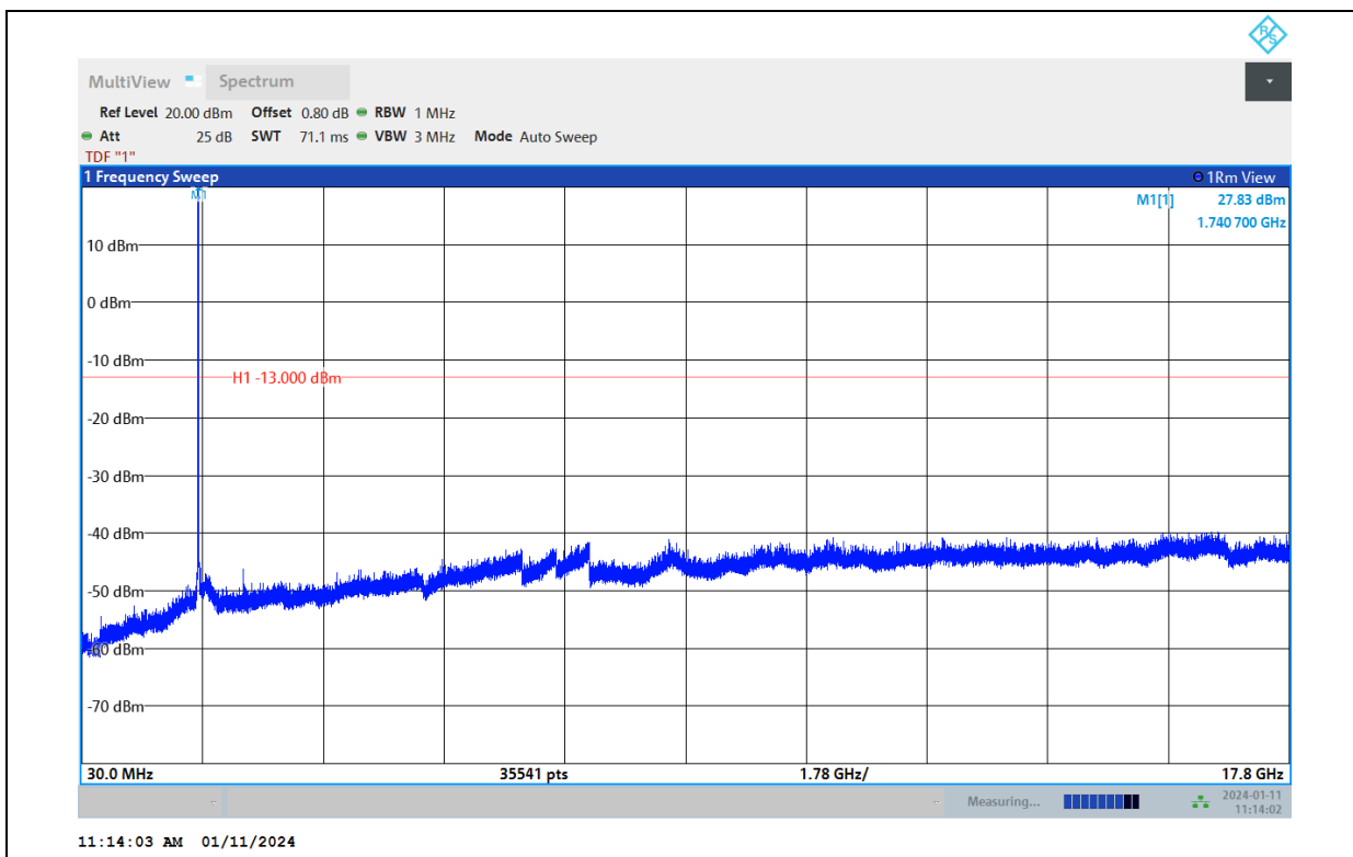
Band66-10MHz-64QAM-132622-1RB#0-Range:30~17800MHz
