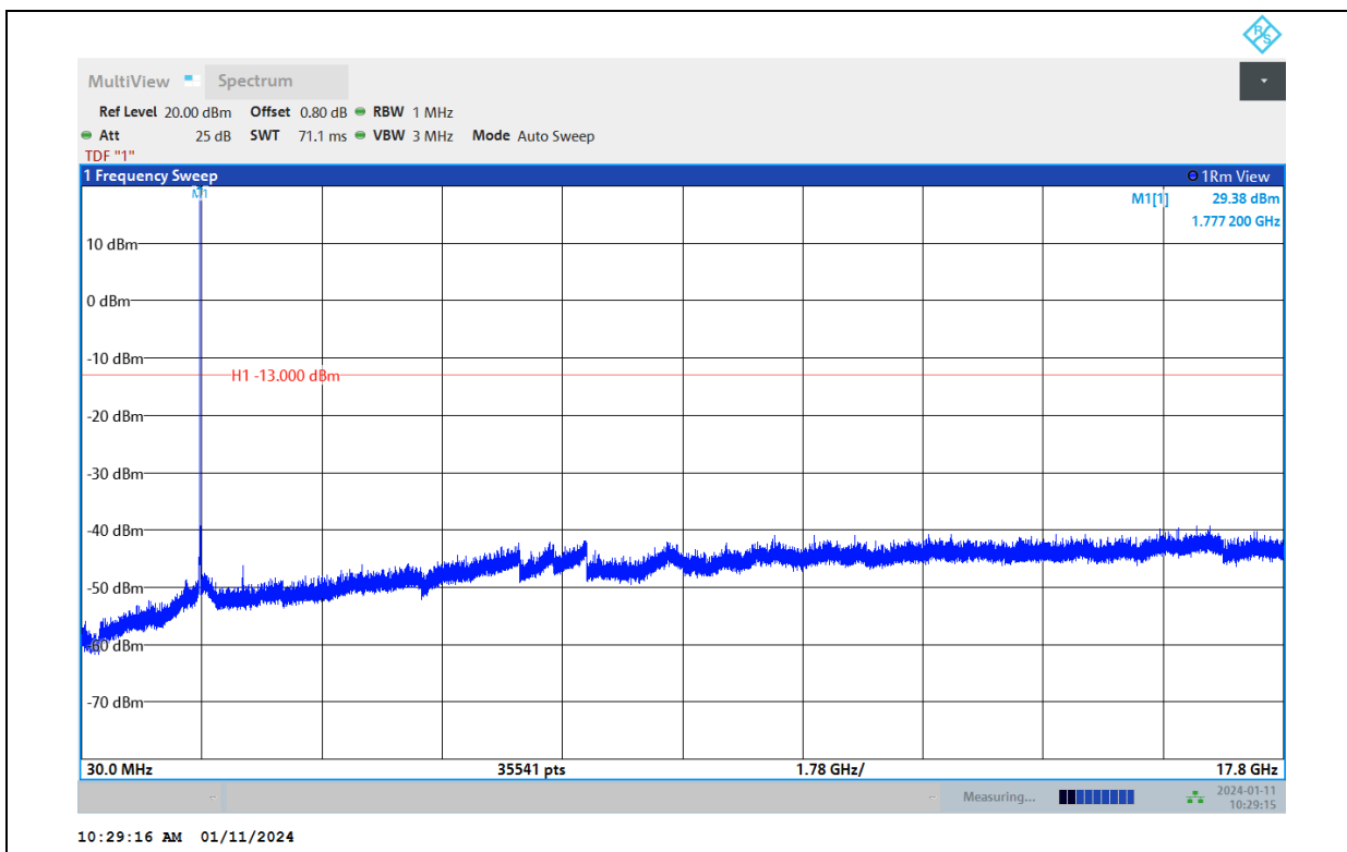
Band66-3MHz-64QAM-131987-1RB#0-Range:30~17800MHz
