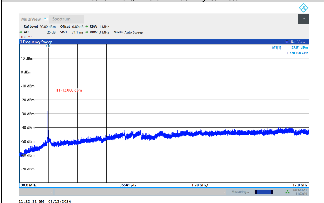
Band66-15MHz-QPSK-132047-1RB#0-Range:30~17800MHz
