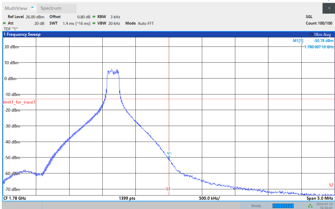
Band66-15MHz-64QAM-132597-75RB#0
