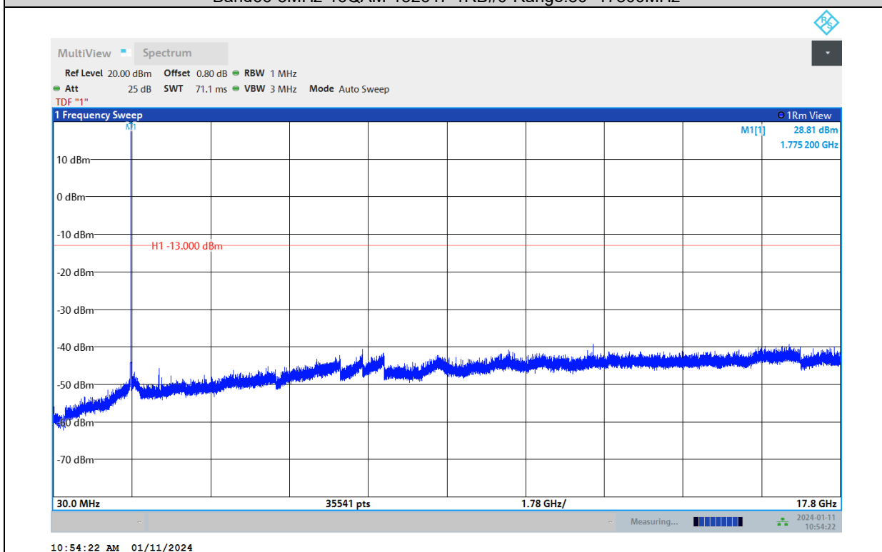
Band66-5MHz-64QAM-131997-1RB#0-Range:30~17800MHz
