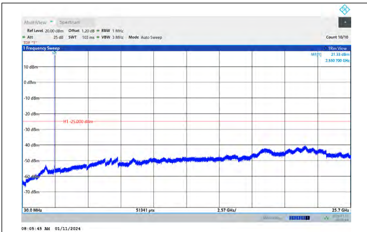
Band7-10MHz-QPSK-21400-1RB#0-Range:30~25700MHz
