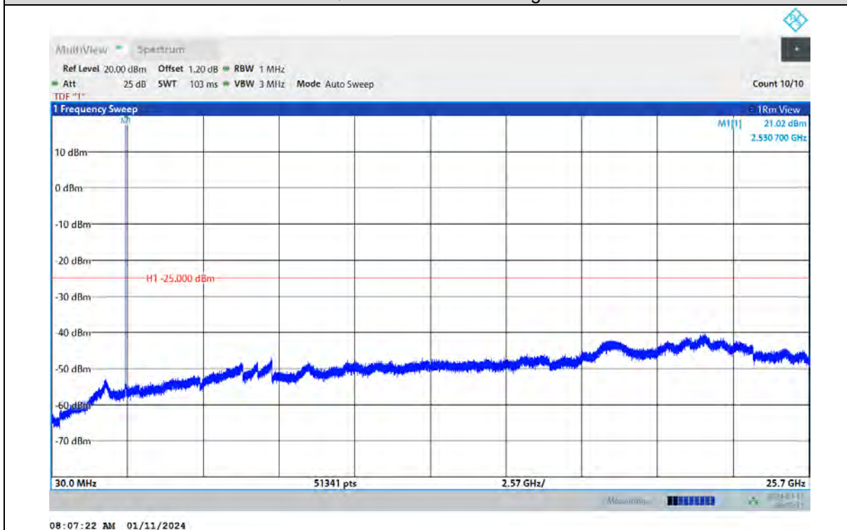
Band7-10MHz-16QAM-21400-1RB#0-Range:30~25700MHz
