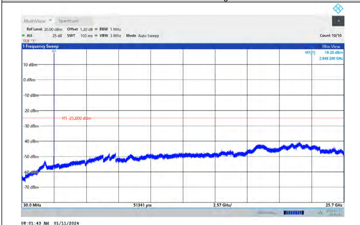
Band7-5MHz-64QAM-20775-1RB#0-Range:30~25700MHz
