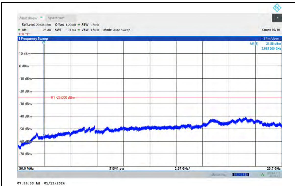
Band7-5MHz-16QAM-21425-1RB#0-Range:30~25700MHz
