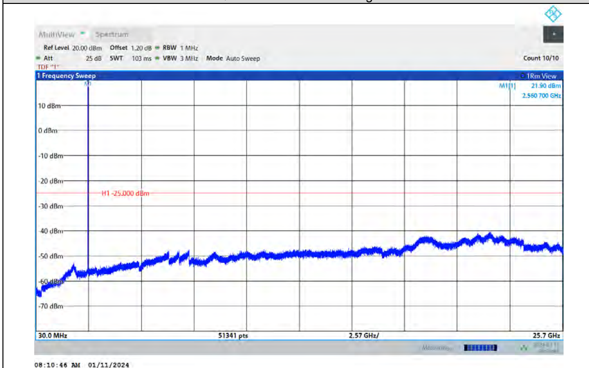
Band7-10MHz-16QAM-20800-1RB#0-Range:30~25700MHz
