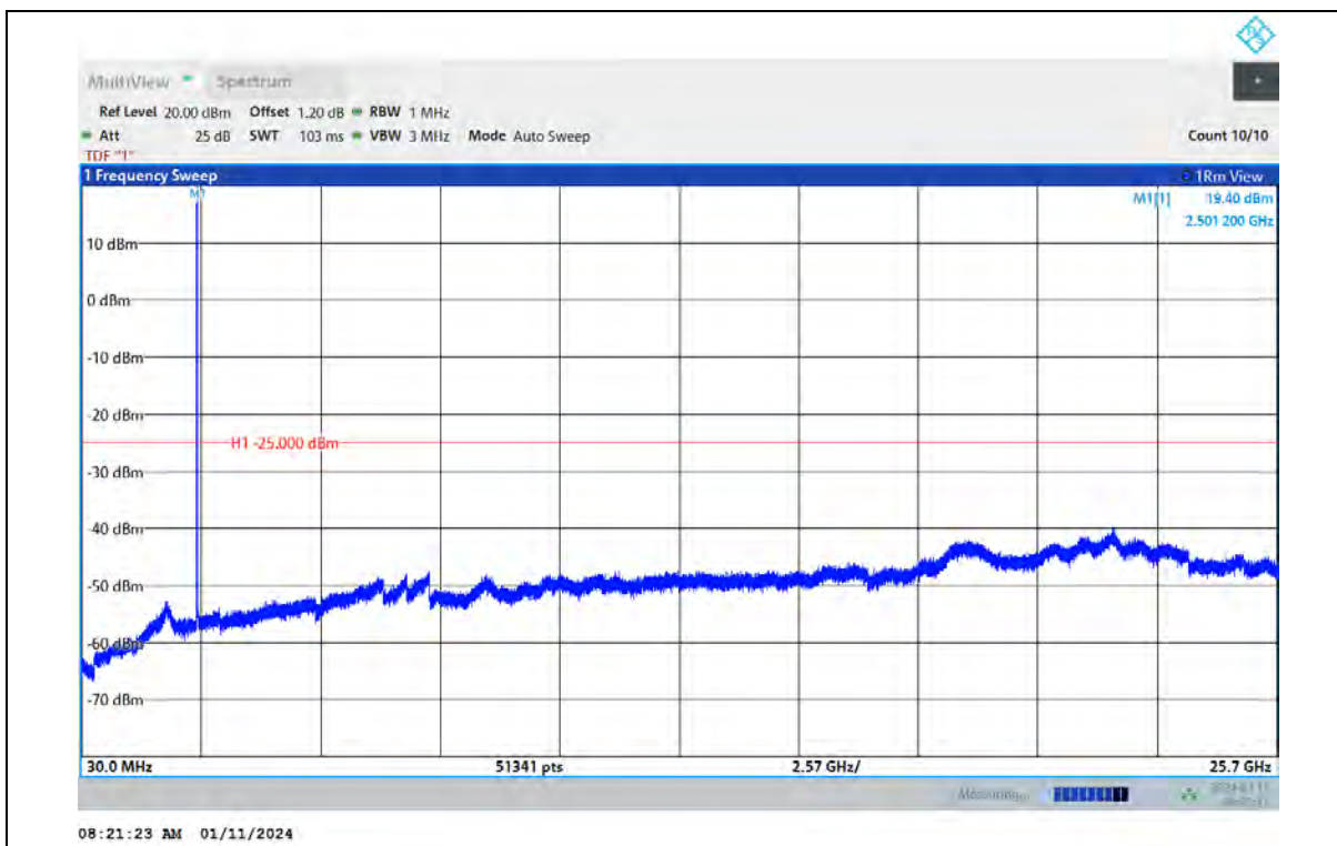
Band7-20MHz-16QAM-21100-1RB#0-Range:30~25700MHz
