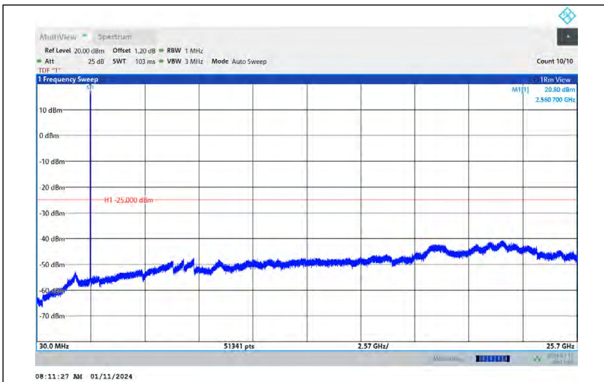
Band7-10MHz-64QAM-20800-1RB#0-Range:30~25700MHz
