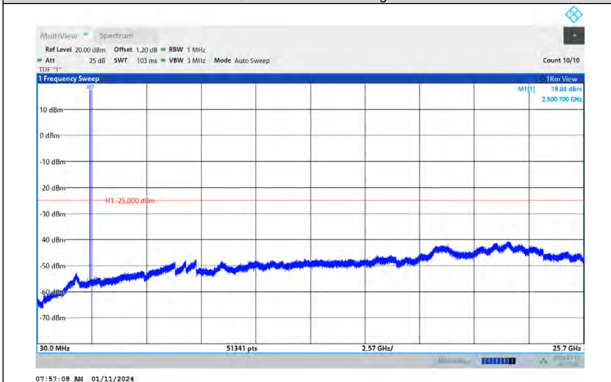
Band7-5MHz-16QAM-21100-1RB#0-Range:30~25700MHz
