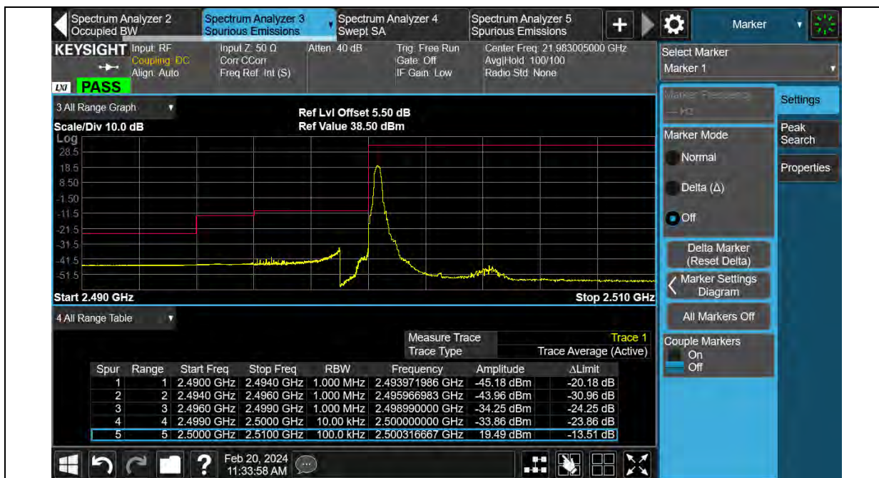
Band7-5MHz-16QAM-20775-25RB#0
