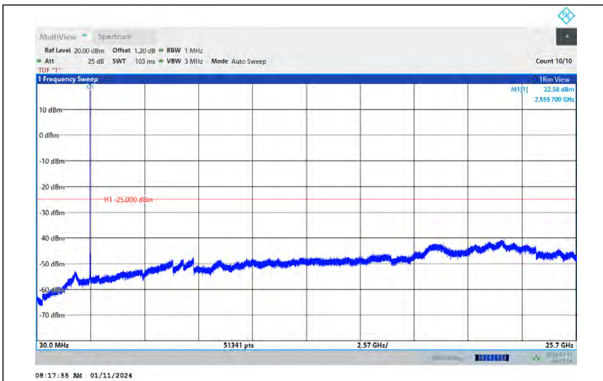
Band7-15MHz-16QAM-20825-1RB#0-Range:30~25700MHz
