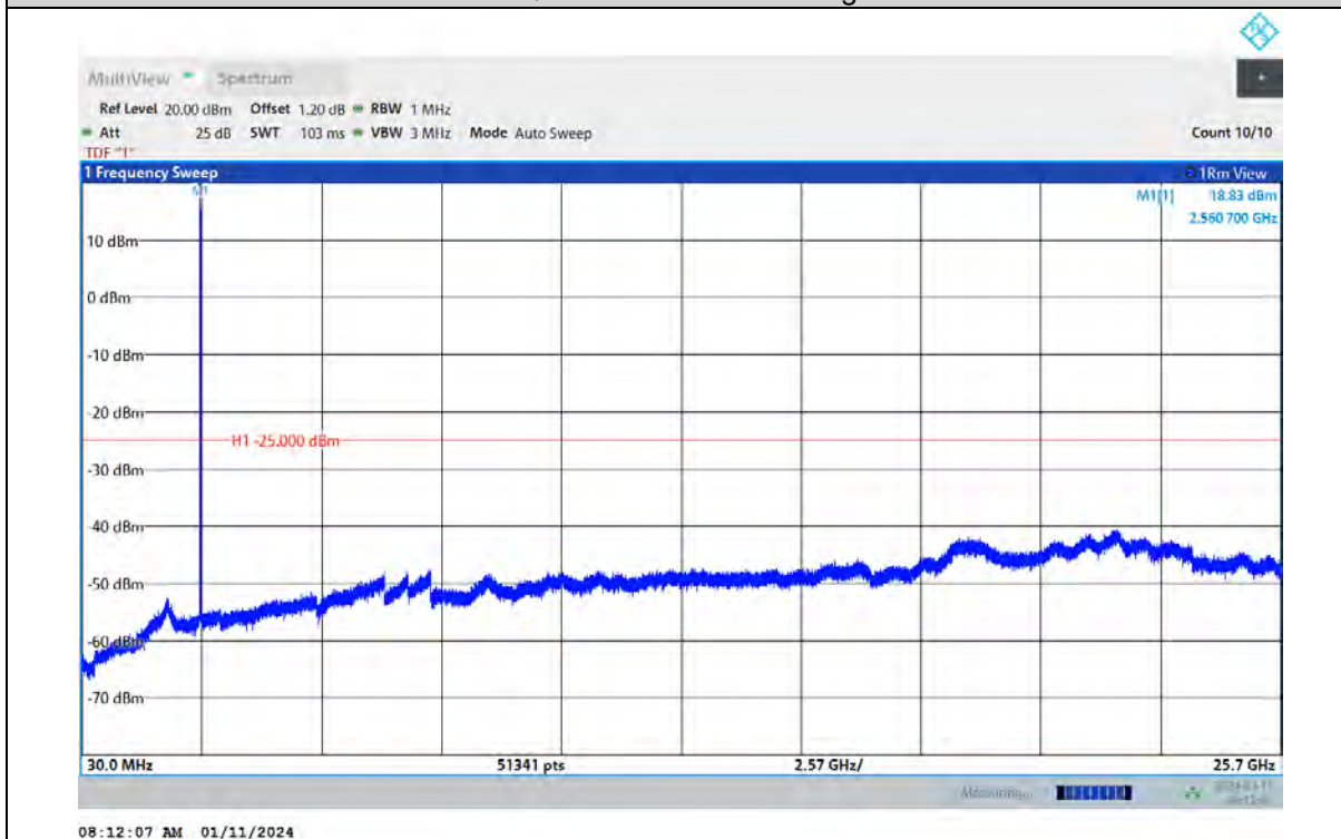
Band7-15MHz-QPSK-20825-1RB#0-Range:30~25700MHz
