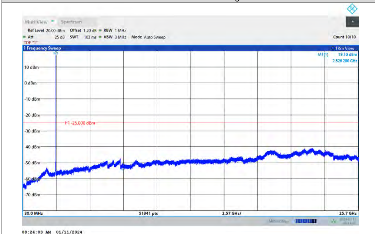
Band7-20MHz-16QAM-21350-1RB#0-Range:30~25700MHz
