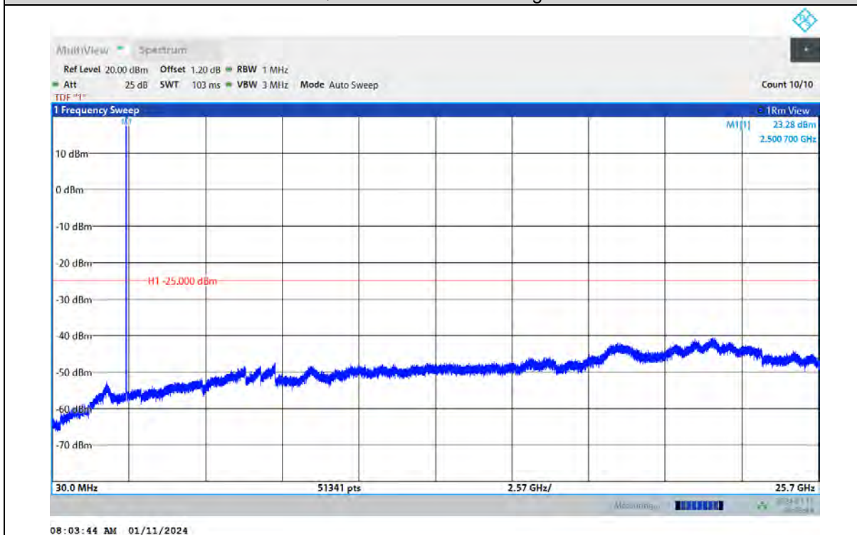
Band7-10MHz-QPSK-21100-1RB#0-Range:30~25700MHz
