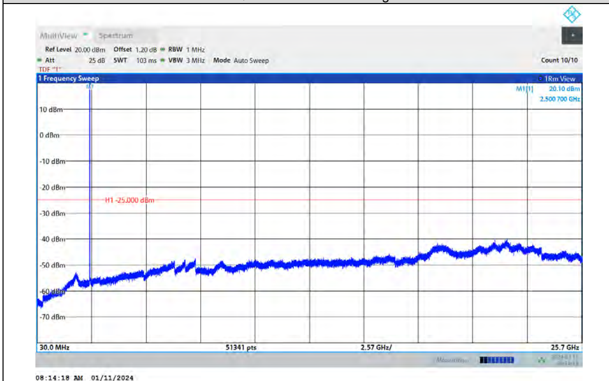
Band7-15MHz-16QAM-21100-1RB#0-Range:30~25700MHz
