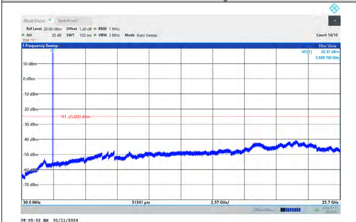
Band7-10MHz-64QAM-21100-1RB#0-Range:30~25700MHz
