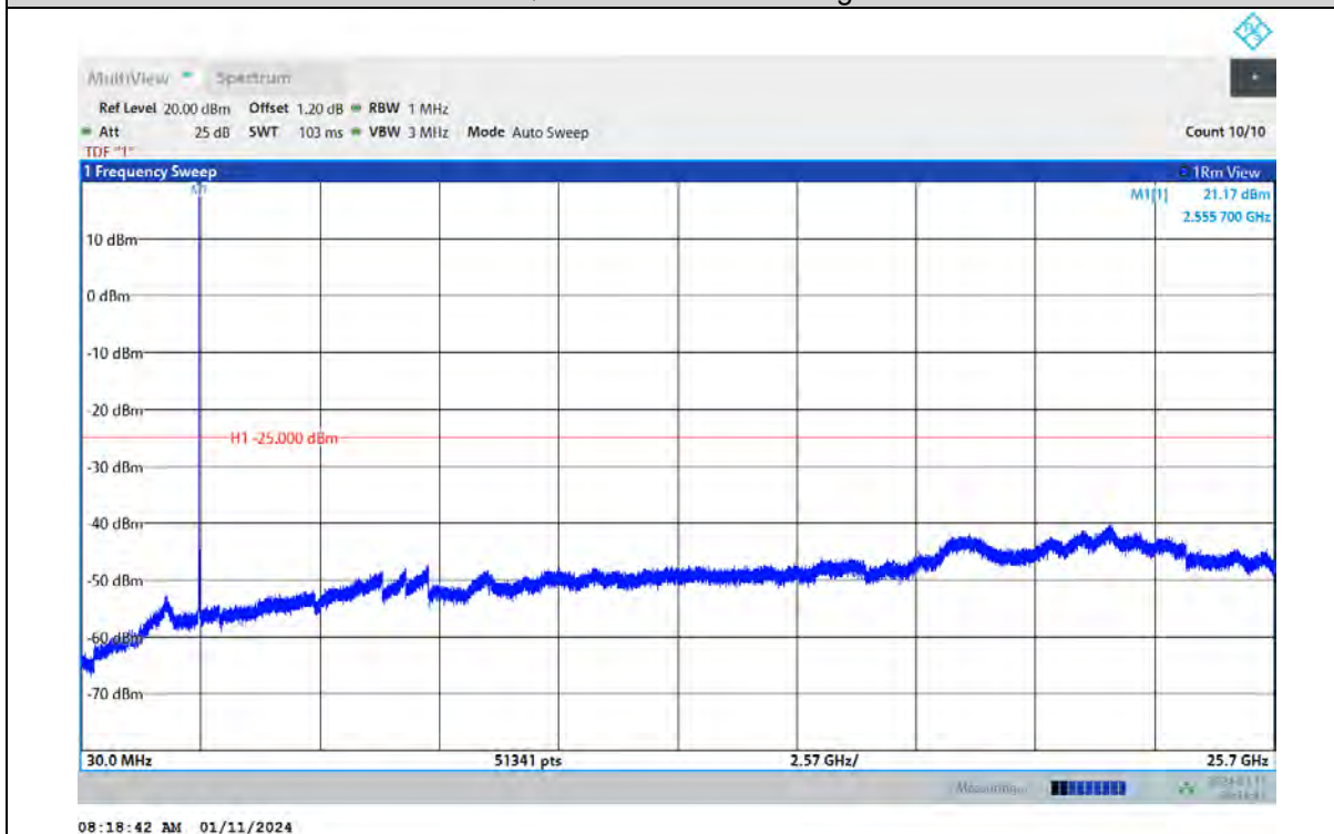
Band7-15MHz-64QAM-20825-1RB#0-Range:30~25700MHz
