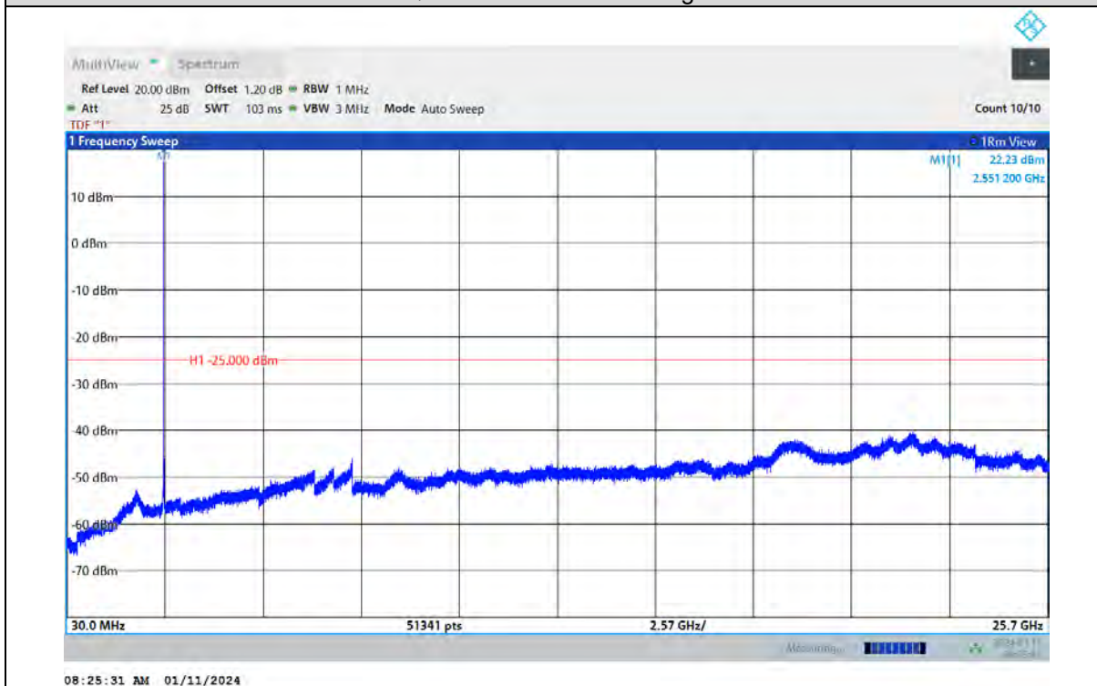
Band7-20MHz-16QAM-20850-1RB#0-Range:30~25700MHz
