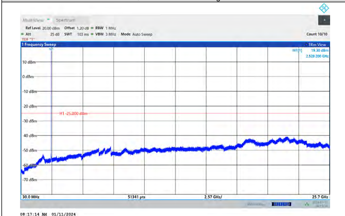
Band7-15MHz-64QAM-21375-1RB#0-Range:30~25700MHz
