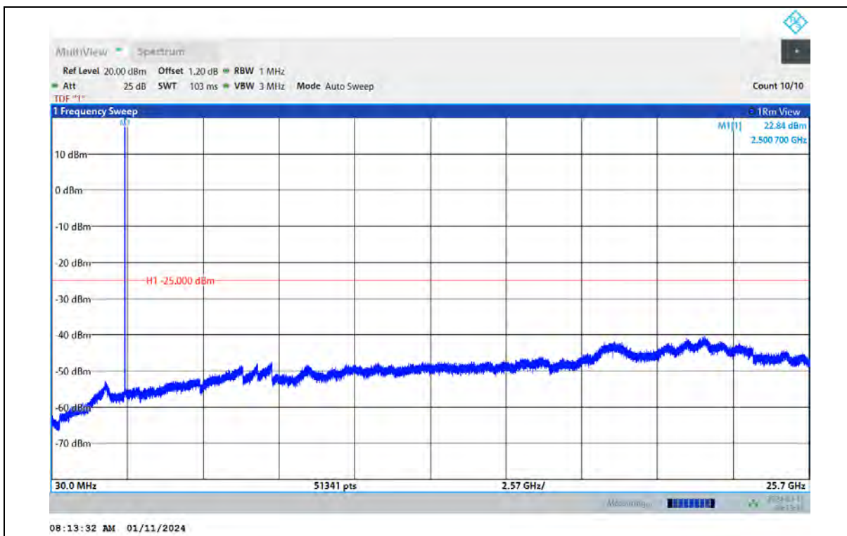
Band7-15MHz-QPSK-21100-1RB#0-Range:30~25700MHz
