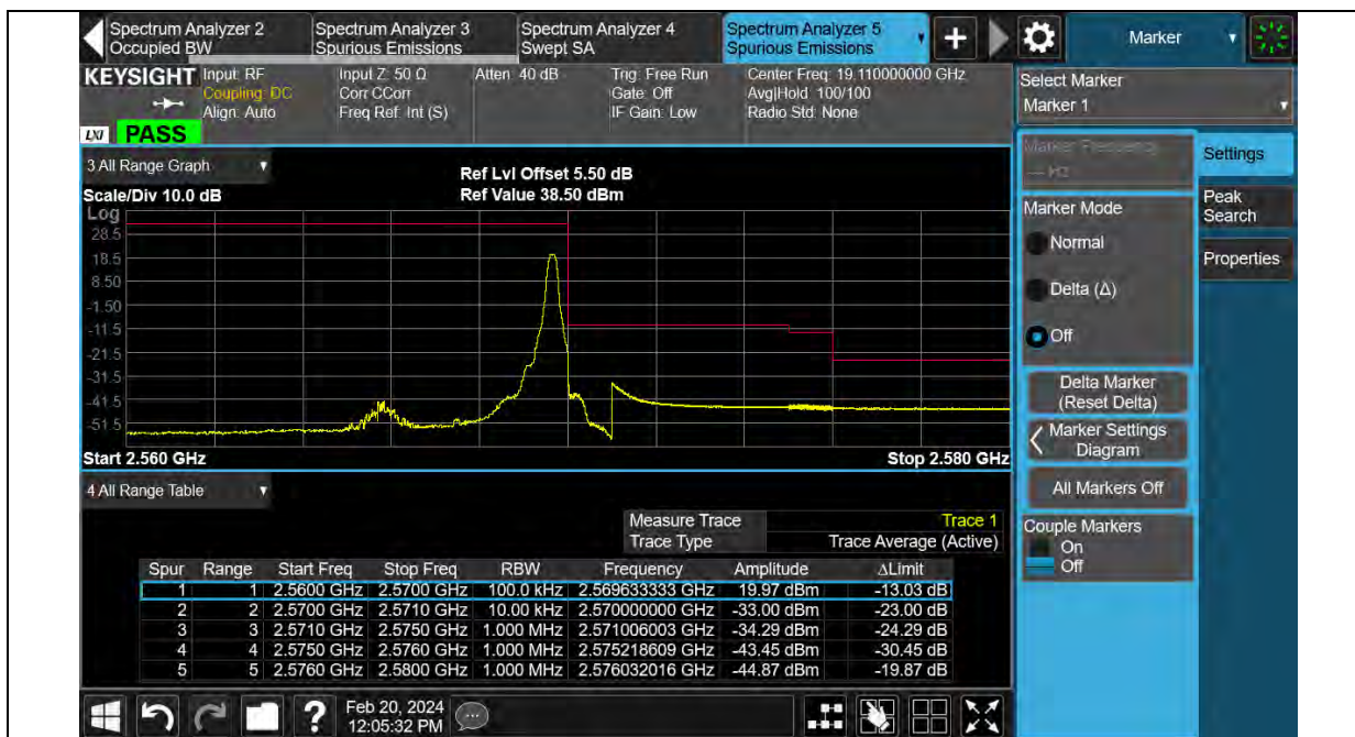
Band7-5MHz-16QAM-21425-25RB#0
