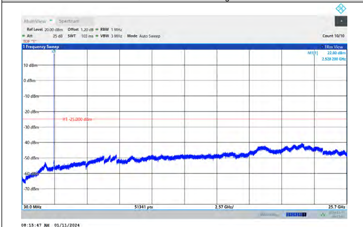
Band7-15MHz-QPSK-21375-1RB#0-Range:30~25700MHz
