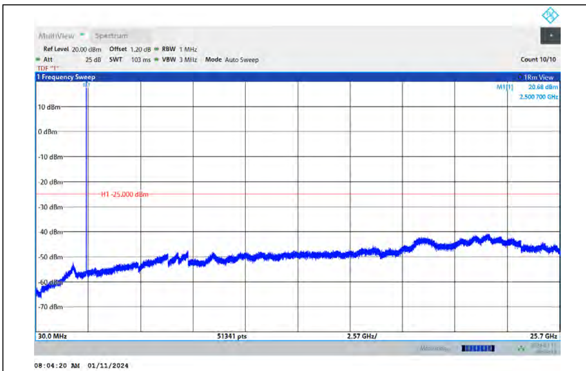
Band7-10MHz-16QAM-21100-1RB#0-Range:30~25700MHz
