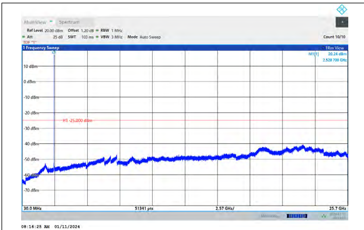
Band7-15MHz-16QAM-21375-1RB#0-Range:30~25700MHz
