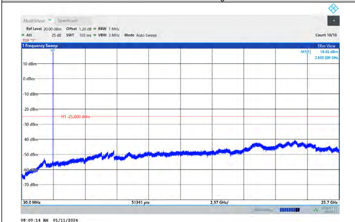
Band7-5MHz-64QAM-21425-1RB#0-Range:30~25700MHz
