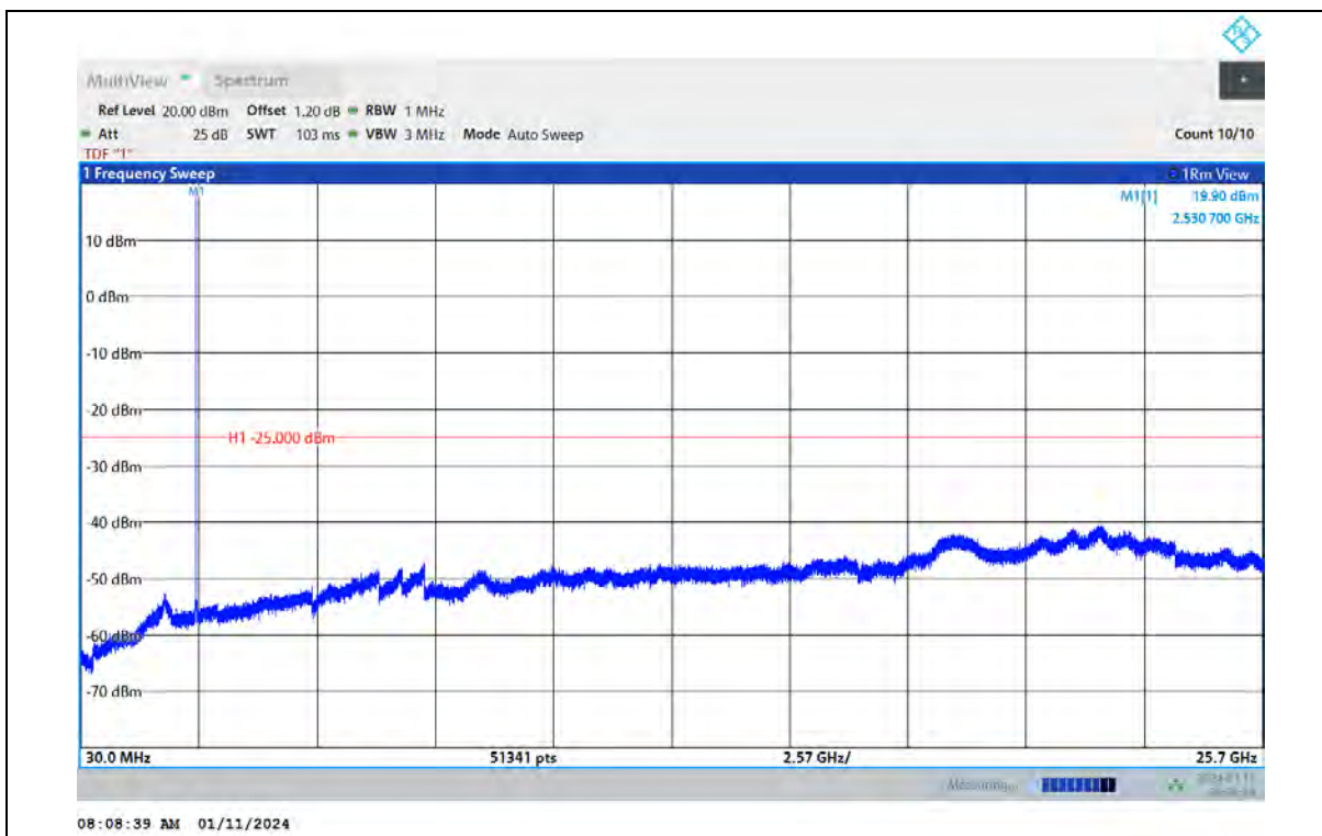
Band7-10MHz-64QAM-21400-1RB#0-Range:30~25700MHz
