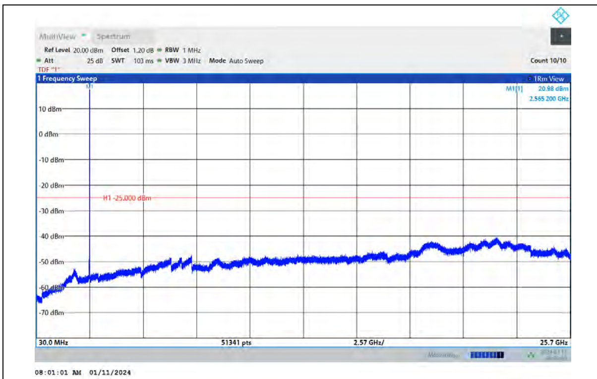
Band7-5MHz-16QAM-20775-1RB#0-Range:30~25700MHz
