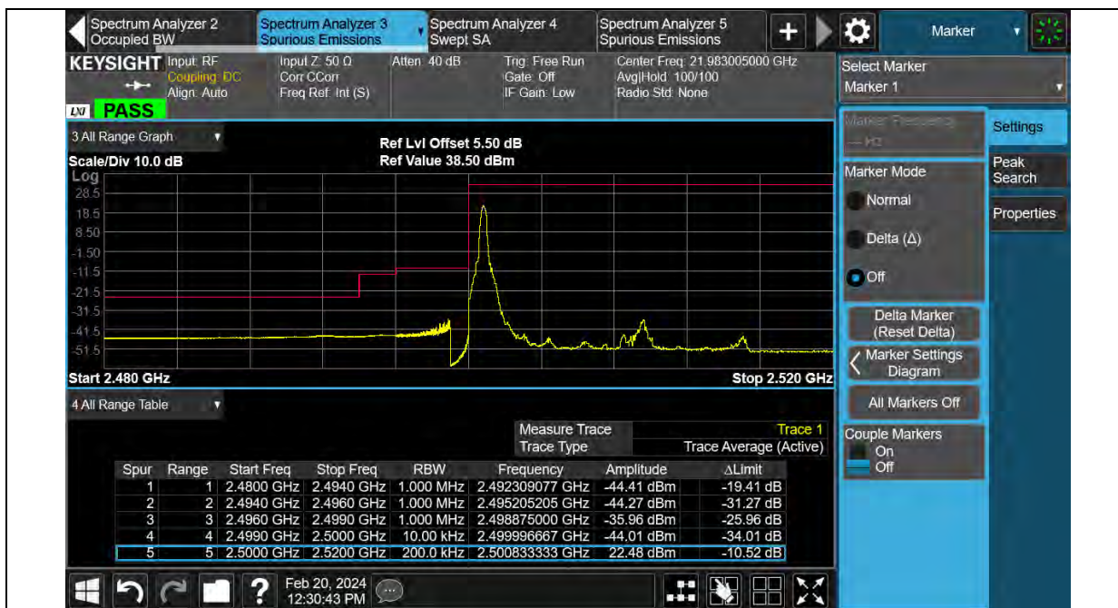
Band7-15MHz-QPSK-20825-75RB#0
