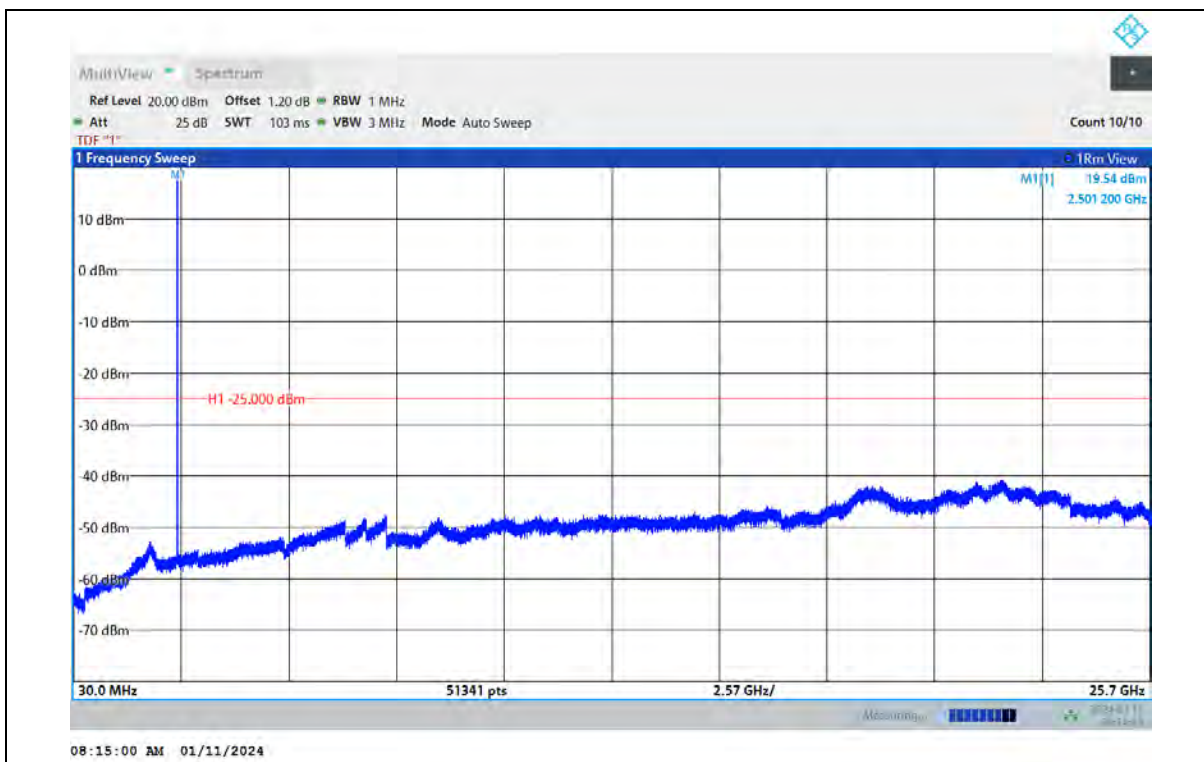
Band7-15MHz-64QAM-21100-1RB#0-Range:30~25700MHz
