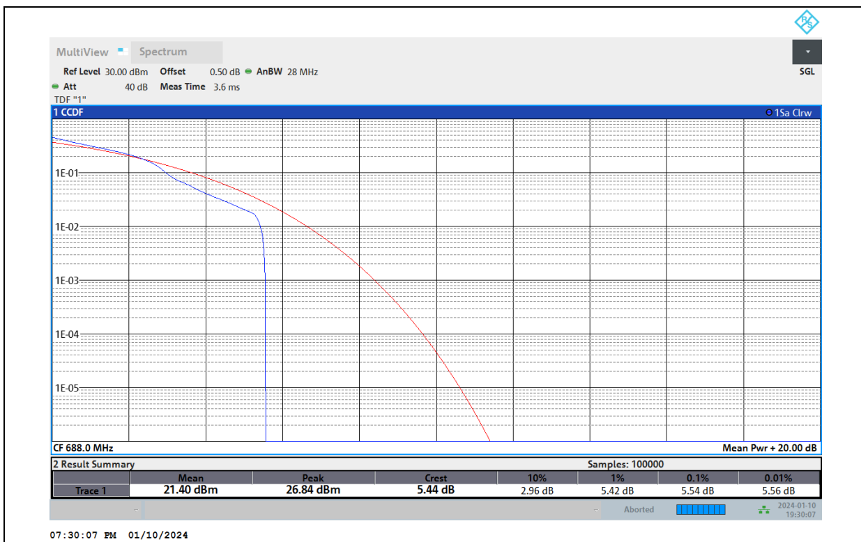
Band71-20MHz-16QAM-133372-100RB#0
