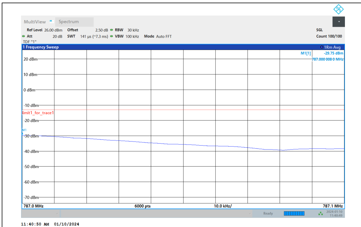
Band13-5MHz-16QAM-23255-1RB#24-P2
