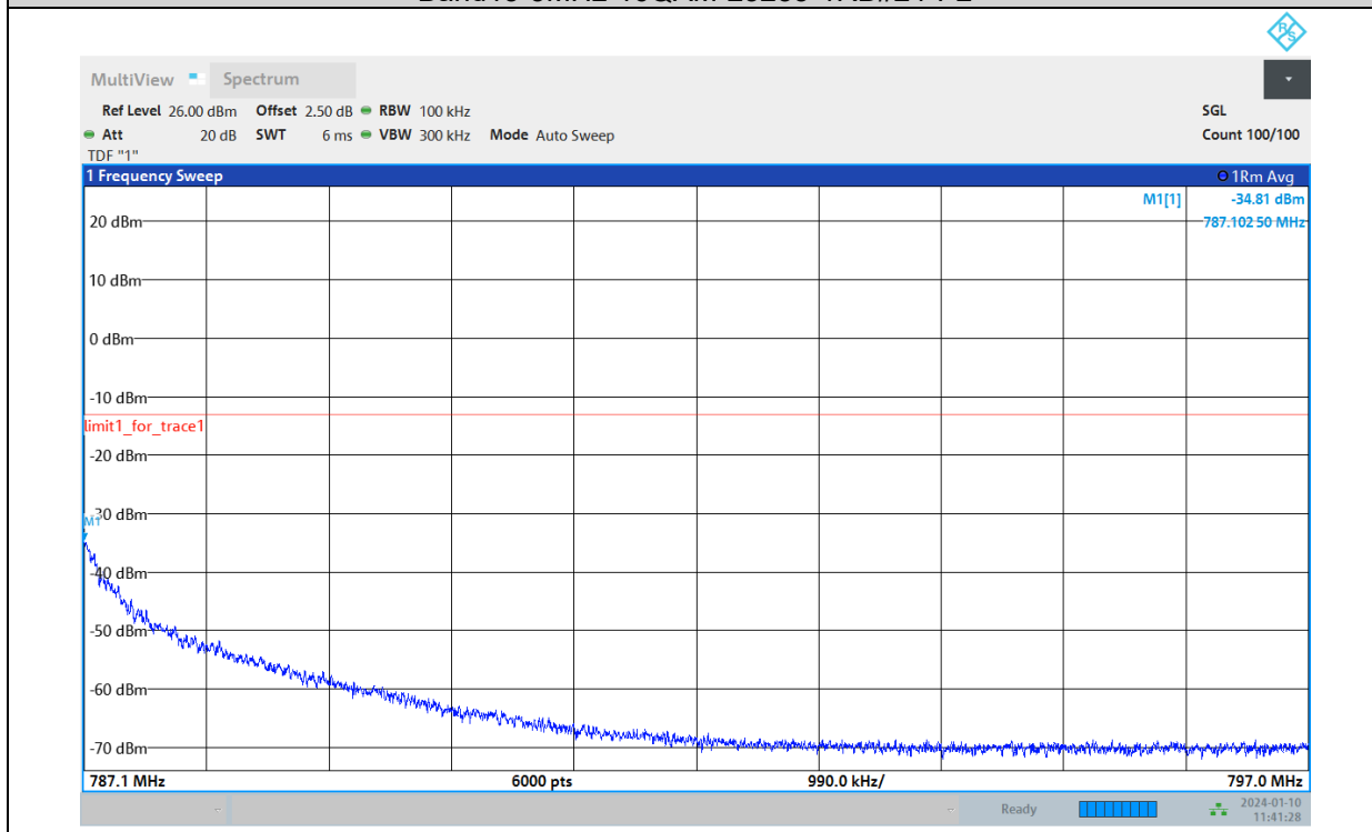
Band13-5MHz-16QAM-23255-1RB#24-P2
