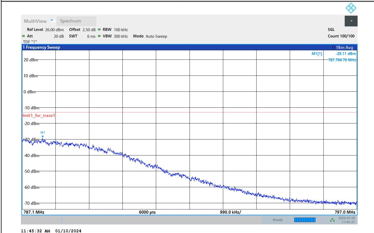
Band13-10MHz-QPSK-23230-1RB#0
