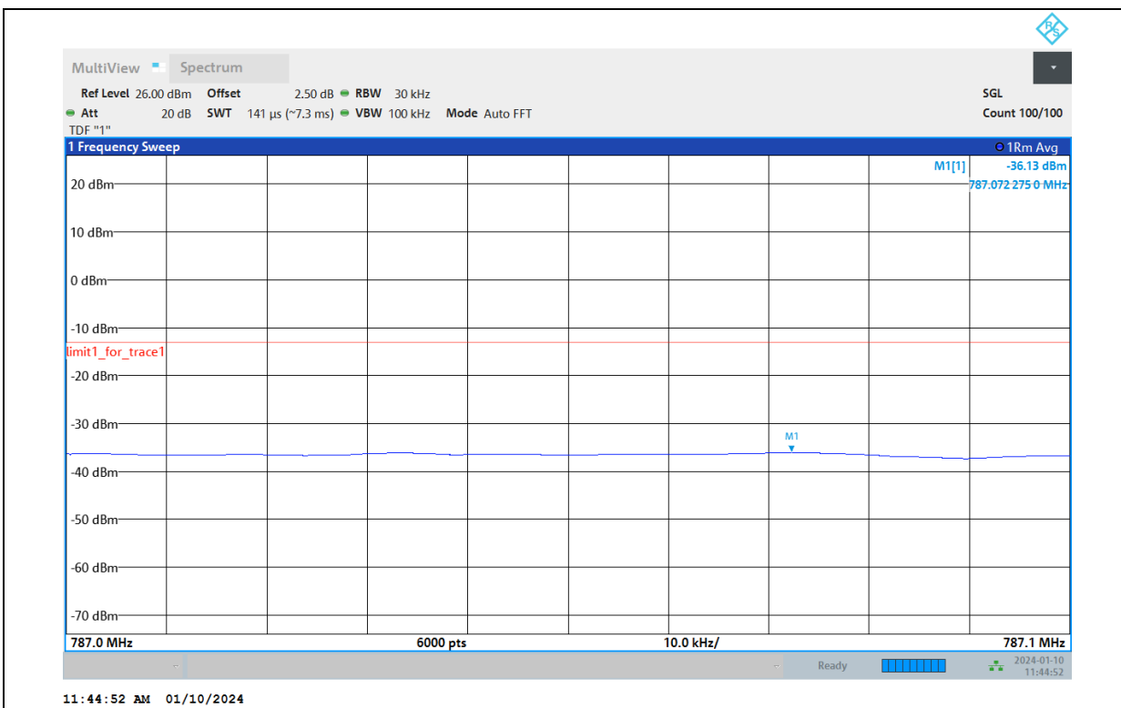
Band13-5MHz-64QAM-23255-25RB#0-P2
