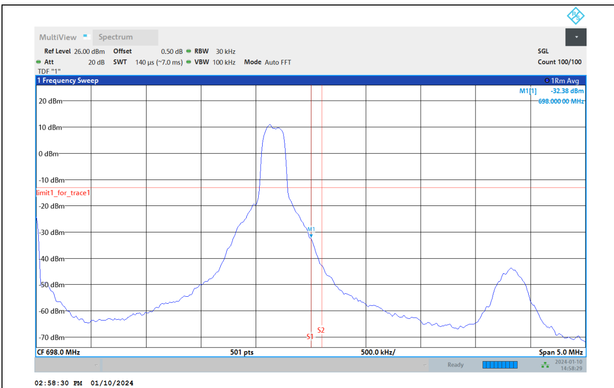
Band71-5MHz-64QAM-133447-25RB#0
