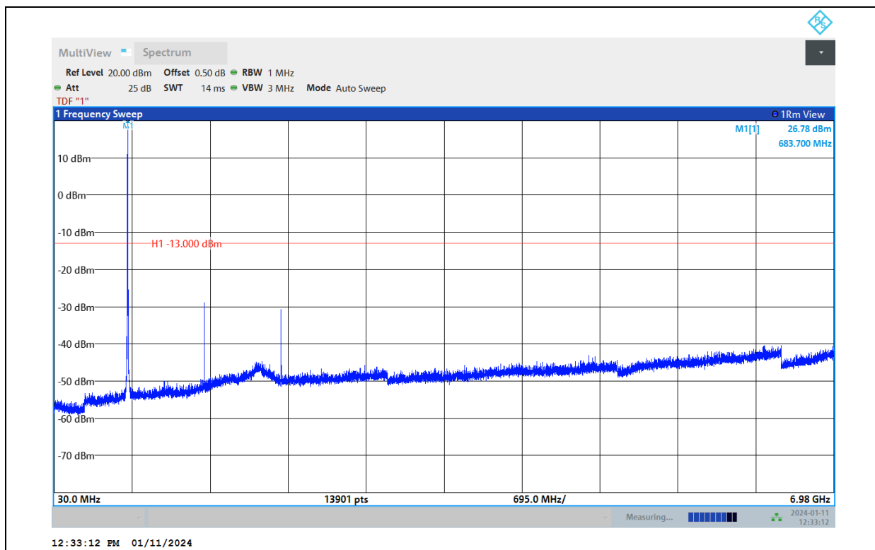
Band71-20MHz-QPSK-133222-1RB#0-Range:30~6980MHz
