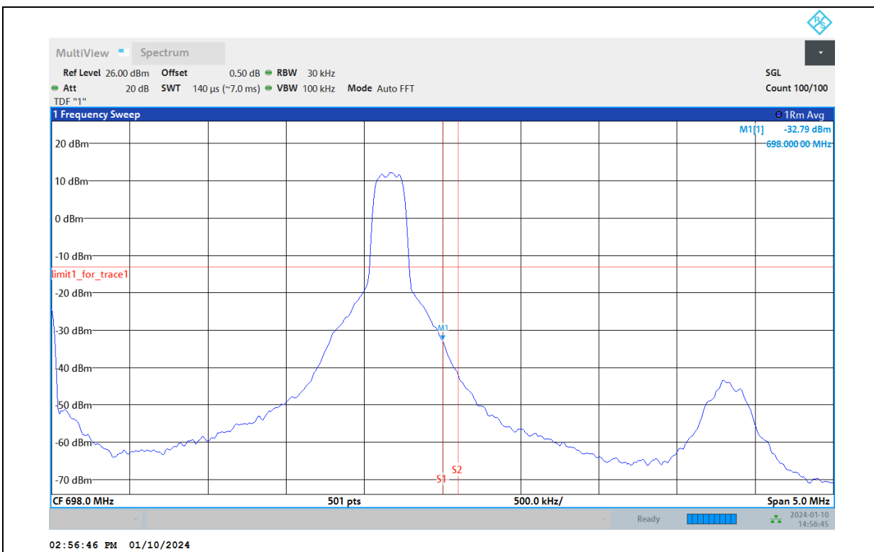
Band71-5MHz-16QAM-133447-25RB#0
