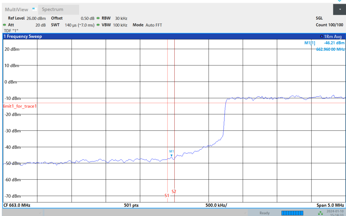
Band71-15MHz-16QAM-133397-1RB#74
