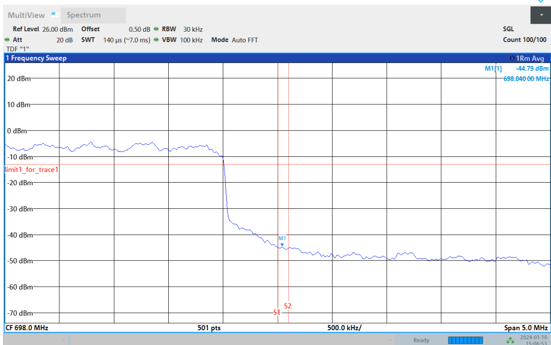
Band71-10MHz-16QAM-133172-1RB#0
