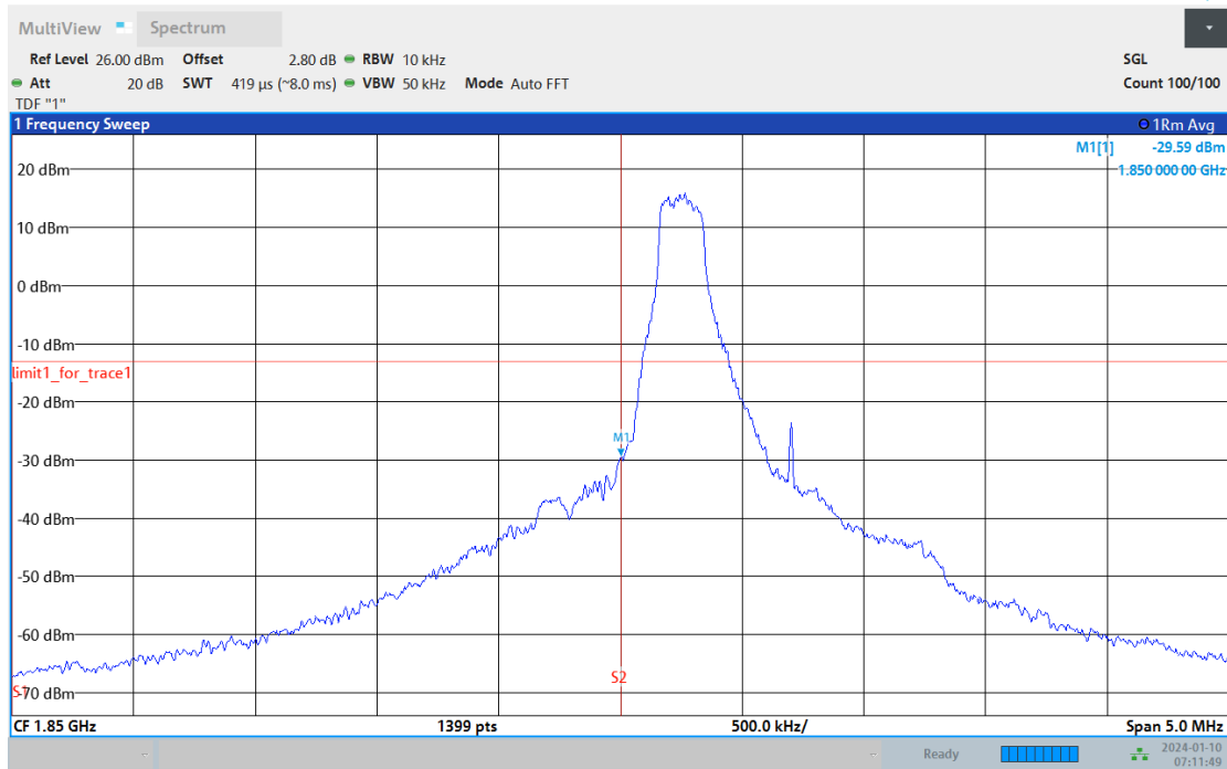
Band2-1.4MHz-QPSK-18607-6RB#0
