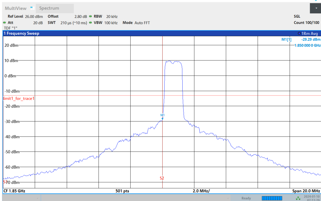
Band2-1.4MHz-QPSK-19193-1RB#5
