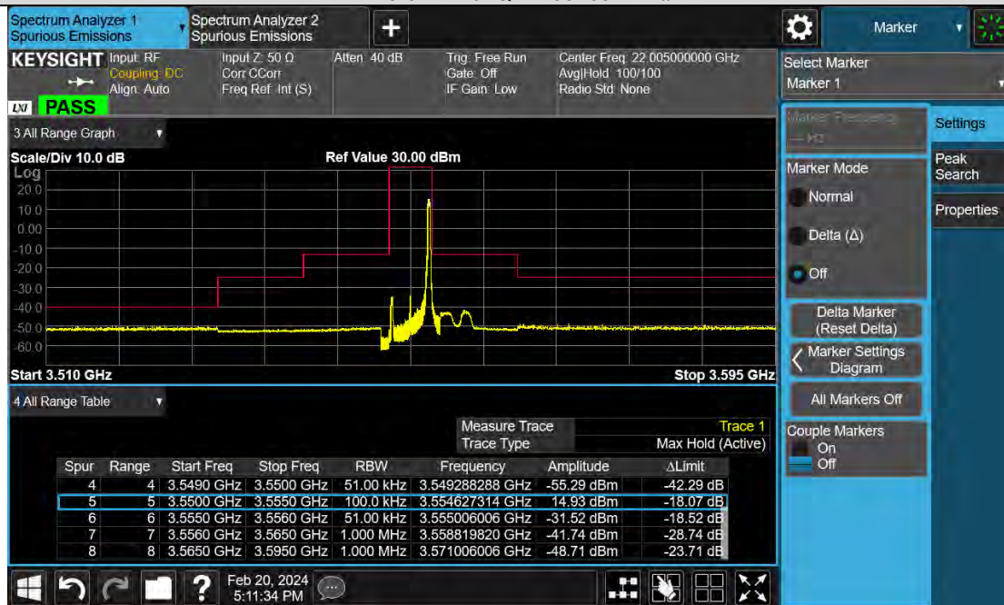
Band48-5MHz-64QAM-55265-25RB#0
