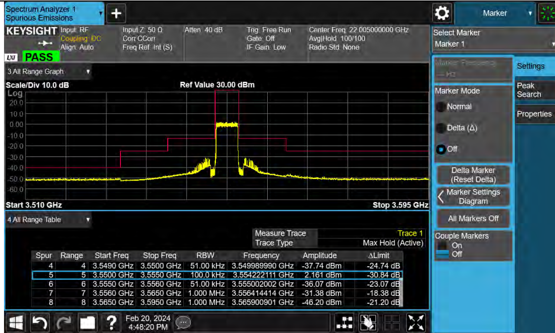
Band48-5MHz-64QAM-55990-1RB#0
