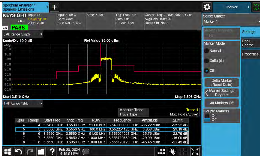
Band48-5MHz-16QAM-55990-1RB#0
