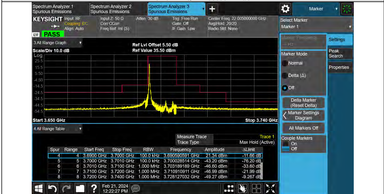
Band48-10MHz-QPSK-56690-1RB#49
