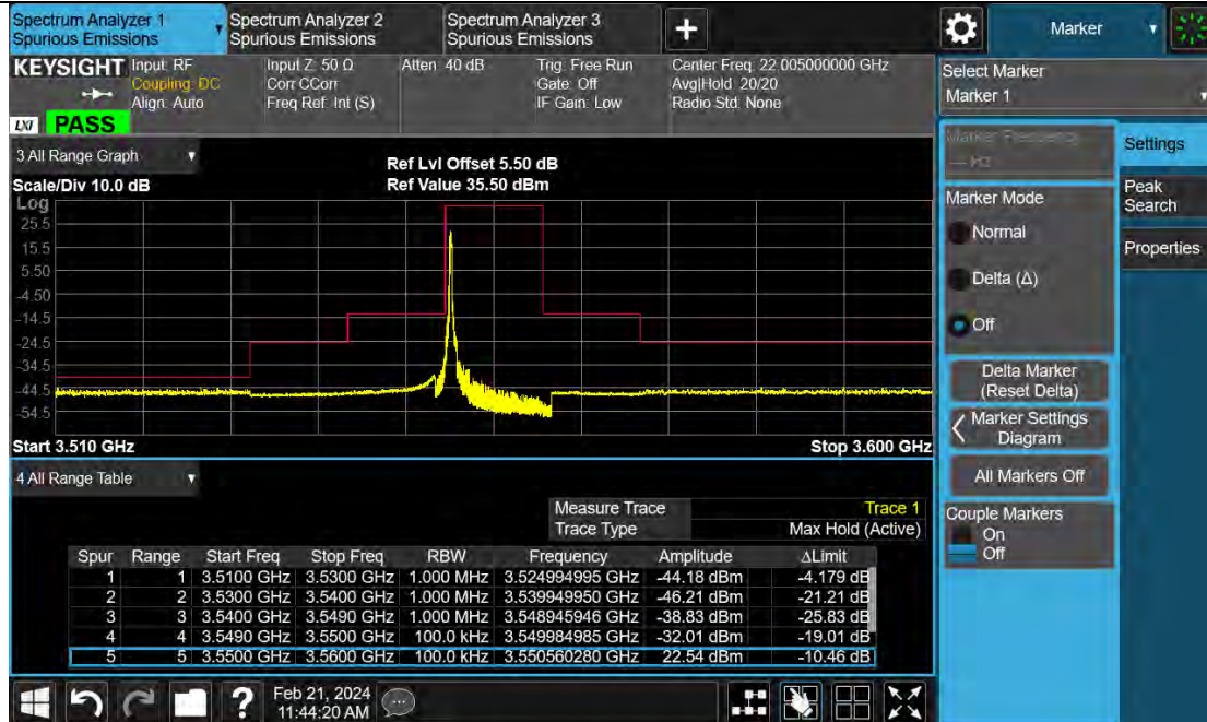
Band48-10MHz-16QAM-55290-1RB#49
