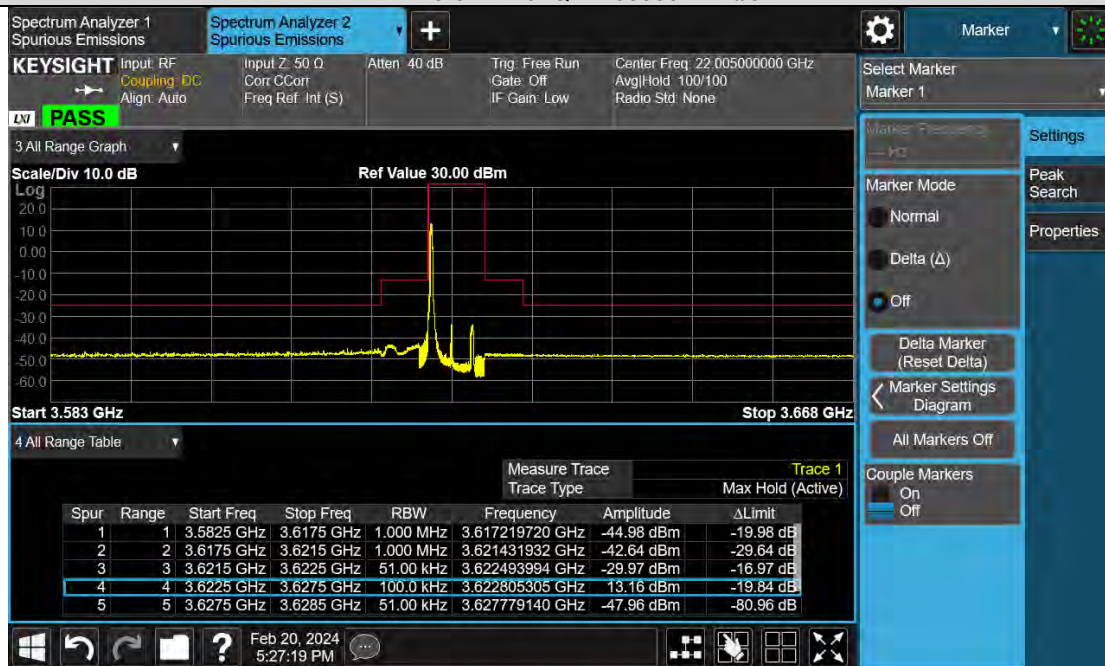
Band48-5MHz-64QAM-55990-1RB#24
