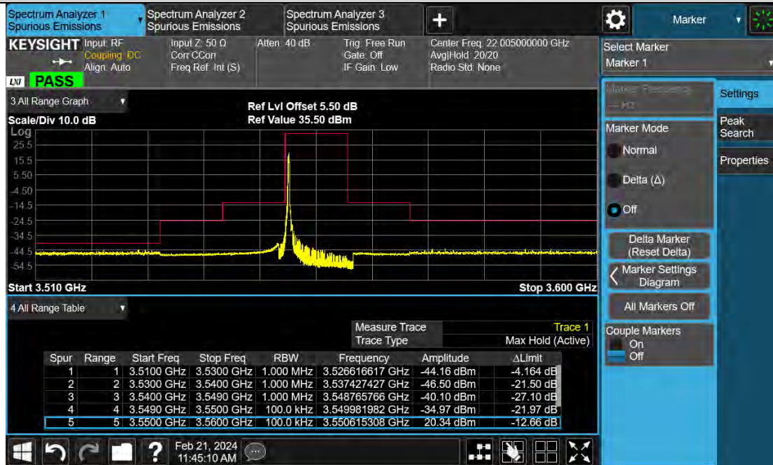
Band48-10MHz-64QAM-55290-1RB#49
