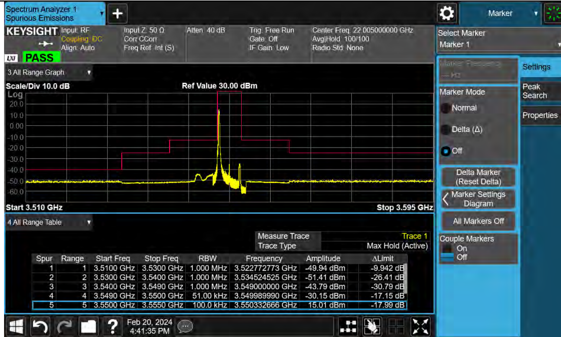
Band48-5MHz-64QAM-55265-1RB#24
