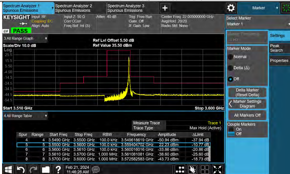
Band48-10MHz-16QAM-55290-50RB#0
