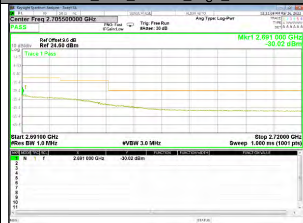
Band 41_10M_16QAM_High_Full-RB
