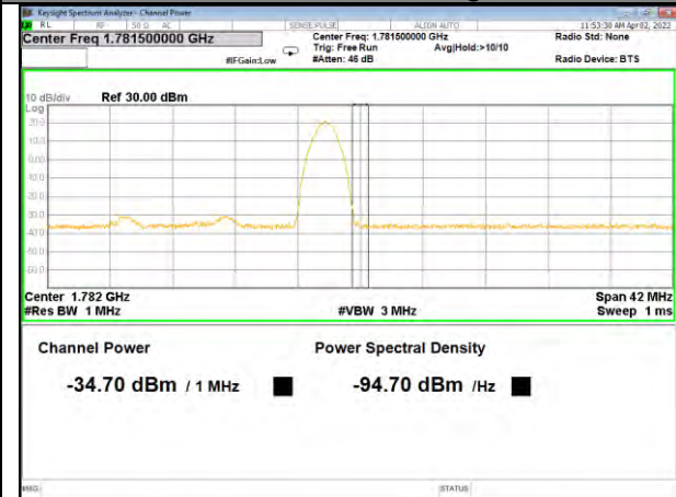
Band 66_15M_QPSK_High_Full-RB
