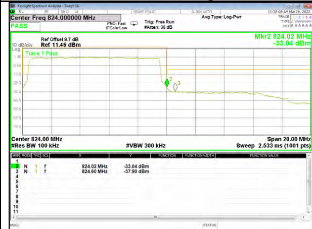
Band 26_10M_16QAM_Low_Full-RB
