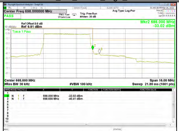
Band 71_5M_QPSK_High_Full-RB
