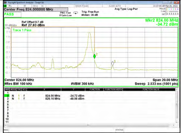
Band 26_10M_16QAM_Low_1-RB
