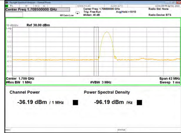
Band 66_20M_16QAM_Low_Full-RB
