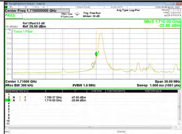
Band 66_15M_QPSK_Low_1-RB
