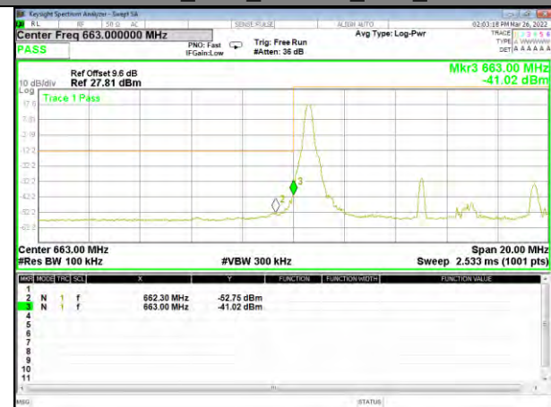
Band 71_10M_16QAM_Low_1-RB
