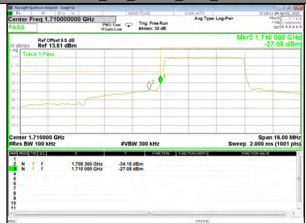
Band 66_5M_QPSK_Low_Full-RB
