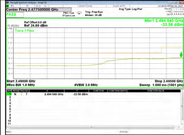
Band 41_20M_QPSK_High_1-RB
