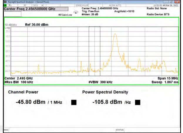
Band 41_5M_QPSK_Low_Full-RB
