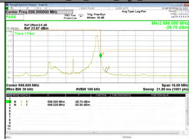
Band 71_5M_QPSK_High_1-RB
