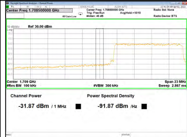
Band 66_10M_16QAM_Low_Full-RB
