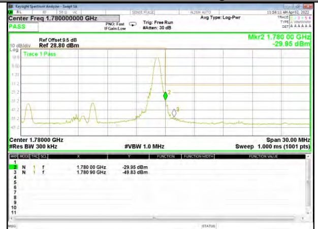
Band 66_15M_16QAM_High_1-RB
