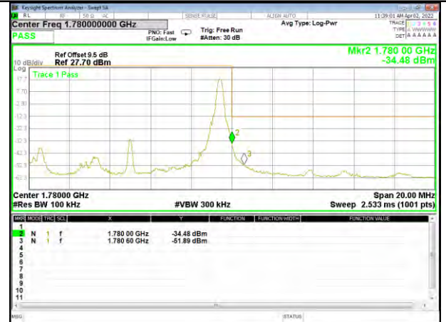
Band 66_10M_QPSK_High_1-RB
