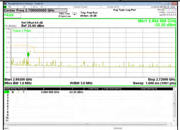
Band 41_5M_QPSK_High_1-RB
