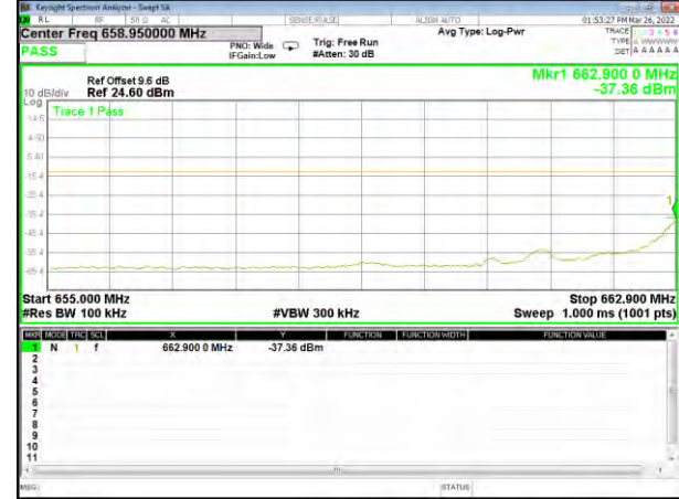
Band 71_5M_16QAM_Low_Full-RB
