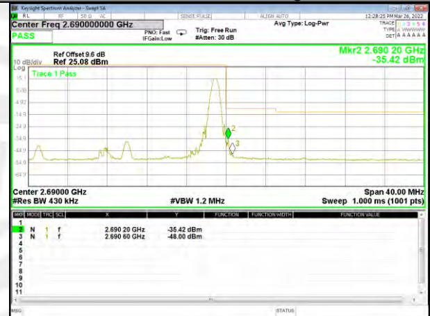
Band 41_20M_QPSK_High_Full-RB
