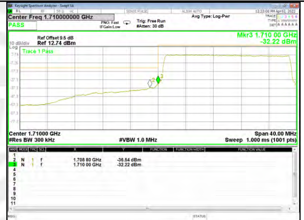
Band 66_20M_16QAM_Low_Full-RB
