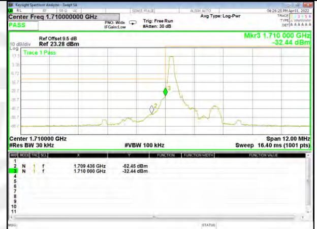
Band 66_1.4M_16QAM_Low_Full-RB
