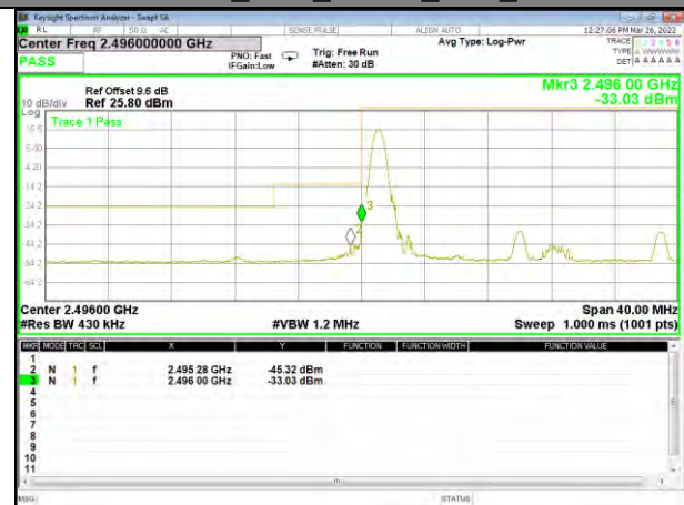
Band 41_20M_QPSK_Low_1-RB
