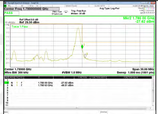
Band 66_15M_QPSK_High_Full-RB
