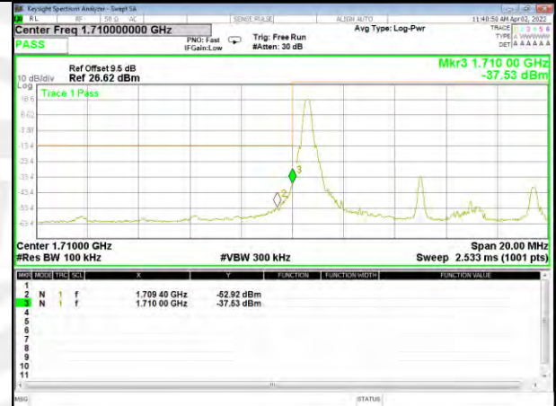
Band 66_10M_16QAM_Low_Full-RB
