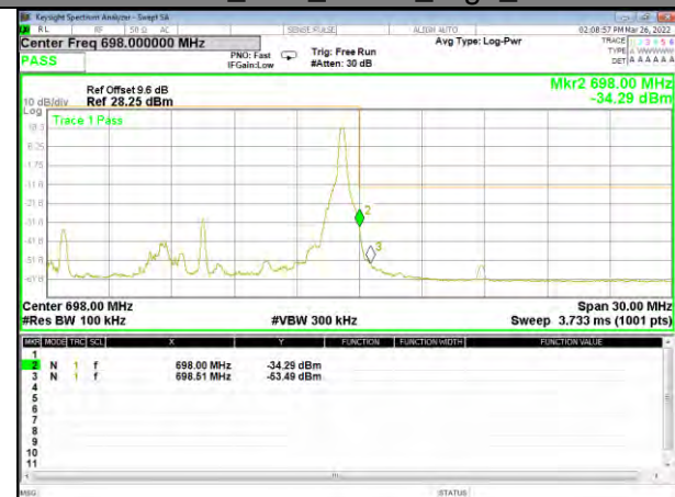
Band 71_15M_QPSK_High_1-RB
