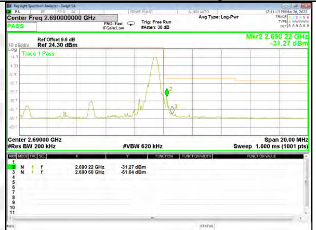
Band 41_10M_16QAM_High_Full-RB
