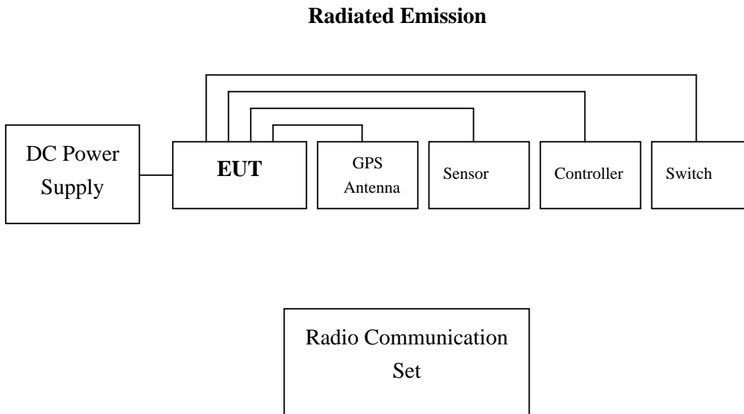
Fig. 2-1 Configuration of Tested System (Fixed Channel)
