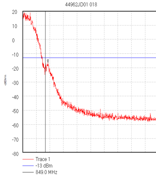
Top Channel
