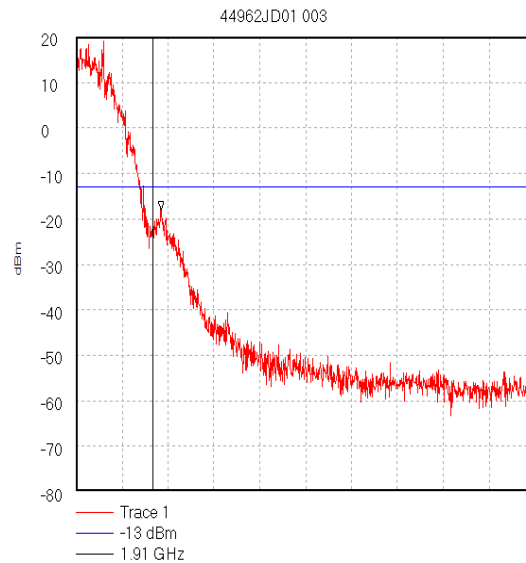
Top Channel
