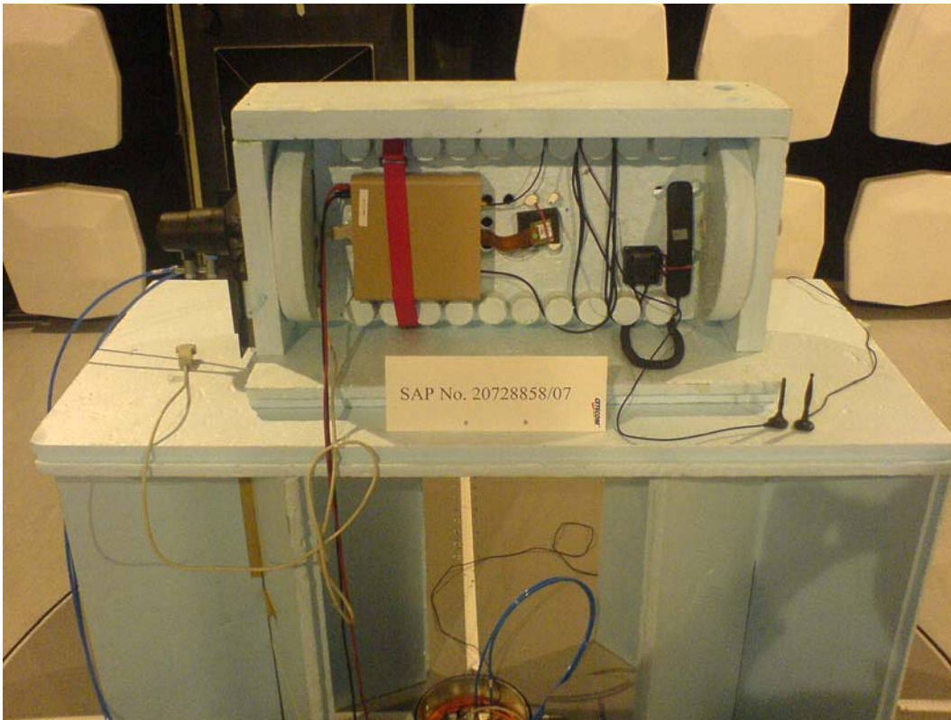
Photograph 1: Measurements in the anechoic chamber, test set-up (front view of test set-up)
