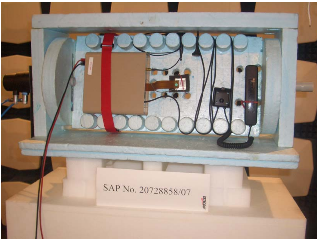
Photograph 2: Measurements in the anechoic chamber, test set-up
