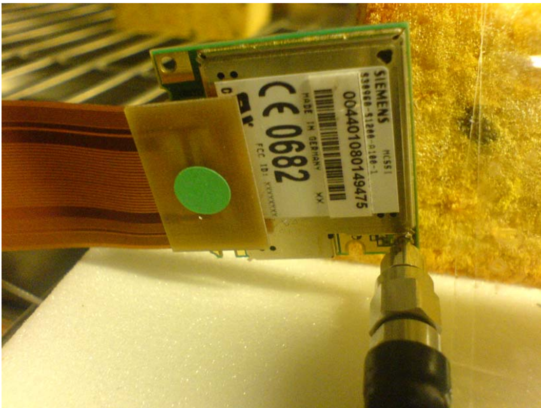
Photograph 4: Measurements of conducted power and spurious emissions on module's RF-port
