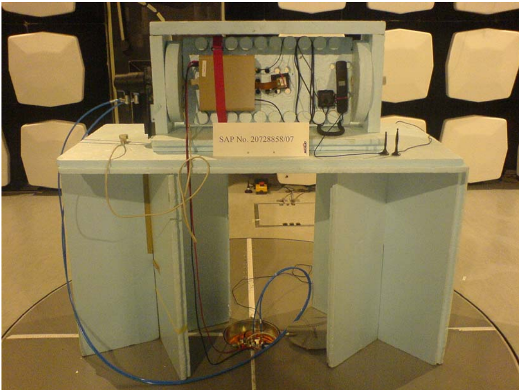
Photograph 2: Measurements in the anechoic chamber, test set-up (front view of test set-up)
