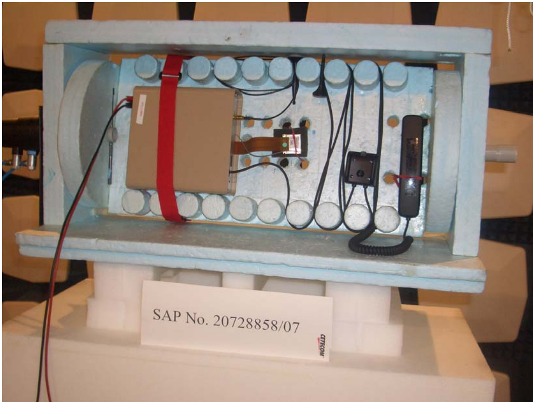
Photograph 1: Measurements in the anechoic chamber, EUT set-up
