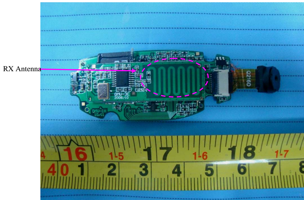
EUT – Main Board Bottom Shielding off View
