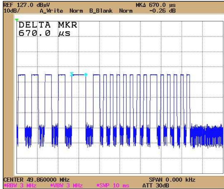
Duty Cycle 3
