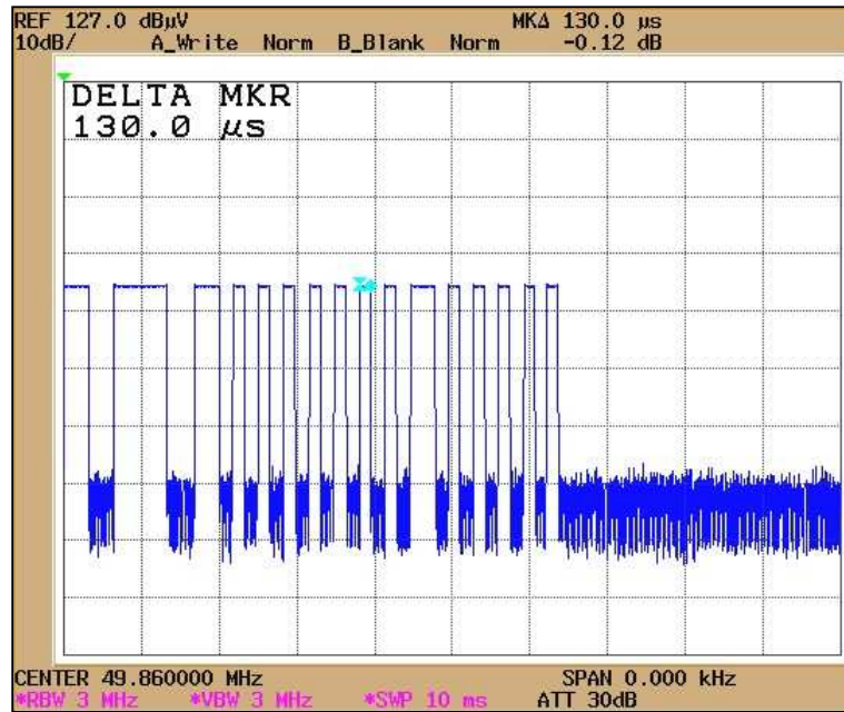
Duty Cycle 5
