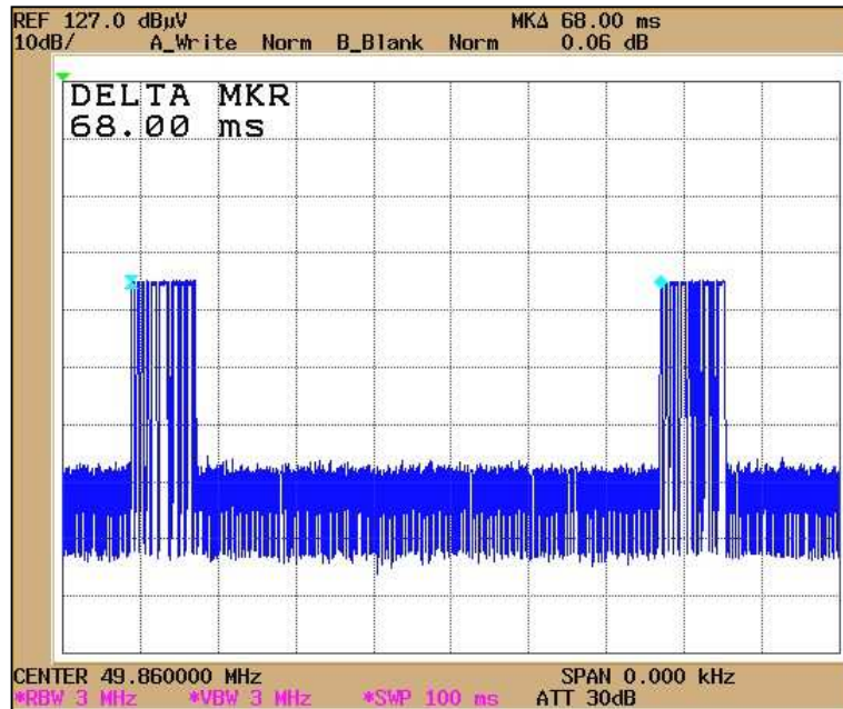
Duty Cycle 1
