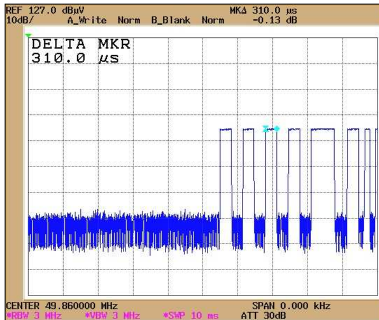
Duty Cycle 4
