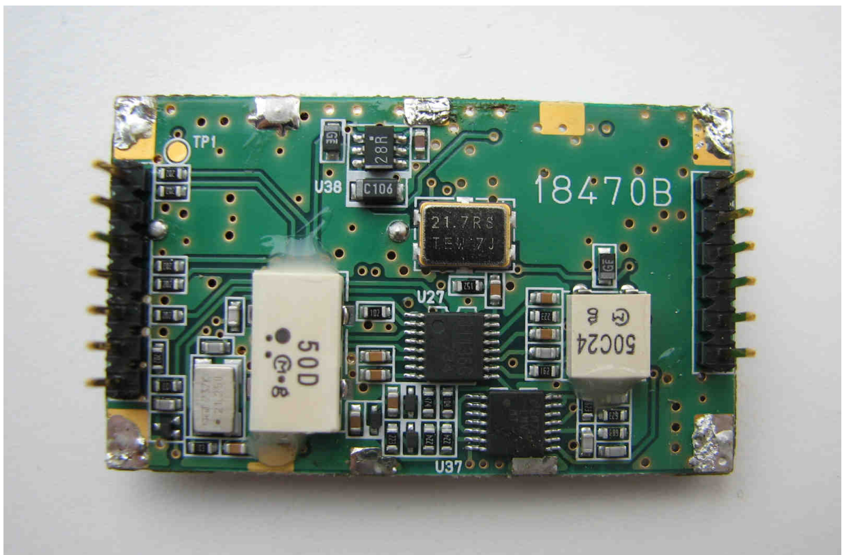
RF Module without Shielding - Bottom
