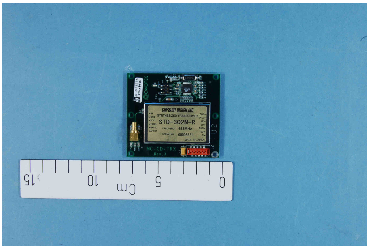
MC-CD-TRX-458 close-up photo, top view
