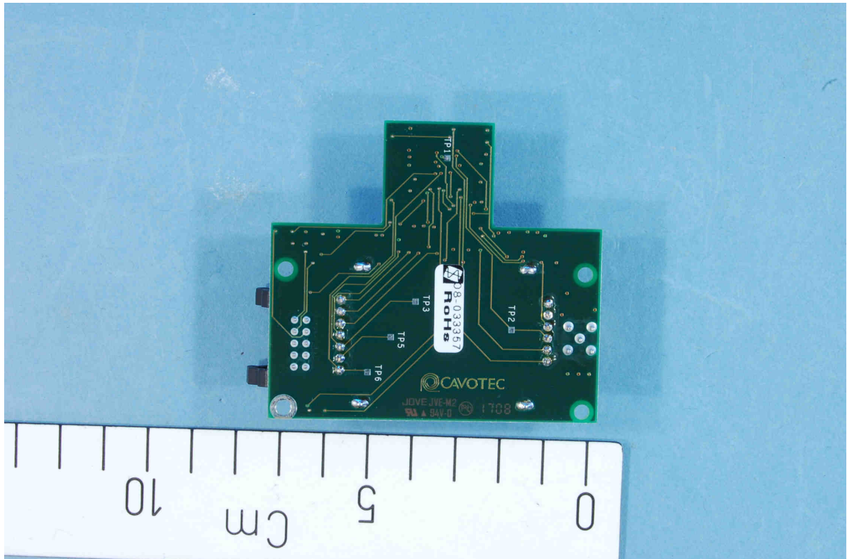
MC-CD-PLL-458 close-up photo, rear view
