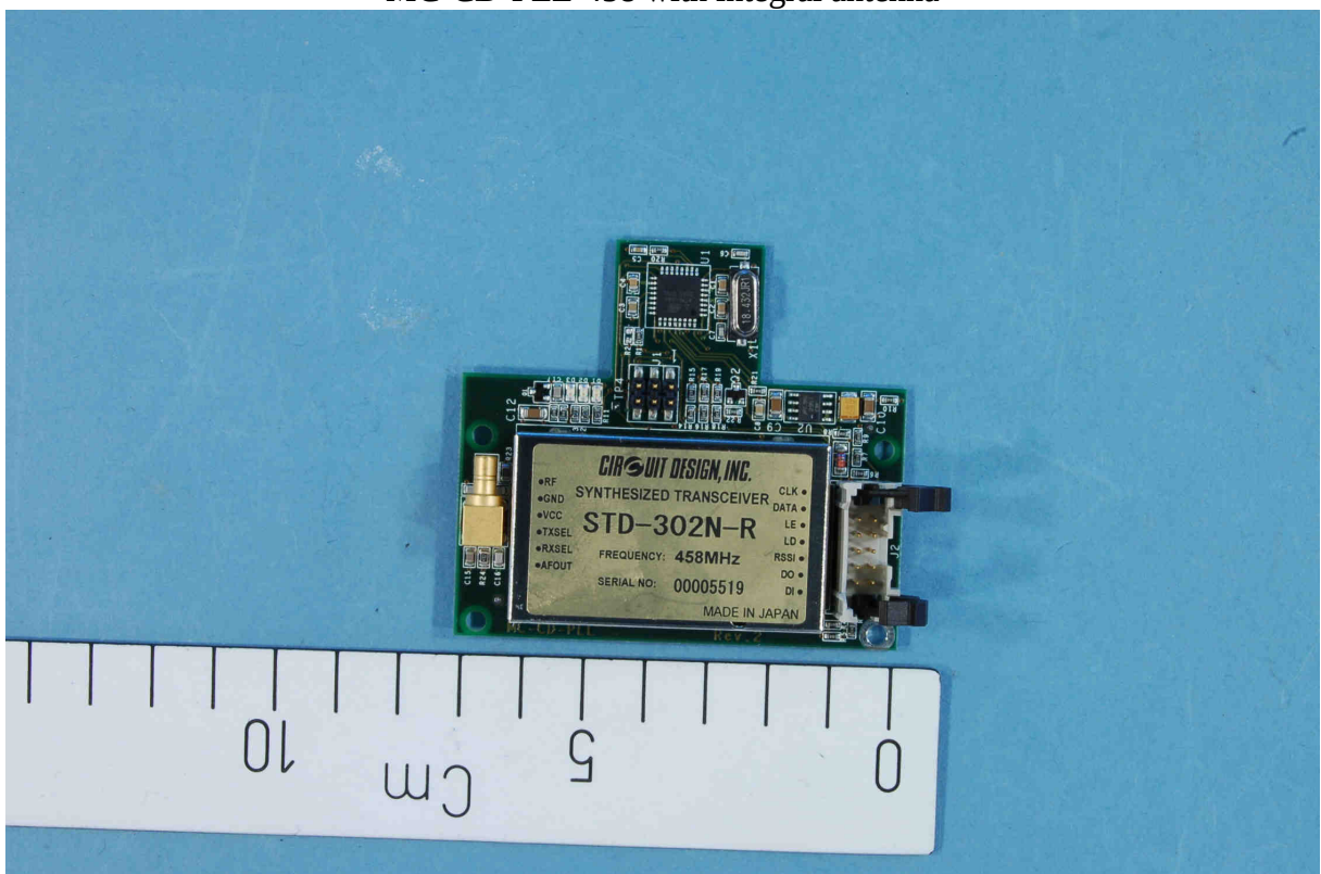
MC-CD-PLL-458 close-up photo, top view
