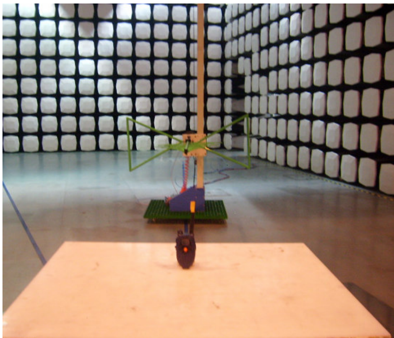
Emissions from 30MHz to 1000MHz:
