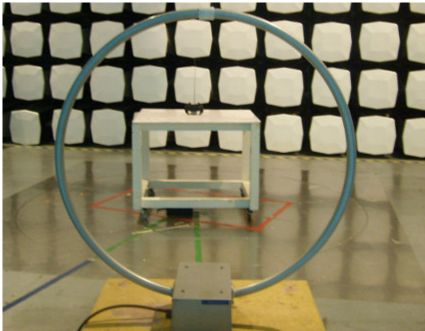
Emissions below 30MHz:
