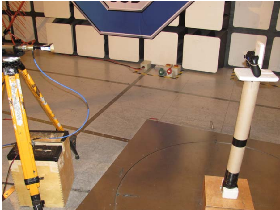
Radiated Emissions 18-25GHz
