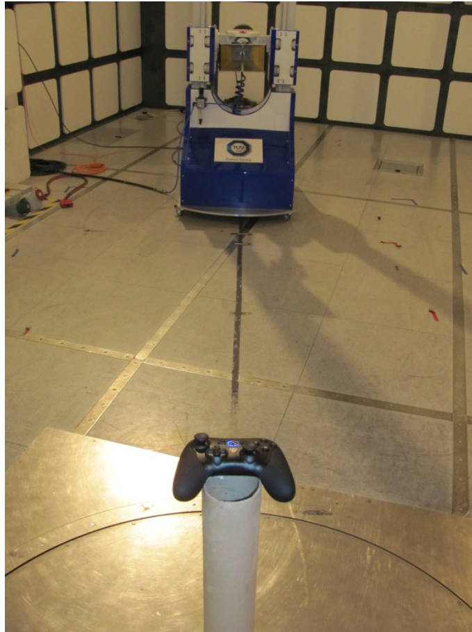
Radiated Emissions 1-18GHz
