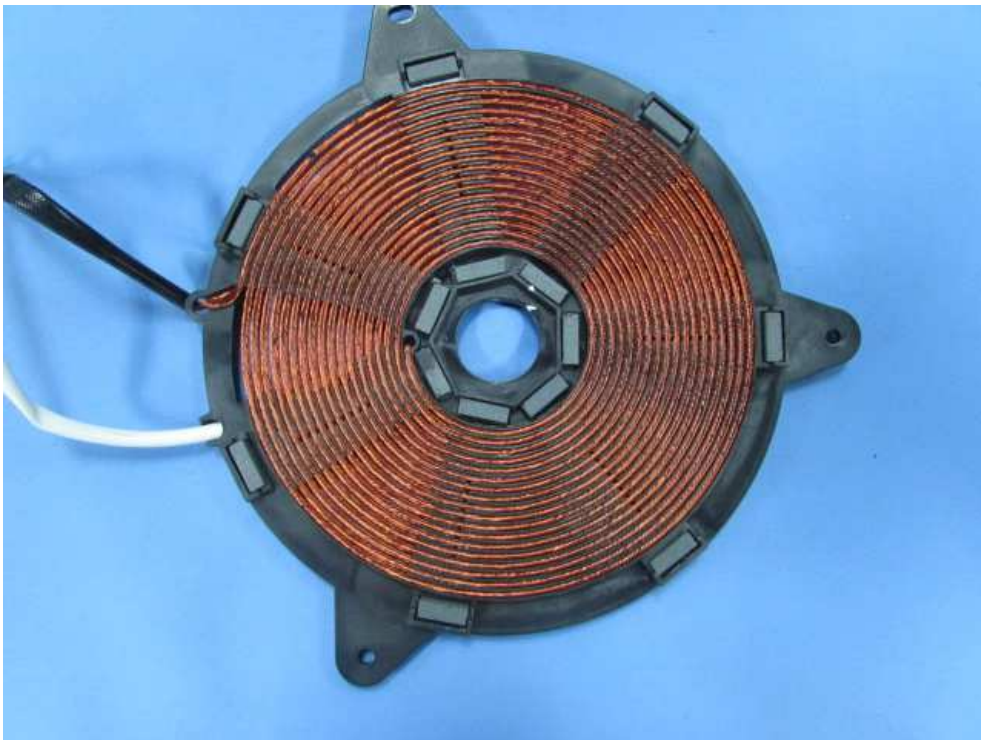
Coil view
