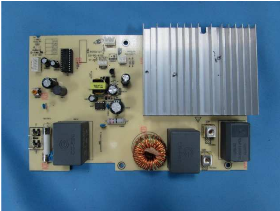
Power PCB:
