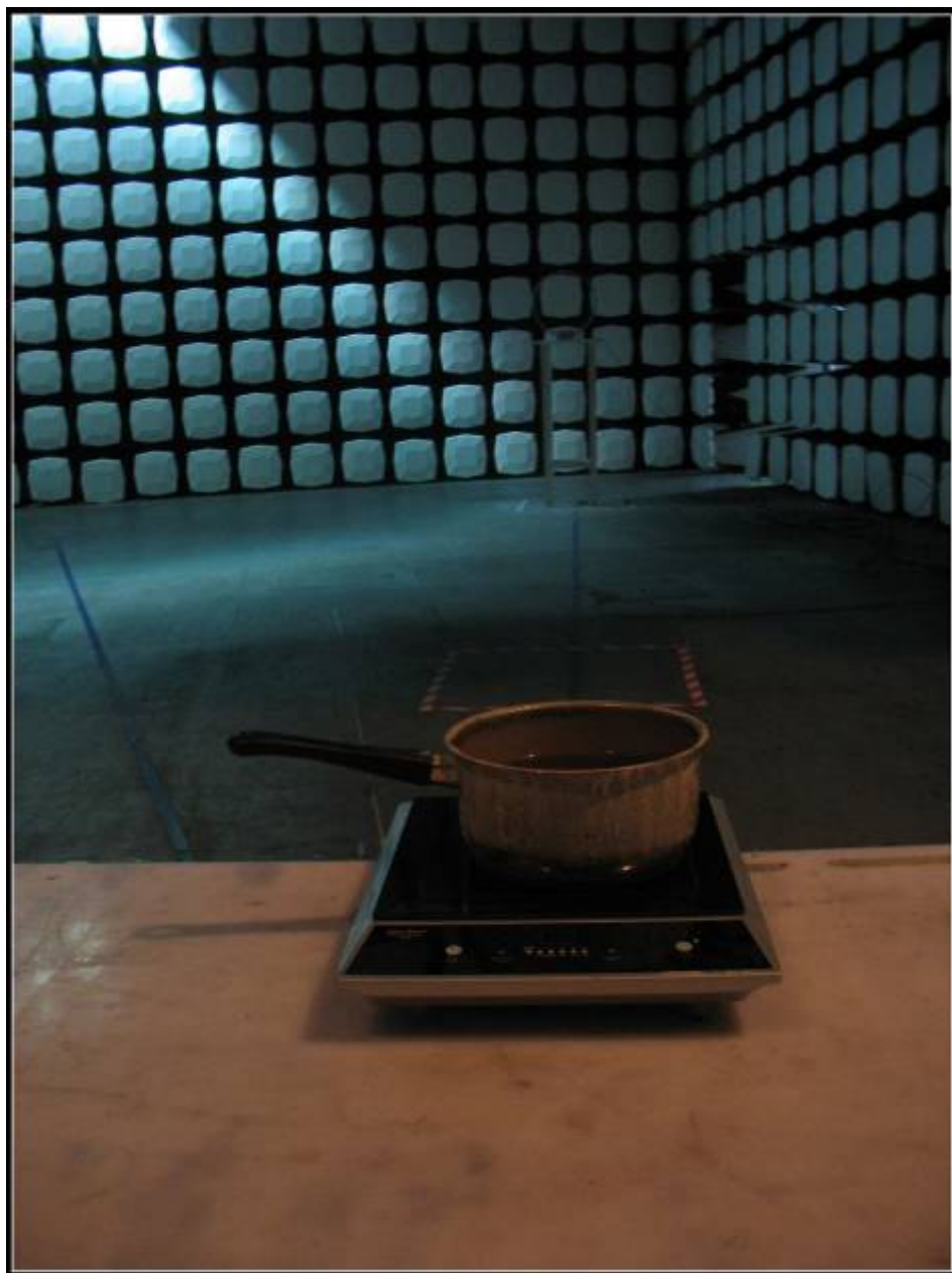
Model: MC-JSH13A(B)-1
