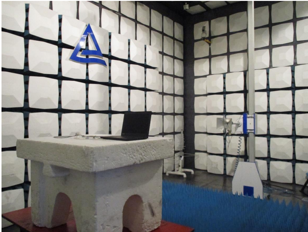
Photograph 3: Set-up for Radiated Spurious Emission, 1GHz - 18GHz
