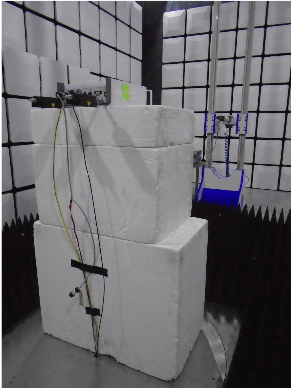
Radiated Emissions 18GHz-20GHz
