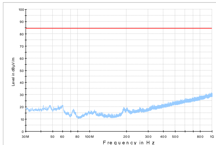
RSE_Erison_30M-1G_FCC
