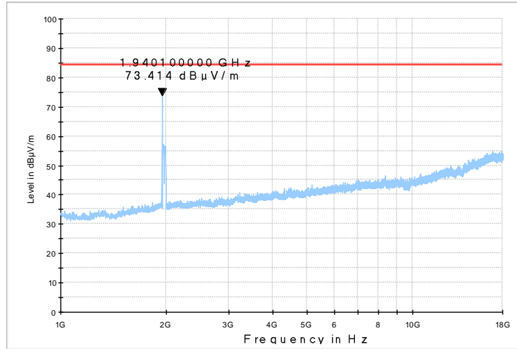
RSE_Erison_1-18G_FCC
