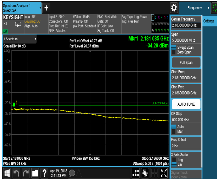
Port D, Channel Position B, 10.0MHz
