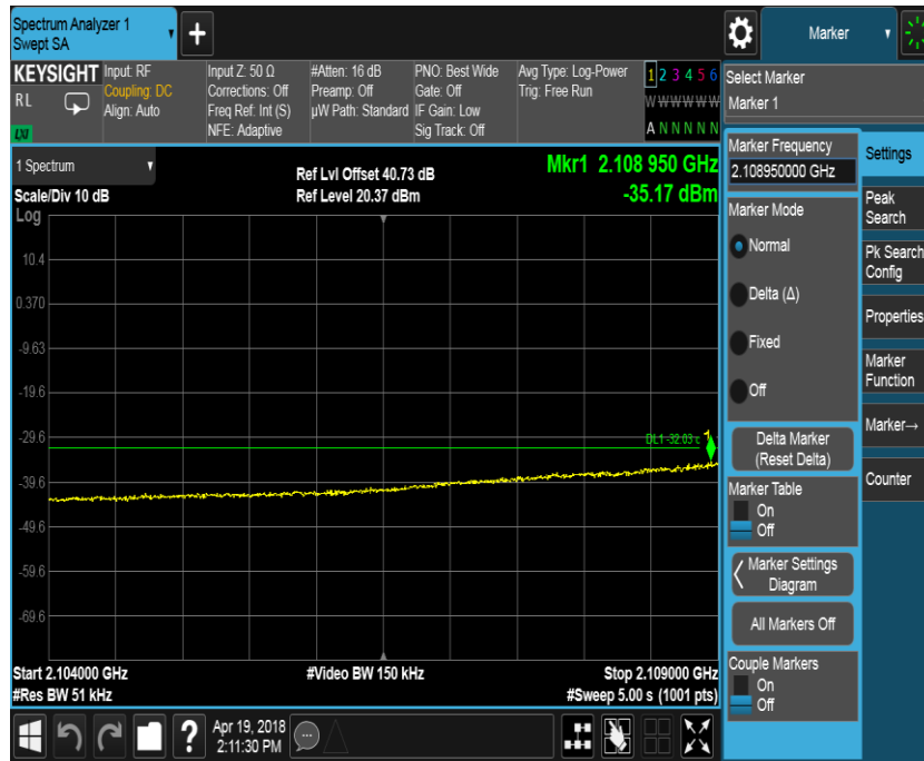
Port D, Channel Position T, 64QAM
