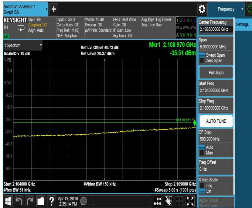
Port D, Channel Position T, 5.0MHz
