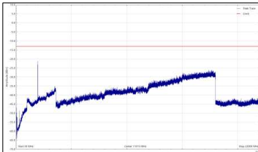
NR&NB-IoT - B2, 1960MHz, 30 MHz to 22 GHz, Vertical (Peak)
