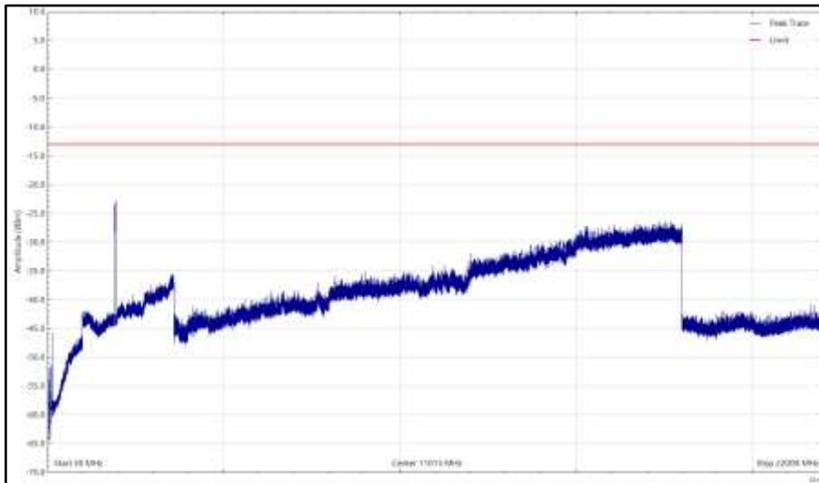
Bot - NR&NB-IoT - B25, 1940MHz, 30 MHz to 22 GHz, Horizontal (Peak)
