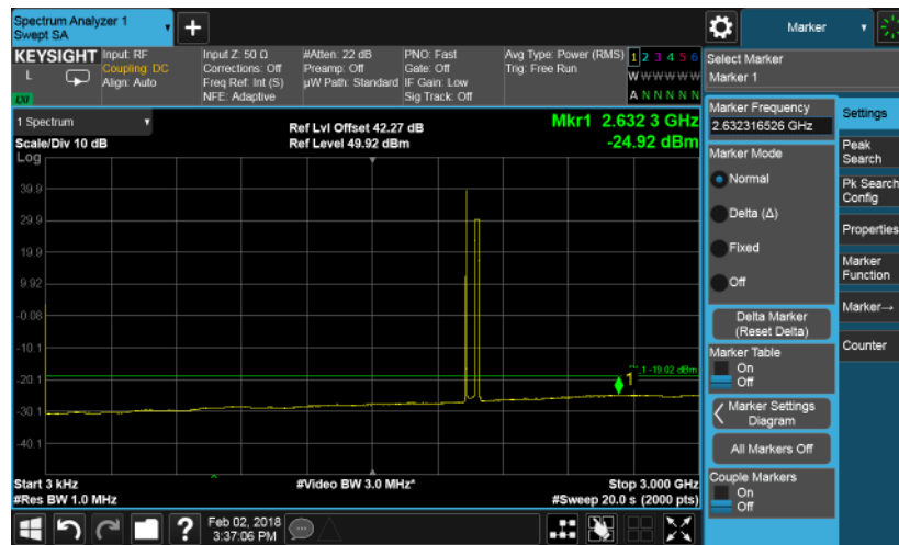
Port B, Channel Position M 20.0 MHz
