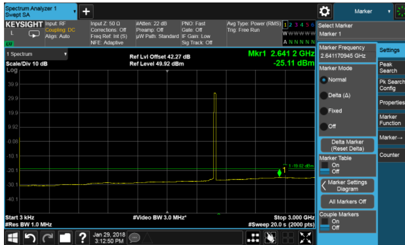
Port B, Channel Position T 20.0 MHz
