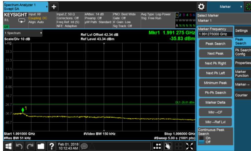
Configuration NB-IOT+GSM-MC-3-BE, (1NB, QPSK +1GSM, GMSK)
