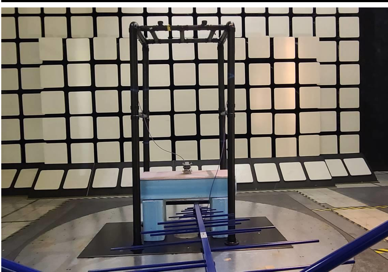
Figure 1: Radiated Test setup (30 to 1000MHz)
