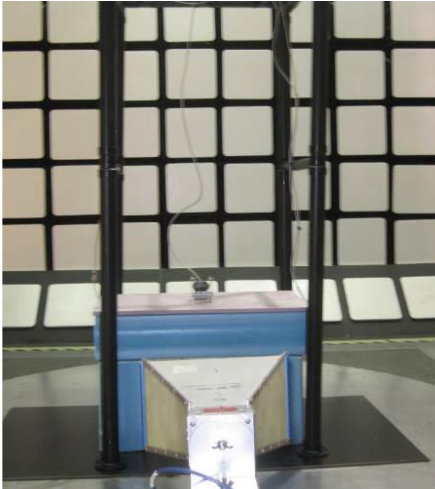
Figure 3 Test Antenna (1 to 10 GHz)
