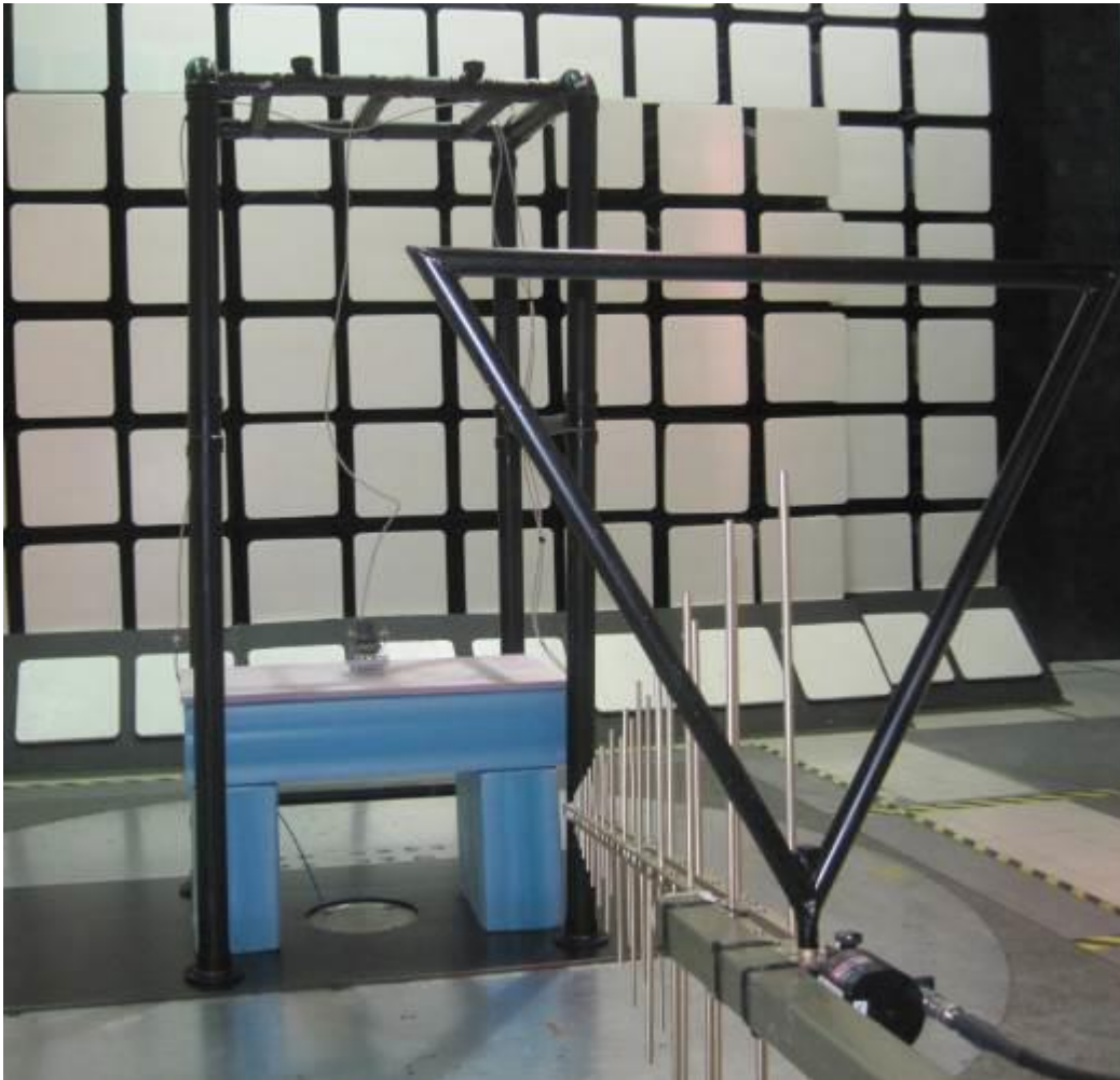
Figure 4 Test Antenna (30 MHz to 1 GHz)
