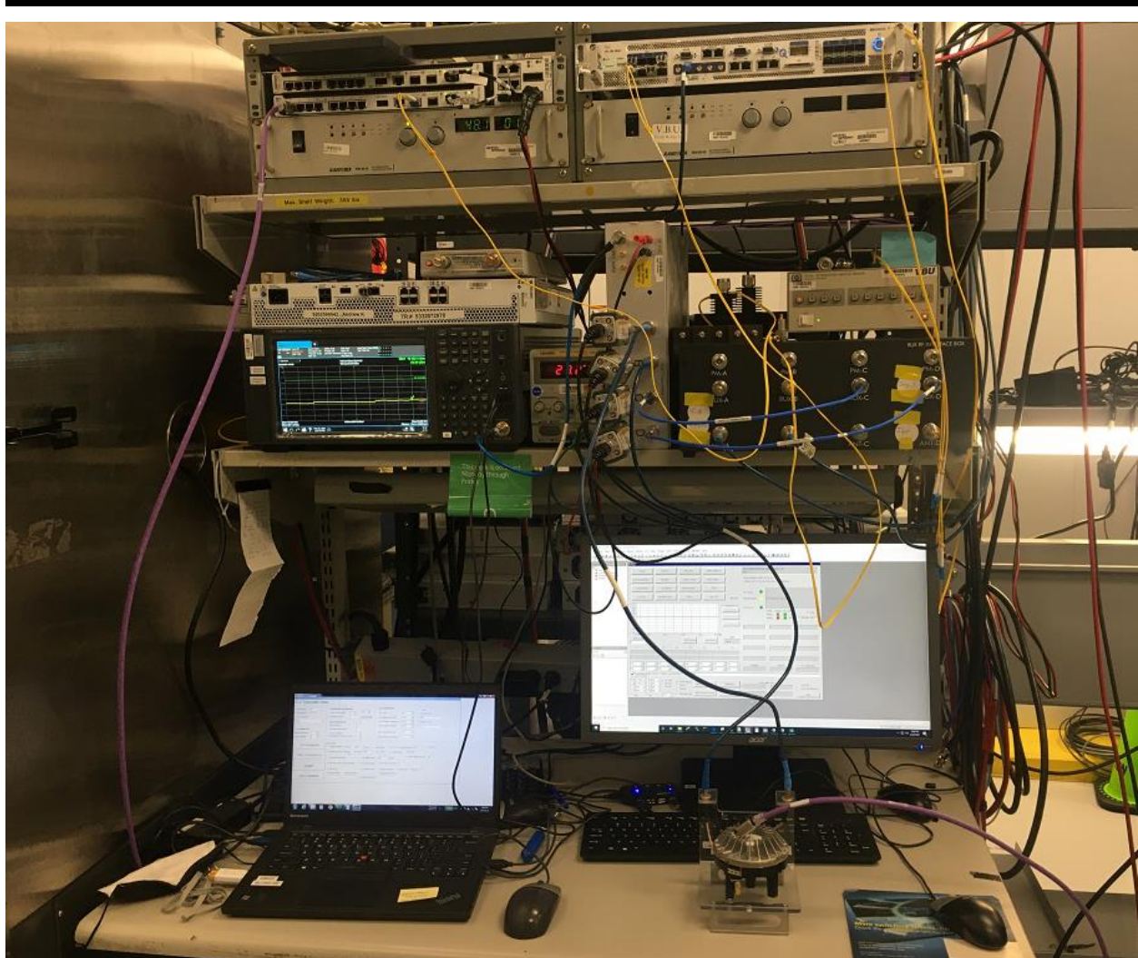
Figure 2: Conducted Test setup
