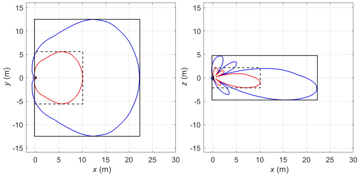
Figure 5 Compliance boundaries for general public (black solid line) and workers (black dashed line) exposure for the markets where the FCC exposure limits apply. The blue and red solid lines correspond to compliance distance results for general public and workers exposure, respectively, obtained using the spherical models. The antenna is shown from above (left) and from the side (right) with its backplane located at x = 0 m. Mode: B77D (NR). Total time-averaged power delivered to the antenna: 52.3 dBm.
