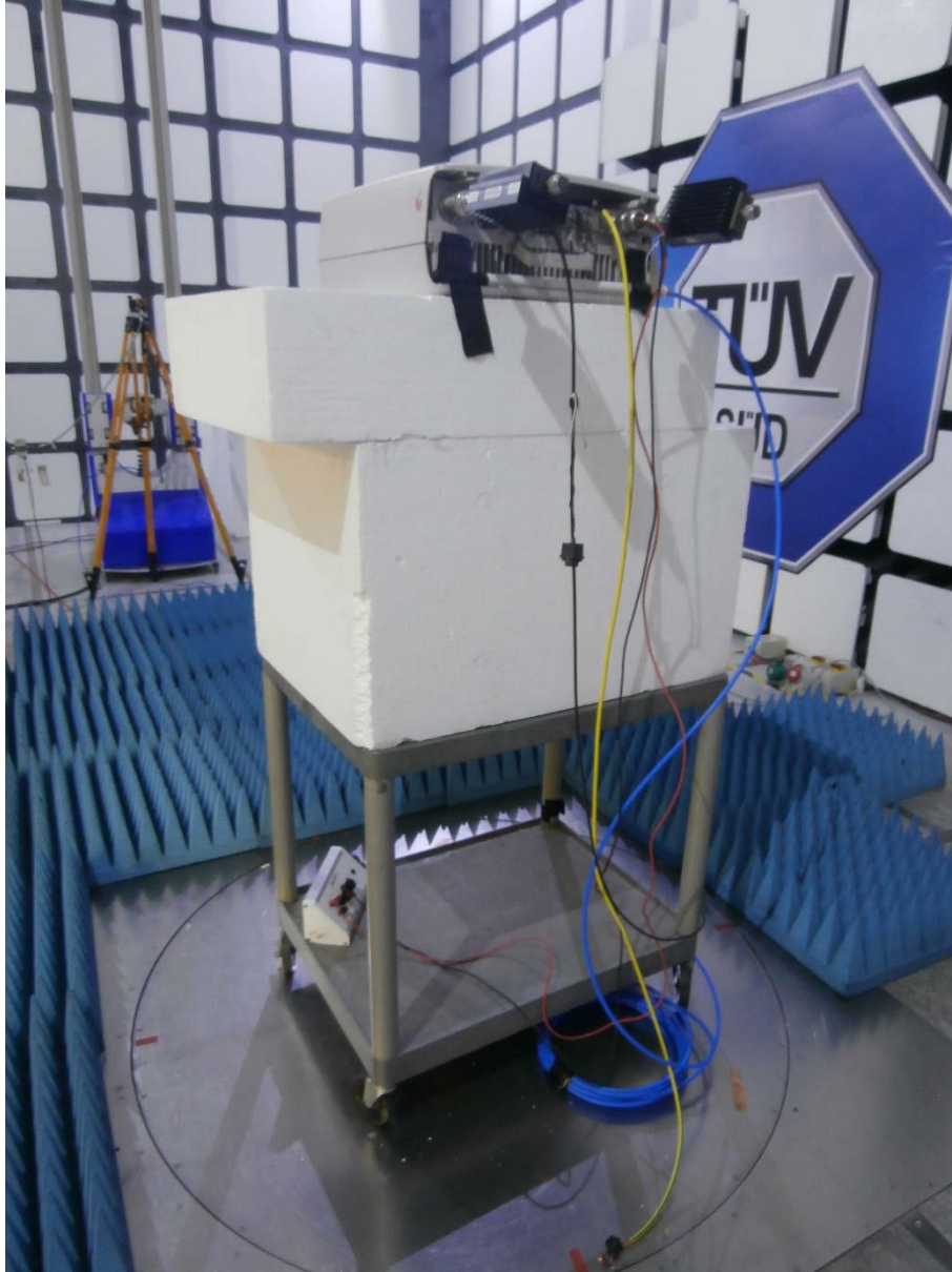
Radiated Emissions 18 GHz to 25 GHz
