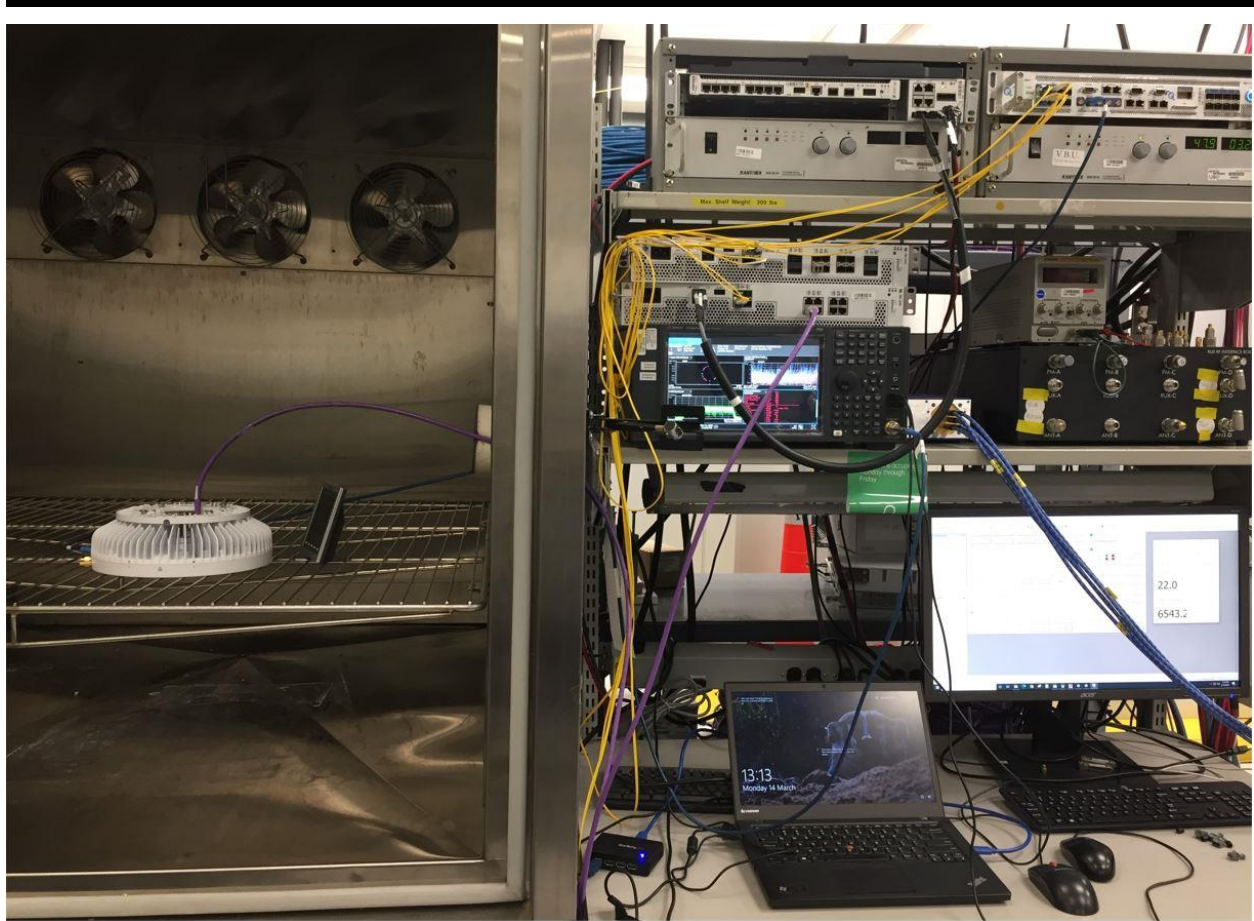
Figure 3: Frequency stability test setup
