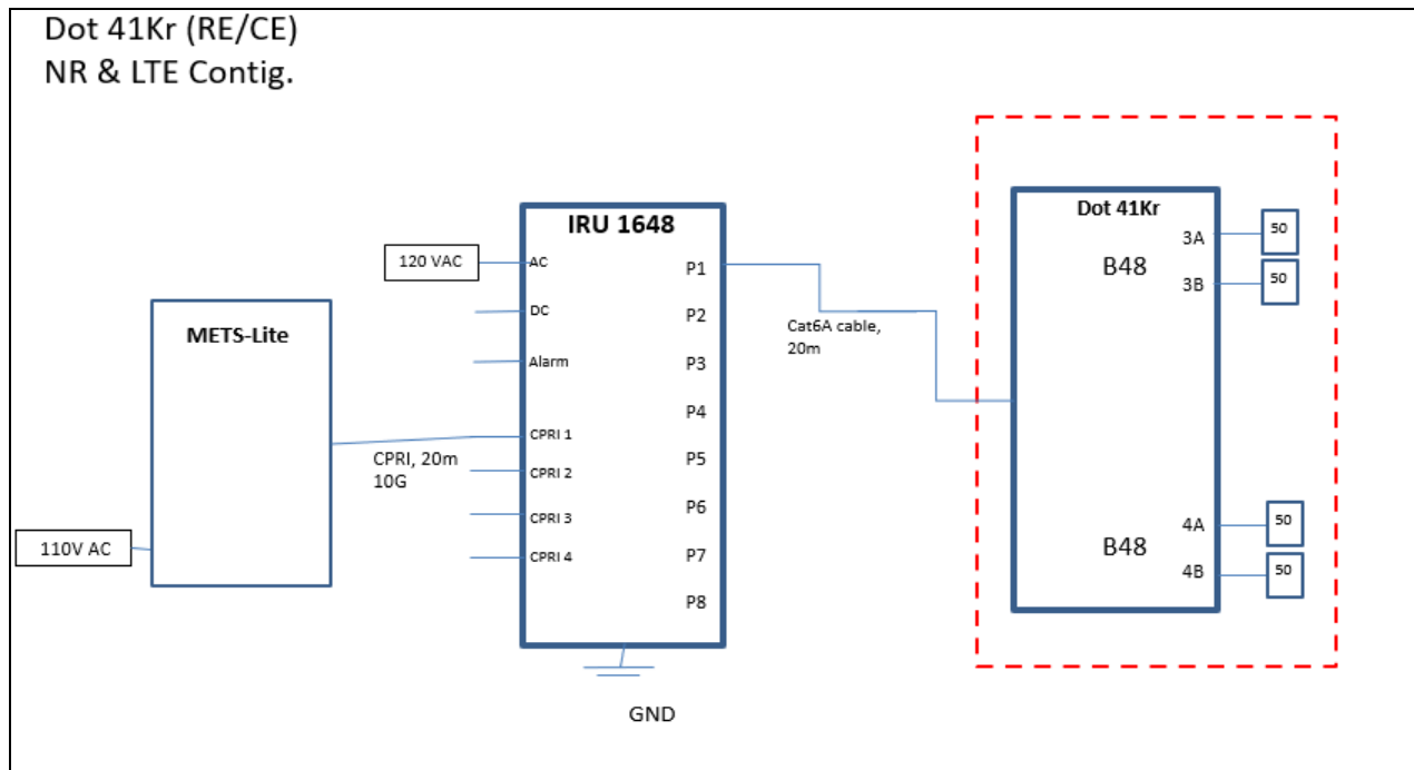
Figure 3: Test configuration 1 for Emission tests (contiguous mode)
