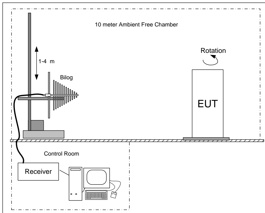
Figure 13: Setup of Radiated Emissions
