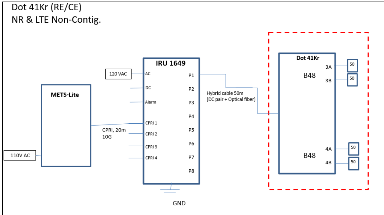
Figure 9: Test configuration 2 for Emission tests (non-contiguous mode)
