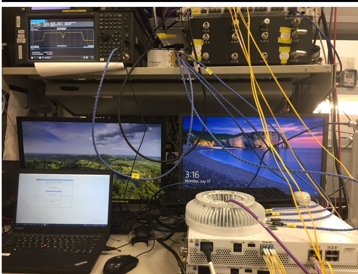
Figure 3: Conducted test setup (Contiguous with IRU 1648)
