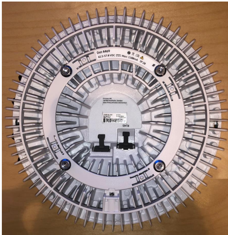
Figure 2: Dot 4469 B48 Bottom View
