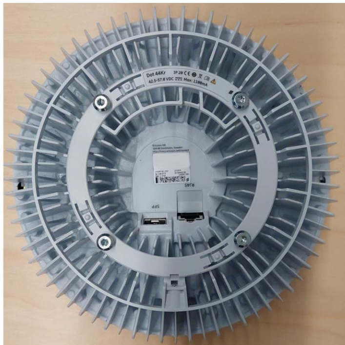
Figure 2: Dot 44Kr B77D Bottom View
