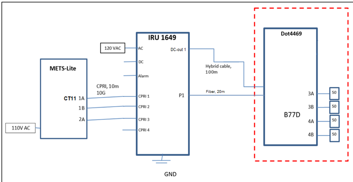
Figure 3: Test configuration for Emission tests (Config 1)
