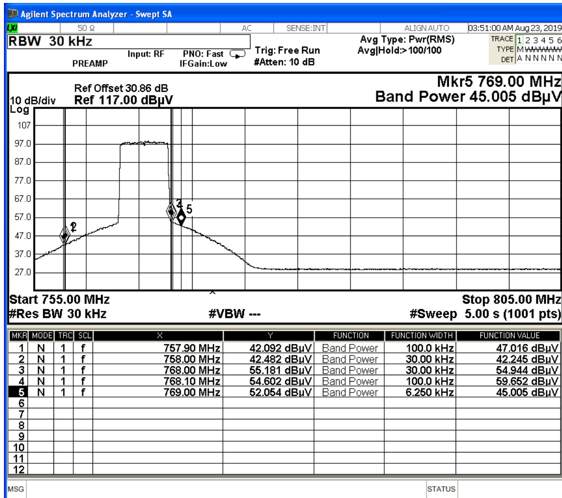
Figure 9: Plot of RE at 3 m – 755 to 805 MHz (5M LTE – Top channel, worst case vertical)
