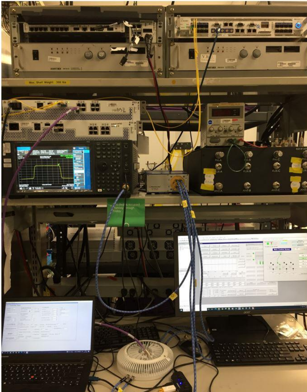
Figure 1: Conducted test setup
