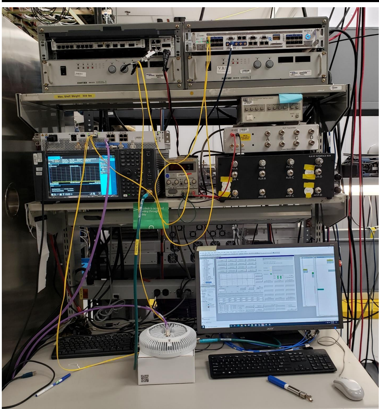
Figure 2: Conducted test setup
