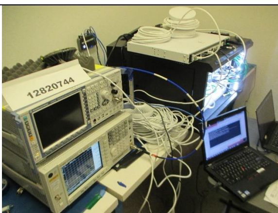
RF POWER TEST MEASUREMENT SETUP
