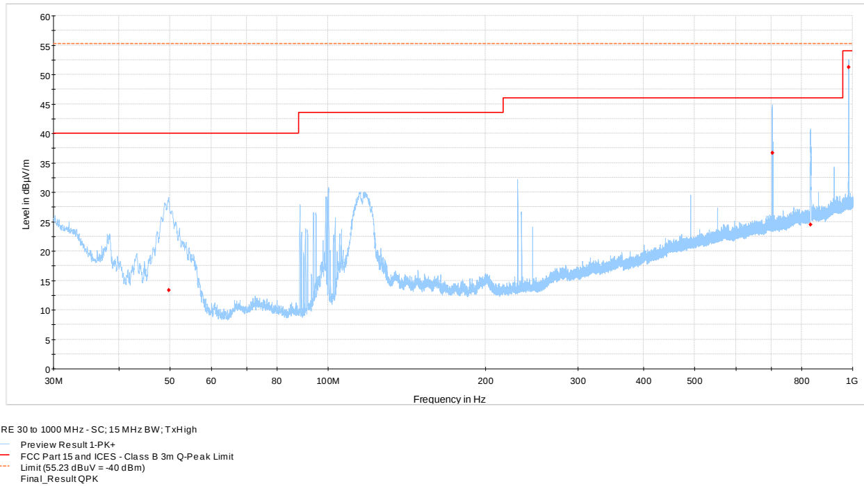
Figure 7.1-3: Radiated emissions spectral plot (30 to 1000 MHz) – Single carrier 15 MHz channel [top]
