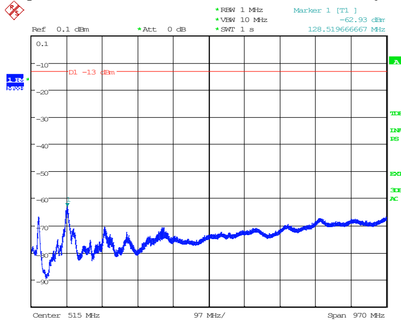
Diagram 2.1b: Pre scan 30 – 1000 MHz, BL 250 , EIRP Vertical polarization
