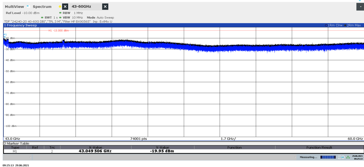
Diagram 2.13b: 43 – 60 GHz, QPSK, BL 250 , EIRP Vertical polarization
