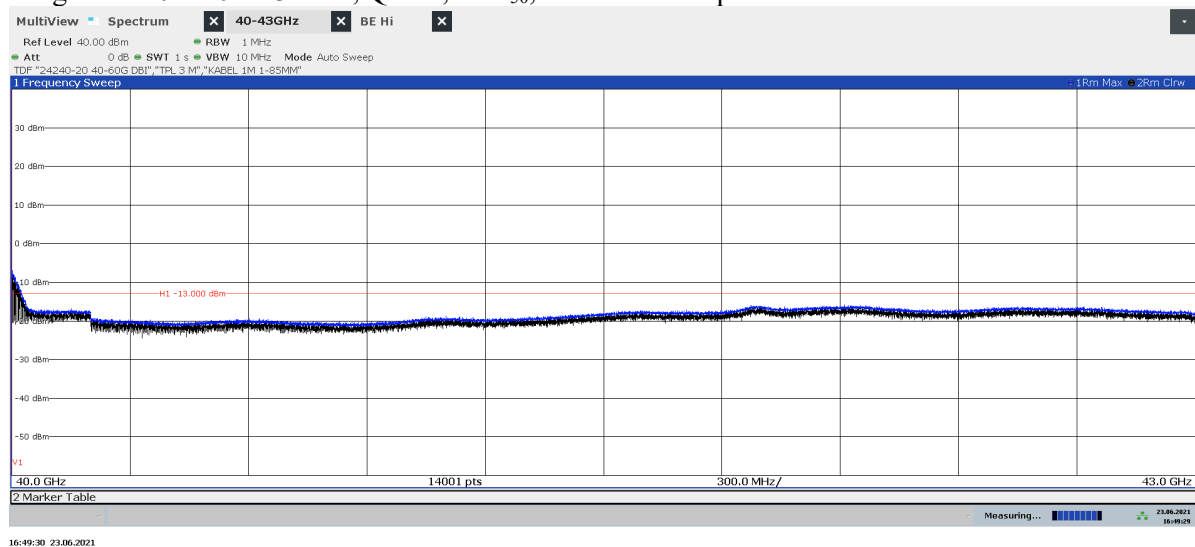
Diagram 2.10b: 40 – 43 GHz, QPSK, TH 250 , EIRP Vertical polarization
