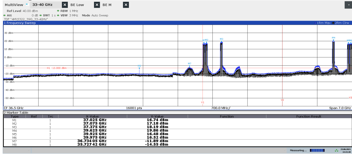
Diagram 2.7a: 33 – 40 GHz, QPSK, BTim6 50 , EIRP Horizontal polarization See diagram 2.7e for TRP result
