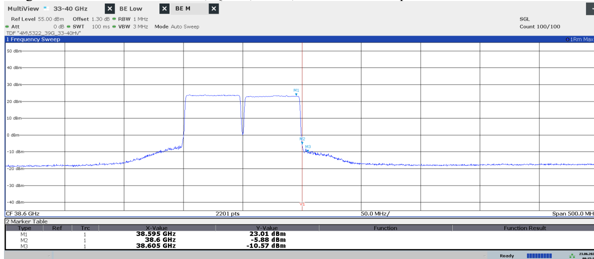
Diagram 2.8a: 38.35 – 38.85 GHz, QPSK, TL2 50 , EIRP Horizontal polarization
