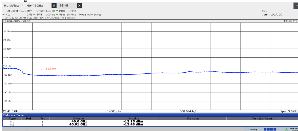
Diagram 2.11d: 40 – 43 GHz, QPSK, TH8 100 , EIRP Vertical polarization See diagram 2.11e for TRP result
