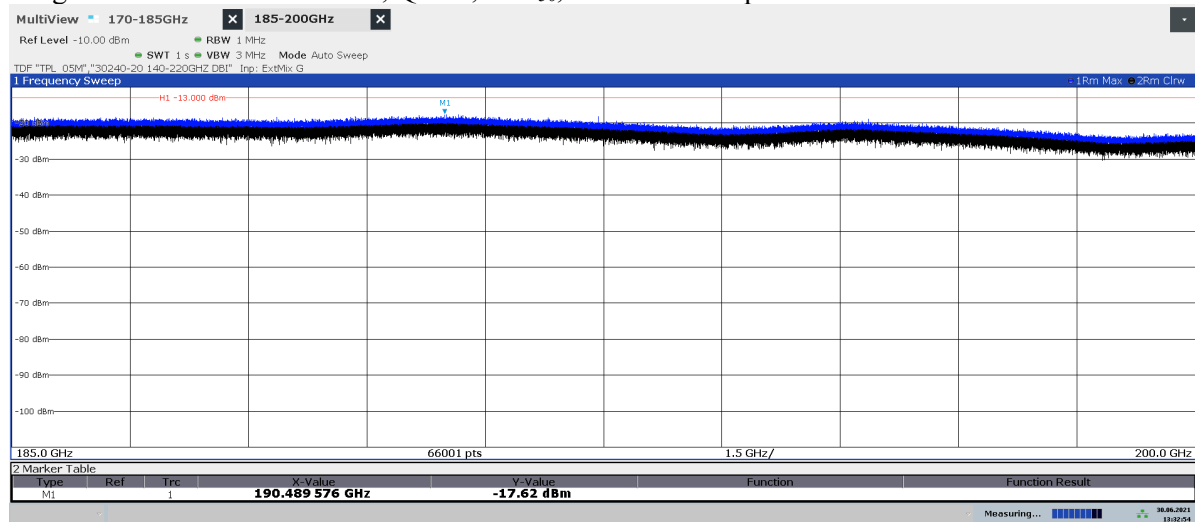
Diagram 2.21b: 185 – 200 GHz, QPSK, BL 250 , EIRP Vertical polarization
